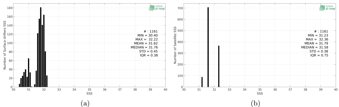
Figure 2: Histograms of SSS from Surface drifters (a) and SMAP-L3-JPL-V4.3-MONTHLY-60KM (b) considering all match-up pairs per bins of 0.1 over the Arctic Ocean Pi-MEP region and for the full satellite product period.
