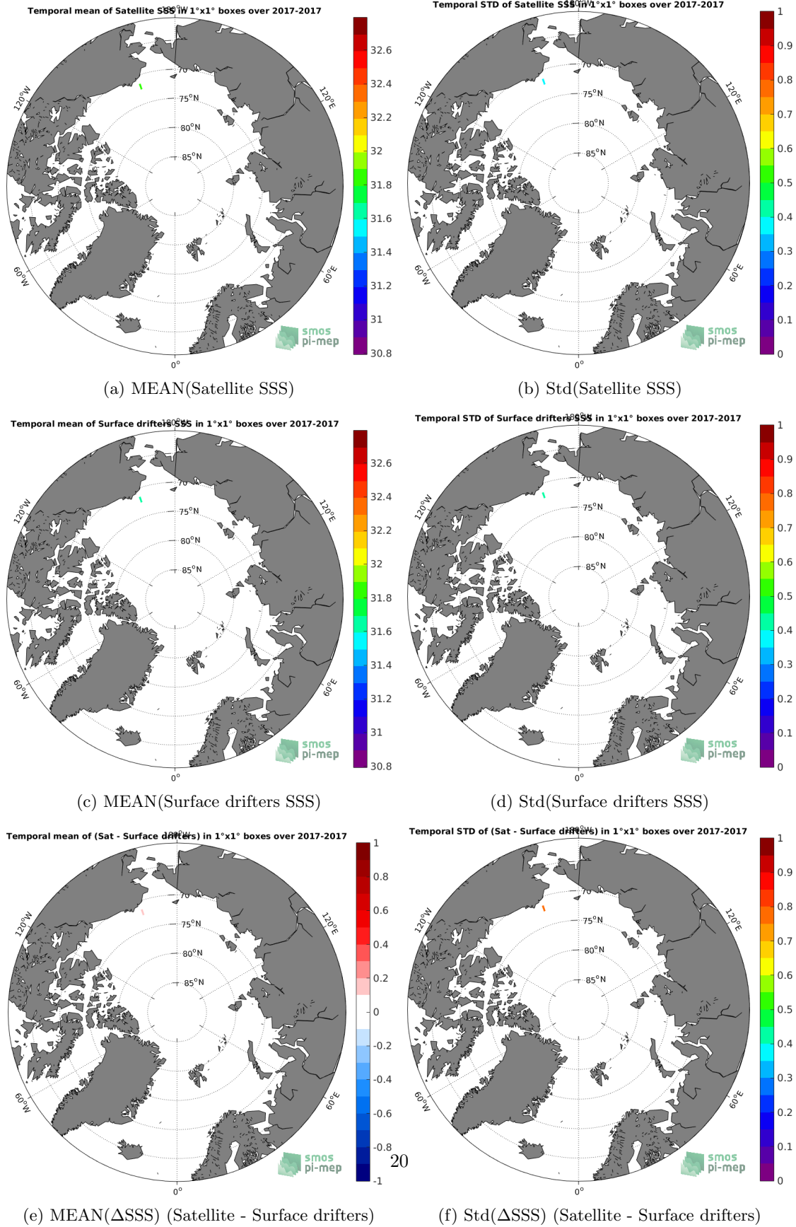
Figure 5: Temporal mean (left) and Std (right) of SSS from SMAP-L3-JPL-V4.3-MONTHLY-60KM (top), Surface drifters (middle), and of \Delta SSS (Satellite - Surface drifters). Only match-up pairs are used to generate these maps.
