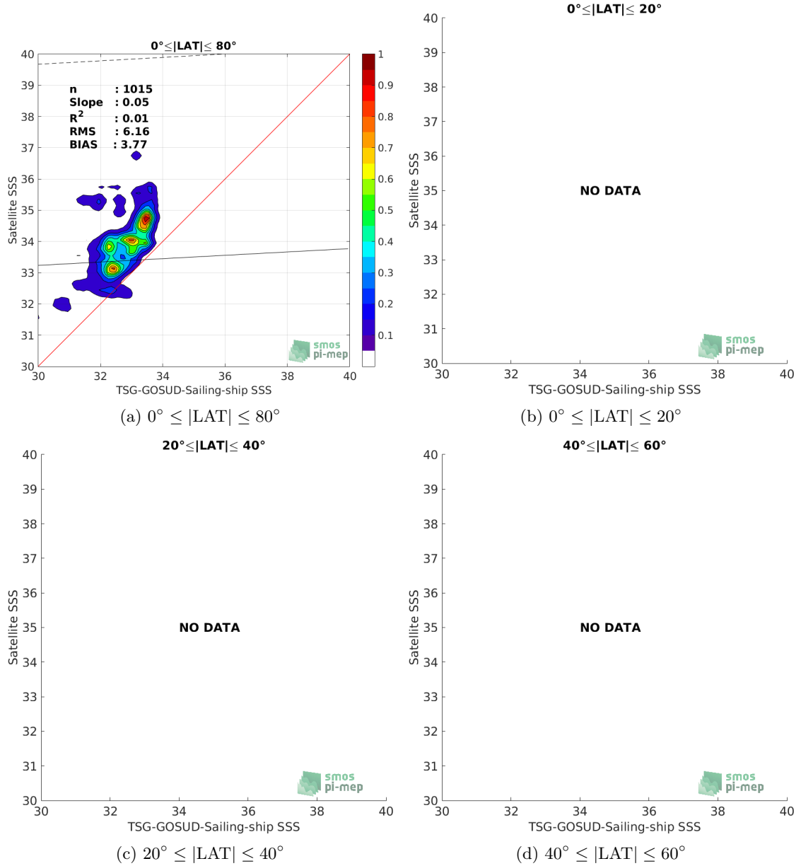
Figure 9: Contour maps of the concentration of SMAP-L3-JPL-V4.2-8DAY-RUNNING-60KM SSS (y-axis) versus TSG-GOSUD-Sailing-ship SSS (x-axis) at match-up pairs for different latitude bands. For each plot, the red line shows x=y . The black thin and dashed lines indicate a linear fit through the data cloud and the \pm 95\% confidence levels, respectively. The number match-up pairs n , the slope and R^2 coefficient of the linear fit, the root mean square (RMS) and the mean bias between satellite and in situ data are indicated for each latitude band in each plots.
