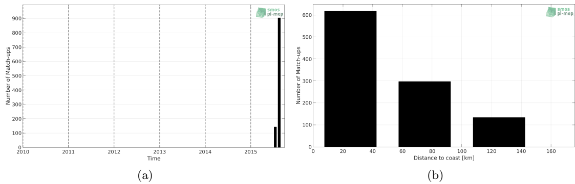
Figure 1: Number of match-ups between TSG-GOSUD-Sailing-ship and SMAP-L3-JPL-V4.2-8DAY-RUNNING-60KM SSS as a function of time (a) and as function of the distance to coast (b) over the Arctic Ocean Pi-MEP region and for the full satellite product period.
