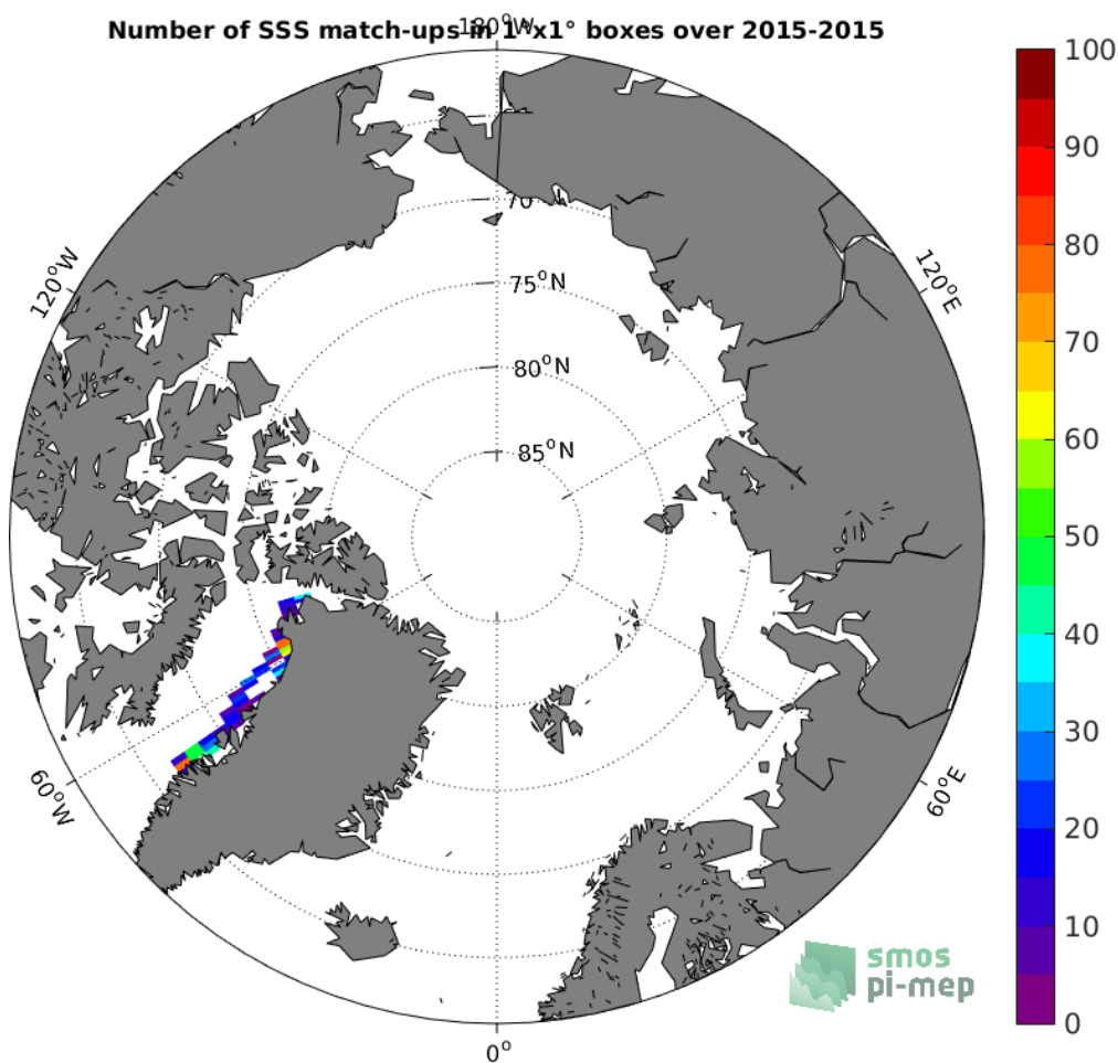
Figure 4: Number of SSS match-ups between TSG-GOSUD-Sailing-ship SSS and the SMAP-L3-JPL-V4.2-8DAY-RUNNING-60KM SSS product for the Arctic Ocean Pi-MEP region over 1^\circ \times 1^\circ boxes and for the full satellite product period.
