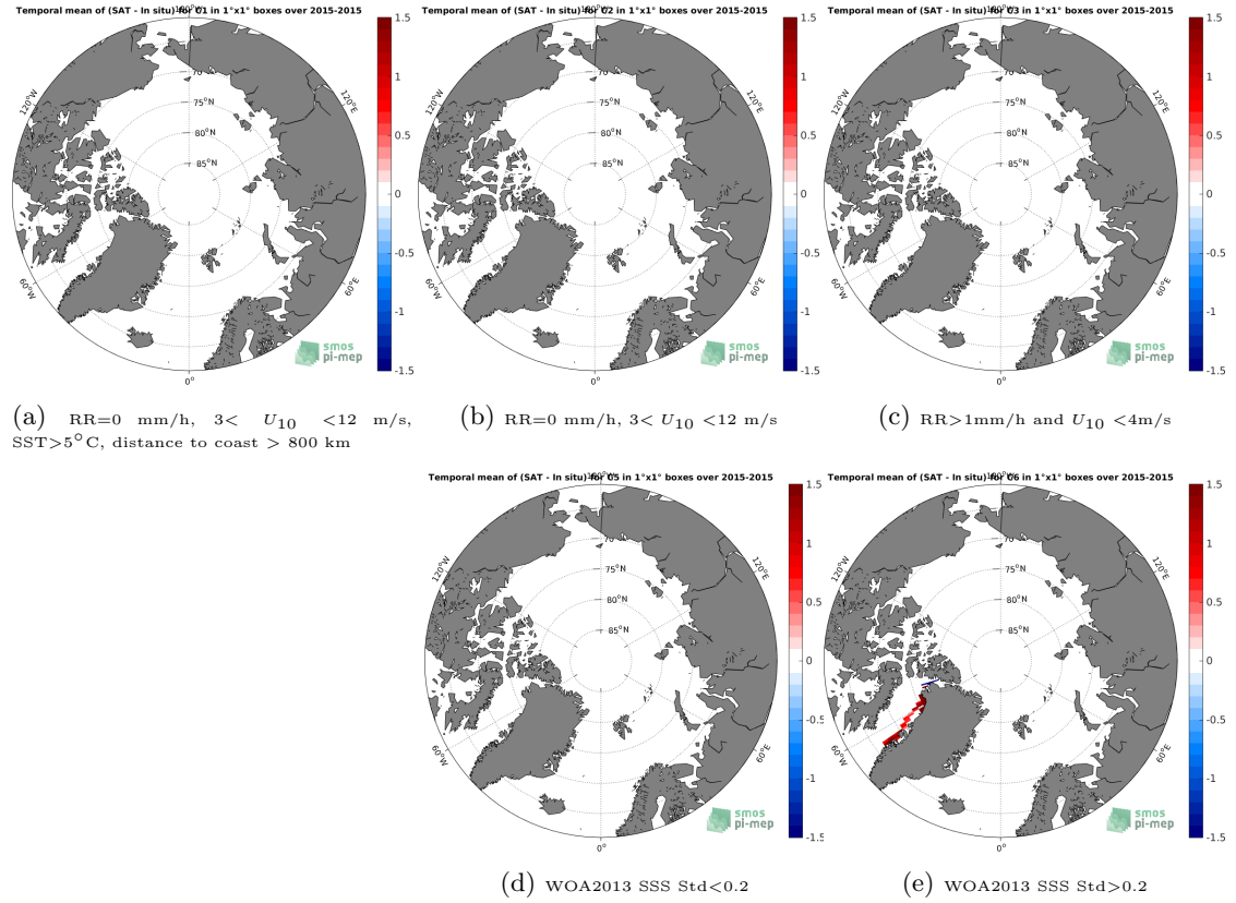
Figure 12: Temporal mean gridded over spatial boxes of size 1^\circ \times 1^\circ of \Delta SSS (SMAP-L3-JPL-V4.2-8DAY-RUNNING-60KM - TSG-GOSUD-Sailing-ship) for 5 different subdatasets corresponding to: RR=0 mm/h, 3 < U_{10} < 12 m/s, SST >5^\circ\text{C} , distance to coast > 800 km (a), RR=0 mm/h, 3 < U_{10} < 12 m/s (b), RR >1 mm/h and U_{10} < 4 m/s (c), WOA2013 SSS Std <0.2 (d), WOA2013 SSS Std >0.2 (e).
