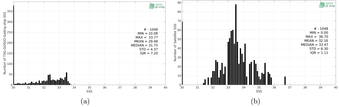
Figure 2: Histograms of SSS from TSG-GOSUD-Sailing-ship (a) and SMAP-L3-JPL-V4.2-8DAY-RUNNING-60KM (b) considering all match-up pairs per bins of 0.1 over the Arctic Ocean Pi-MEP region and for the full satellite product period.
