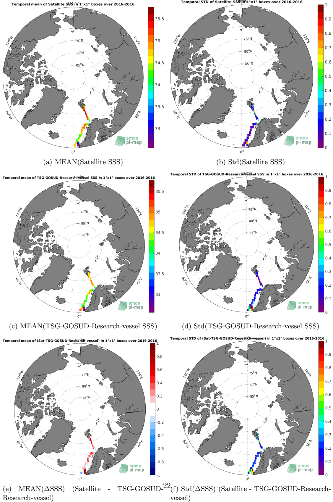
Figure 6: Temporal mean (left) and Std (right) of SSS from SMAP-L3-JPL-V4.2-8DAY-RUNNING-60KM (top), TSG-GOSUD-Research-vessel (middle), and of \Delta SSS (Satellite - TSG-GOSUD-Research-vessel). Only match-up pairs are used to generate these maps.
