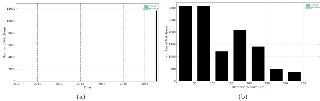
Figure 1: Number of match-ups between TSG-GOSUD-Research-vessel and SMAP-L3-JPL-V4.2-8DAY-RUNNING-60KM SSS as a function of time (a) and as function of the distance to coast (b) over the Arctic Ocean Pi-MEP region and for the full satellite product period.
