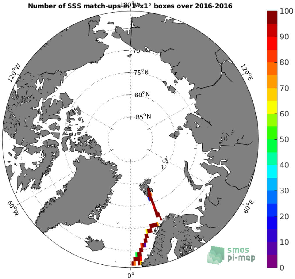
Figure 4: Number of SSS match-ups between TSG-GOSUD-Research-vessel SSS and the SMAP-L3-JPL-V4.2-8DAY-RUNNING-60KM SSS product for the Arctic Ocean Pi-MEP region over 1^\circ \times 1^\circ boxes and for the full satellite product period.
