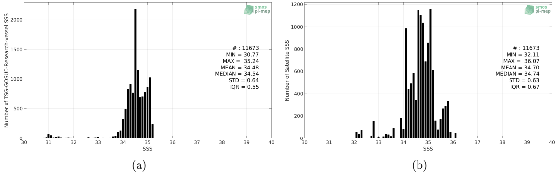
Figure 2: Histograms of SSS from TSG-GOSUD-Research-vessel (a) and SMAP-L3-JPL-V4.2-8DAY-RUNNING-60KM (b) considering all match-up pairs per bins of 0.1 over the Arctic Ocean Pi-MEP region and for the full satellite product period.
