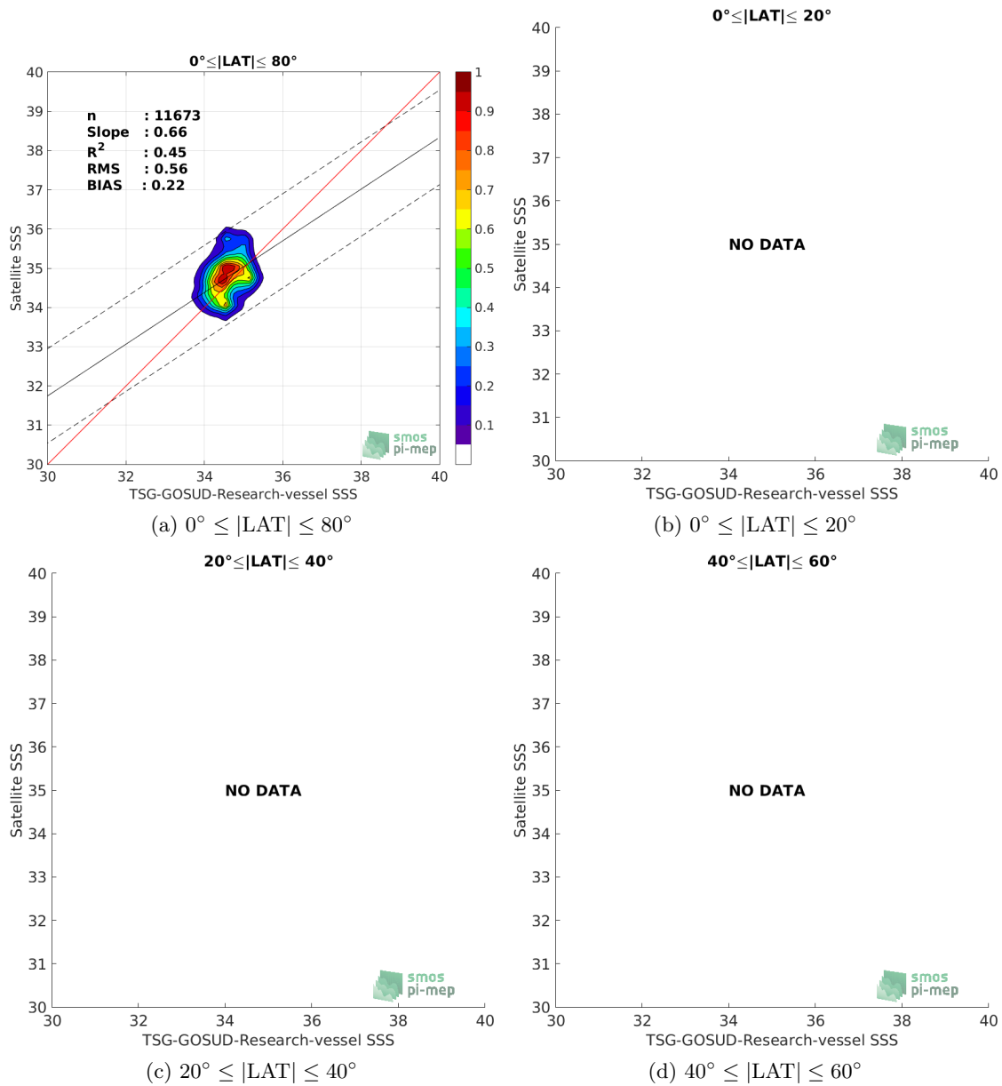
Figure 9: Contour maps of the concentration of SMAP-L3-JPL-V4.2-8DAY-RUNNING-60KM SSS (y-axis) versus TSG-GOSUD-Research-vessel SSS (x-axis) at match-up pairs for different latitude bands. For each plot, the red line shows x=y . The black thin and dashed lines indicate a linear fit through the data cloud and the \pm 95\% confidence levels, respectively. The number match-up pairs n , the slope and R^2 coefficient of the linear fit, the root mean square (RMS) and the mean bias between satellite and in situ data are indicated for each latitude band in each plots.
