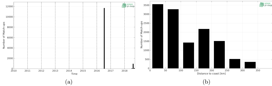
Figure 1: Number of match-ups between TSG-GOSUD-Research-vessel and SMAP-L3-JPL-V4.2-MONTHLY-60KM SSS as a function of time (a) and as function of the distance to coast (b) over the Arctic Ocean Pi-MEP region and for the full satellite product period.
