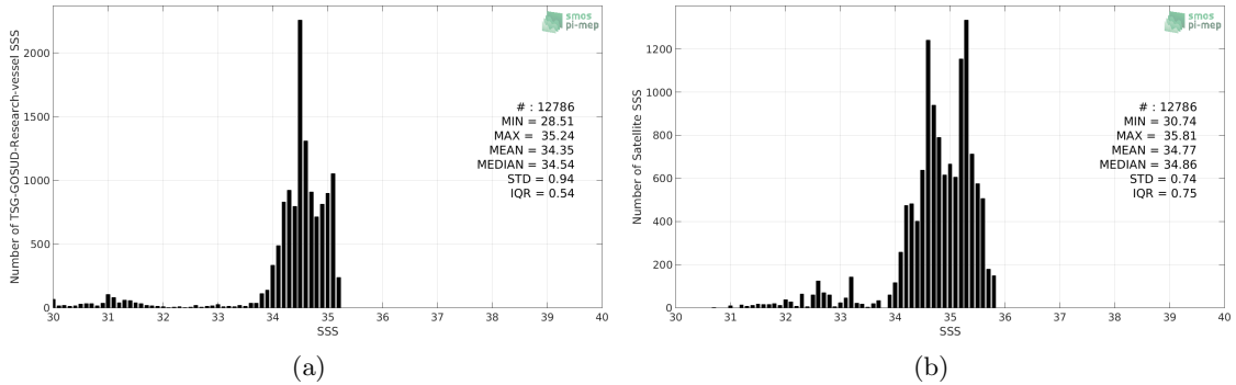
Figure 2: Histograms of SSS from TSG-GOSUD-Research-vessel (a) and SMAP-L3-JPL-V4.2-MONTHLY-60KM (b) considering all match-up pairs per bins of 0.1 over the Arctic Ocean Pi-MEP region and for the full satellite product period.
