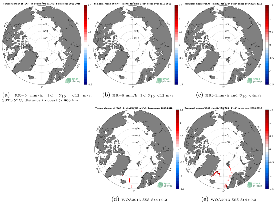
Figure 12: Temporal mean gridded over spatial boxes of size 1^\circ \times 1^\circ of \Delta SSS (SMAP-L3-JPL-V4.2-MONTHLY-60KM - TSG-GOSUD-Research-vessel) for 5 different subdatasets corresponding to:RR=0 mm/h, 3 < U_{10} < 12 m/s, SST>5°C, distance to coast > 800 km (a), RR=0 mm/h, 3 < U_{10} < 12 m/s (b), RR>1mm/h and U_{10} < 4 m/s (c), WOA2013 SSS Std<0.2 (d), WOA2013 SSS Std>0.2 (e).
