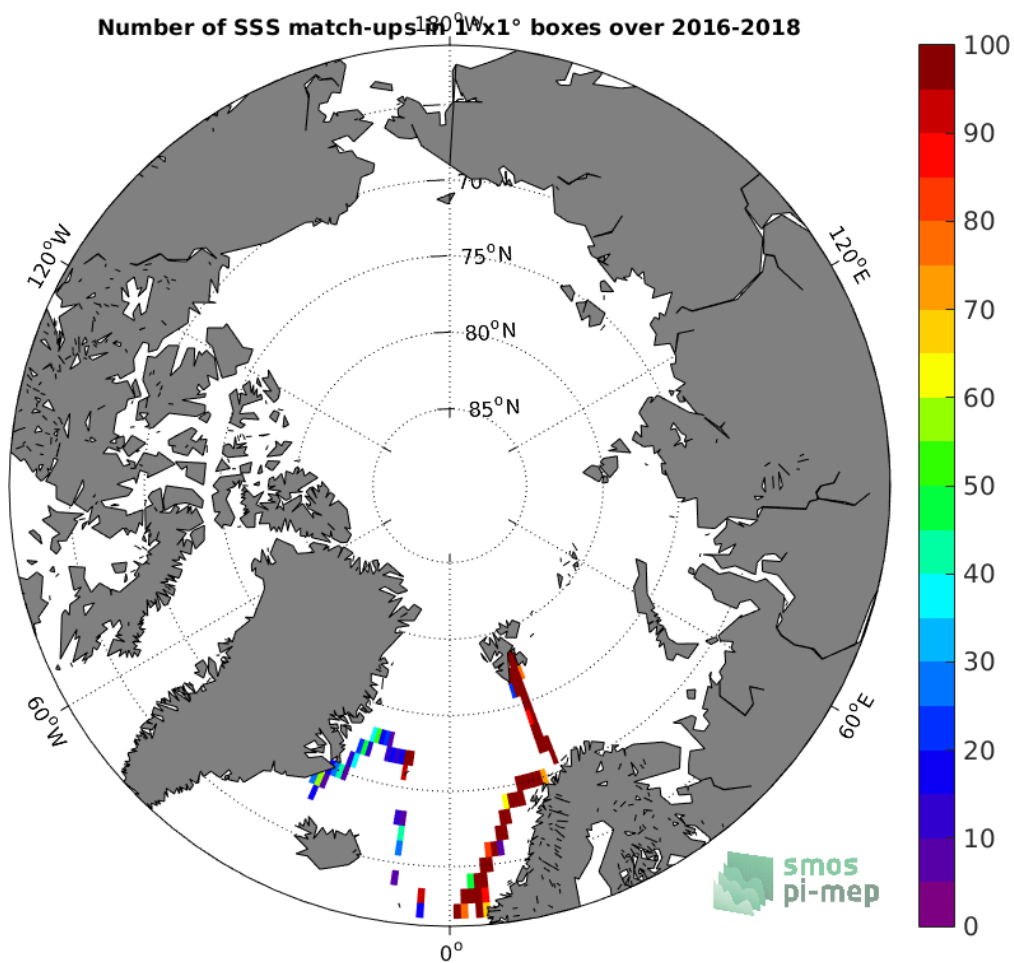
Figure 4: Number of SSS match-ups between TSG-GOSUD-Research-vessel SSS and the SMAP-L3-JPL-V4.2-MONTHLY-60KM SSS product for the Arctic Ocean Pi-MEP region over 1^\circ \times 1^\circ boxes and for the full satellite product period.
