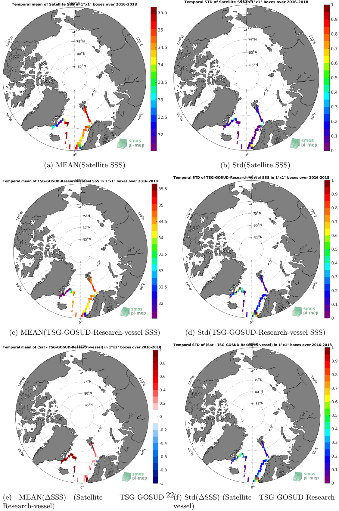
Figure 6: Temporal mean (left) and Std (right) of SSS from SMAP-L3-JPL-V4.2-MONTHLY-60KM (top), TSG-GOSUD-Research-vessel (middle), and of \Delta SSS (Satellite - TSG-GOSUD-Research-vessel). Only match-up pairs are used to generate these maps.
