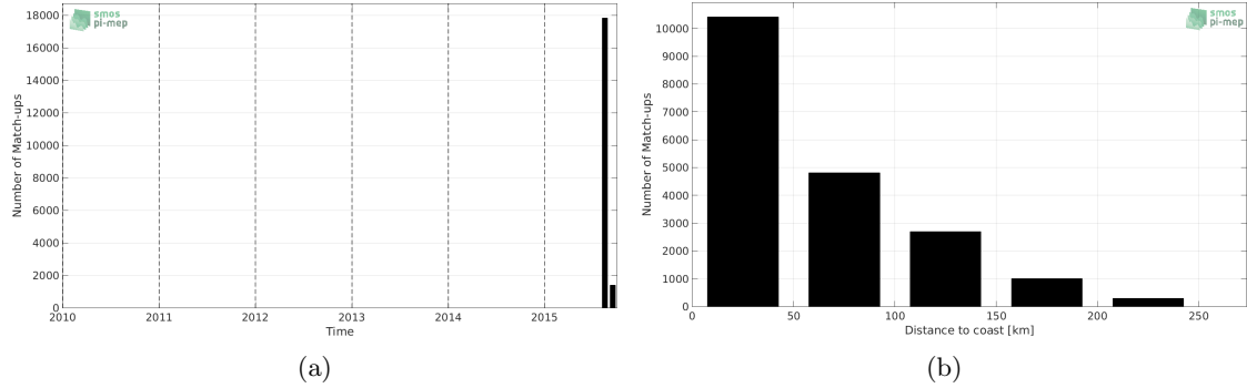
Figure 1: Number of match-ups between TSG-SAMOS and SMAP-L3-JPL-V4-MONTHLY-60KM SSS as a function of time (a) and as function of the distance to coast (b) over the Arctic Ocean Pi-MEP region and for the full satellite product period.
