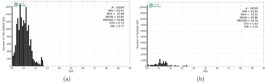
Figure 2: Histograms of SSS from TSG-SAMOS (a) and SMAP-L3-JPL-V4-MONTHLY-60KM (b) considering all match-up pairs per bins of 0.1 over the Arctic Ocean Pi-MEP region and for the full satellite product period.
