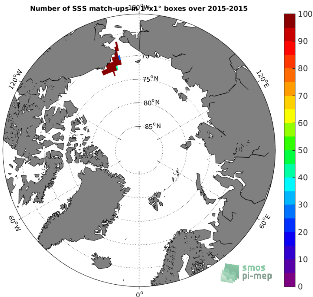
Figure 4: Number of SSS match-ups between TSG-SAMOS SSS and the SMAP-L3-JPL-V4-MONTHLY-60KM SSS product for the Arctic Ocean Pi-MEP region over 1^\circ \times 1^\circ boxes and for the full satellite product period.
