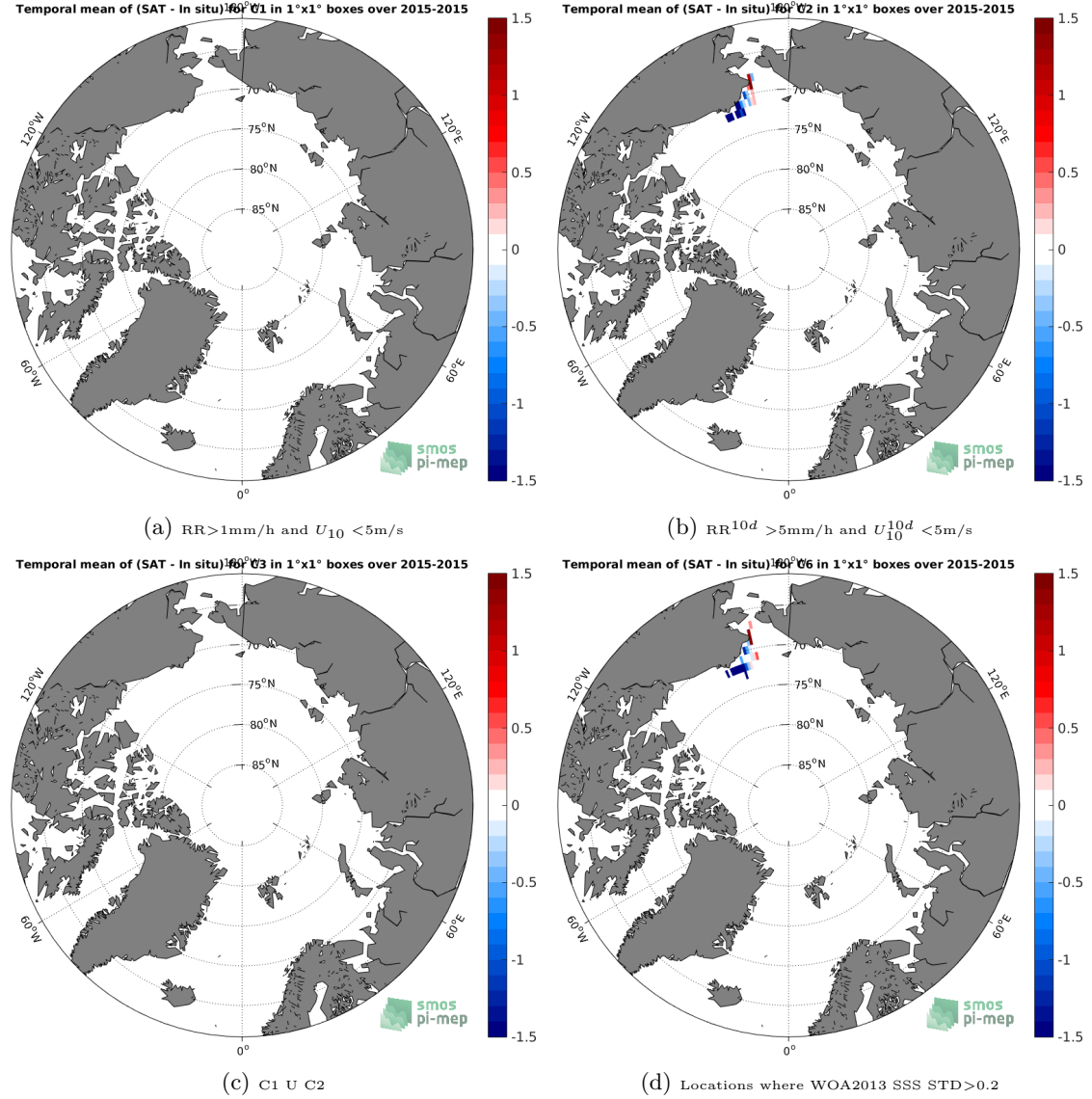
Figure 12: Temporal mean gridded over spatial boxes of size 1^\circ \times 1^\circ of \Delta SSS (SMAP-L3-JPL-V4-MONTHLY-60KM - TSG-SAMOS) for 4 different subdatasets corresponding to: RR > 1\text{mm/h} and U_{10} < 5\text{m/s} (a), RR^{10d} > 5\text{mm/h} and U_{10}^{10d} < 5\text{m/s} (b), C1 U C2 (c), Locations where WOA2013 SSS STD > 0.2 (d).
