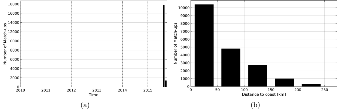
Figure 1: Number of match-ups between TSG-SAMOS and SMAP-L3-JPL-V4-MONTHLY-60KM SSS as a function of time (a) and as function of the distance to coast (b) over the Arctic Ocean Pi-MEP region and for the full satellite product period.
