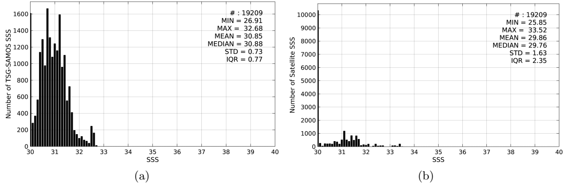
Figure 2: Histograms of SSS from TSG-SAMOS (a) and SMAP-L3-JPL-V4-MONTHLY-60KM (b) considering all match-up pairs per bins of 0.1 over the Arctic Ocean Pi-MEP region and for the full satellite product period.
