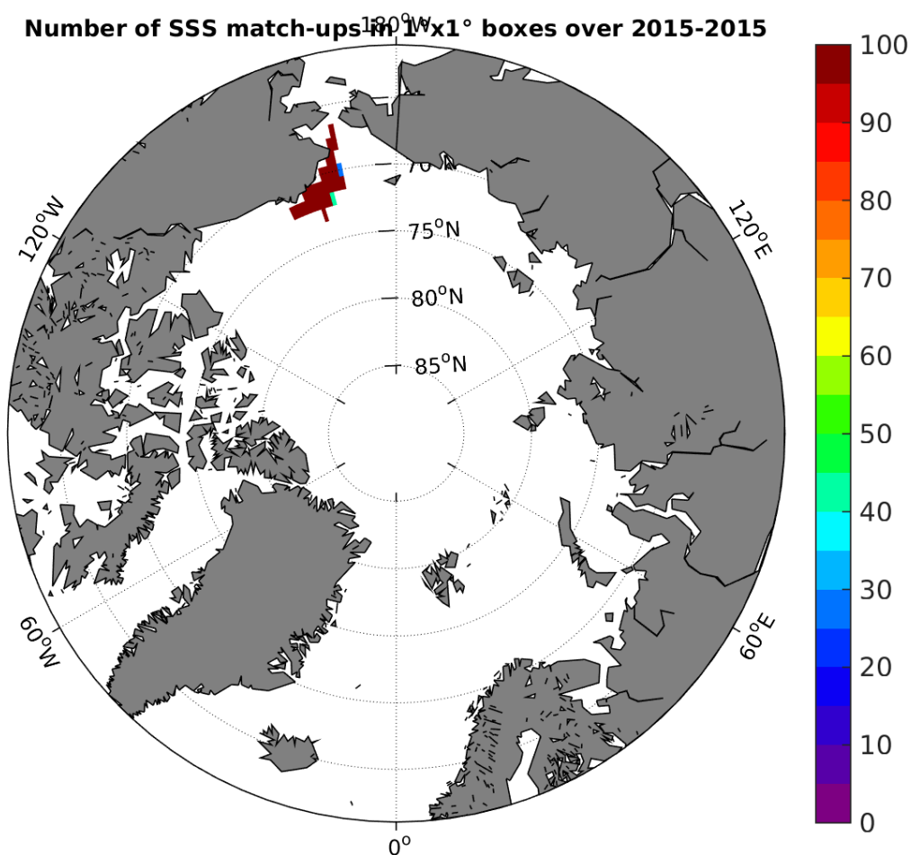
Figure 4: Number of SSS match-ups between TSG-SAMOS SSS and the SMAP-L3-JPL-V4-MONTHLY-60KM SSS product for the Arctic Ocean Pi-MEP region over 1°x1° boxes and for the full satellite product period.
