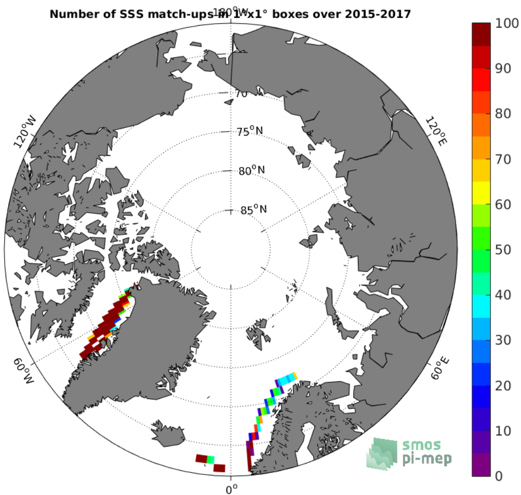
Figure 4: Number of SSS match-ups between TSG-LEGOS-DM SSS and the SMAP-L3-JPL-V4-MONTHLY-60KM SSS product for the Arctic Ocean Pi-MEP region over 1^\circ \times 1^\circ boxes and for the full satellite product period.
