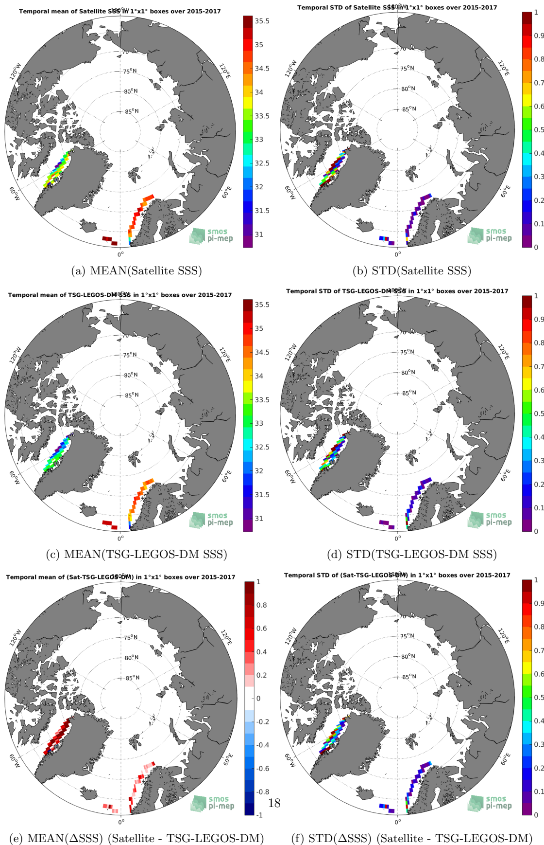
Figure 6: Temporal mean (left) and STD (right) of SSS from SMAP-L3-JPL-V4-MONTHLY-60KM (top), TSG-LEGOS-DM (middle), and of \Delta SSS (Satellite - TSG-LEGOS-DM). Only match-up pairs are used to generate these maps.
