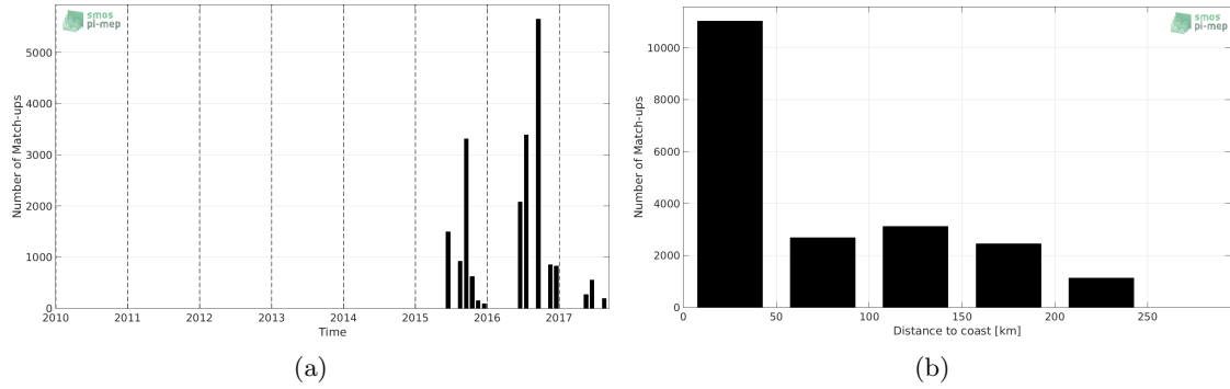
Figure 1: Number of match-ups between TSG-LEGOS-DM and SMAP-L3-JPL-V4-MONTHLY-60KM SSS as a function of time (a) and as function of the distance to coast (b) over the Arctic Ocean Pi-MEP region and for the full satellite product period.
