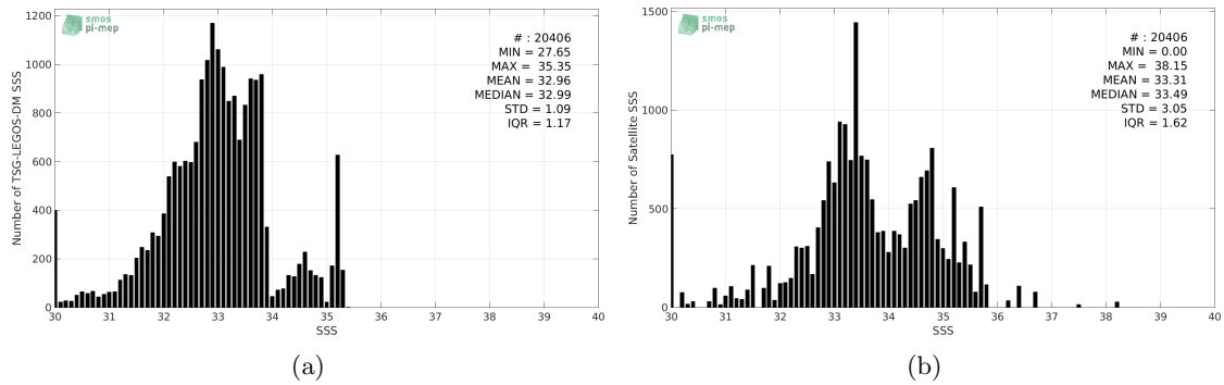
Figure 2: Histograms of SSS from TSG-LEGOS-DM (a) and SMAP-L3-JPL-V4-MONTHLY-60KM (b) considering all match-up pairs per bins of 0.1 over the Arctic Ocean Pi-MEP region and for the full satellite product period.
