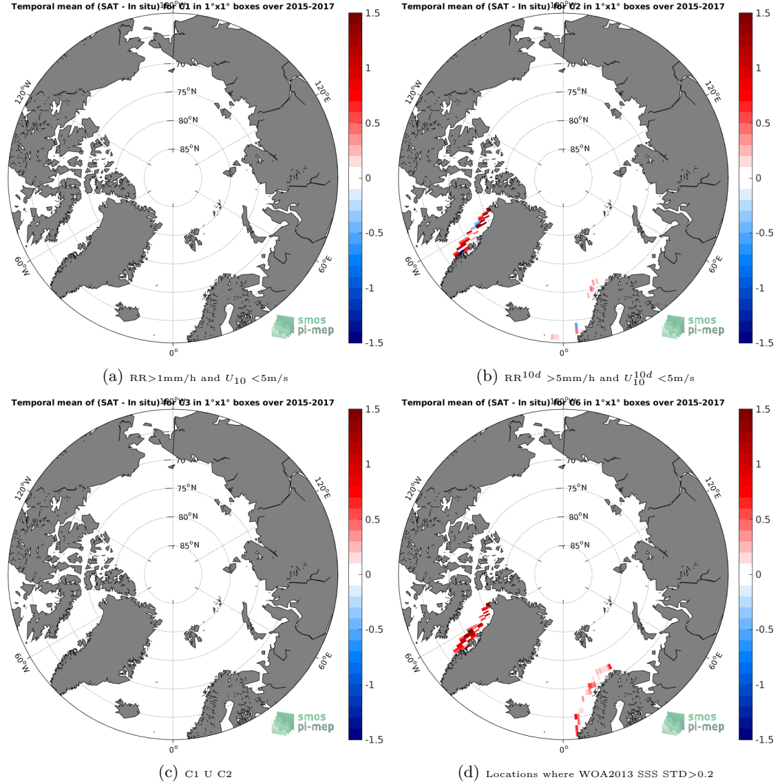
Figure 12: Temporal mean gridded over spatial boxes of size 1^\circ \times 1^\circ of \Delta SSS (SMAP-L3-JPL-V4-MONTHLY-60KM - TSG-LEGOS-DM) for 4 different subdatasets corresponding to: RR > 1\text{mm/h} and U_{10} < 5\text{m/s} (a), RR^{10d} > 5\text{mm/h} and U_{10}^{10d} < 5\text{m/s} (b), C1 U C2 (c), Locations where WOA2013 SSS STD > 0.2 (d).
