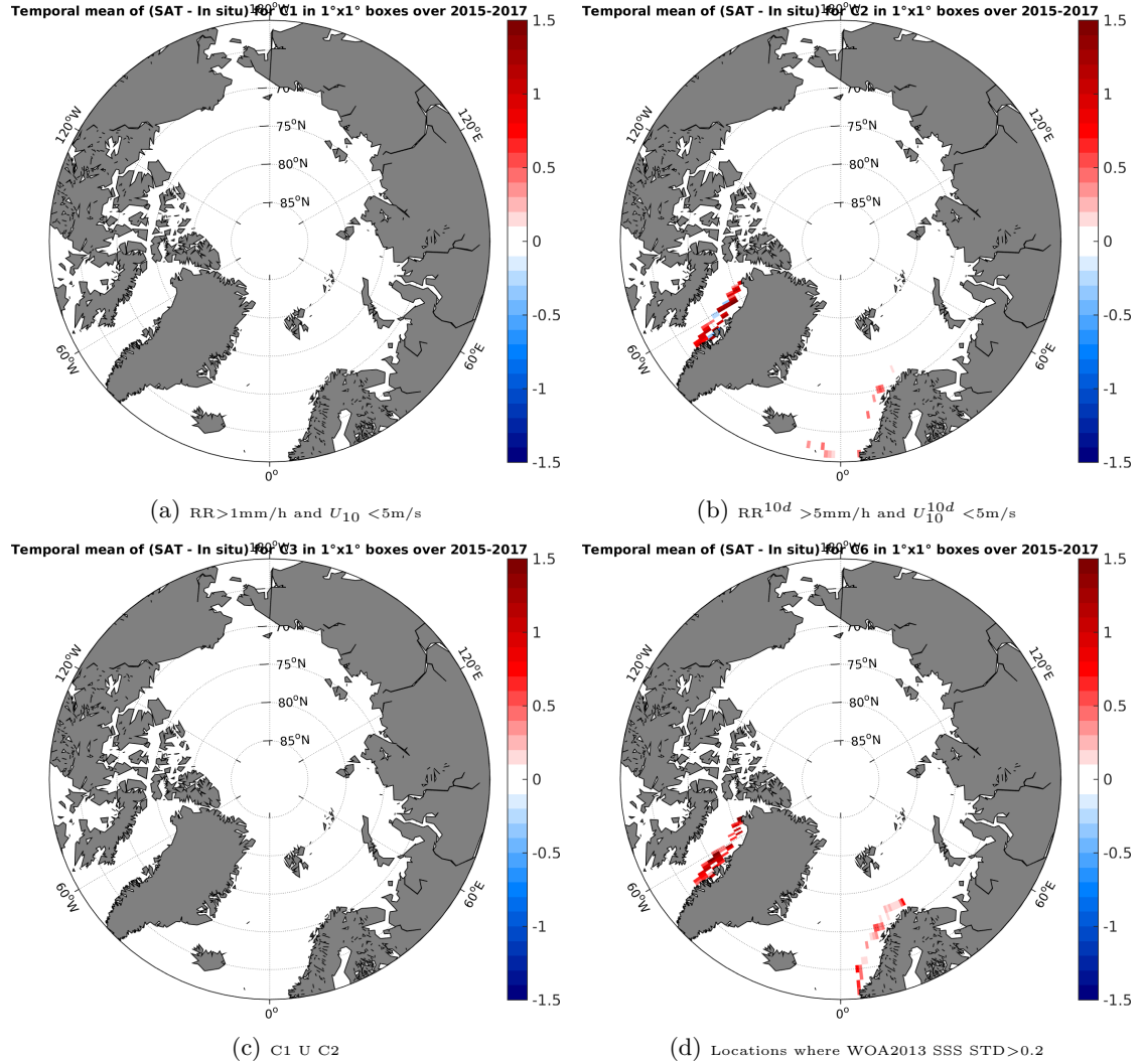
Figure 12: Temporal mean gridded over spatial boxes of size 1^\circ \times 1^\circ of \Delta SSS (SMAP-L3-JPL-V4-MONTHLY-60KM - TSG-LEGOS-DM) for 4 different subdatasets corresponding to: RR > 1 mm/h and U_{10} < 5 m/s (a), RR^{10d} > 5 mm/h and U_{10}^{10d} < 5 m/s (b), C1 U C2 (c), Locations where WOA2013 SSS STD > 0.2 (d).
