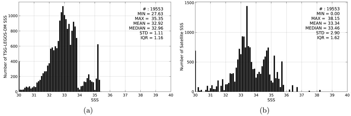
Figure 2: Histograms of SSS from TSG-LEGOS-DM (a) and SMAP-L3-JPL-V4-MONTHLY-60KM (b) considering all match-up pairs per bins of 0.1 over the Arctic Ocean Pi-MEP region and for the full satellite product period.
