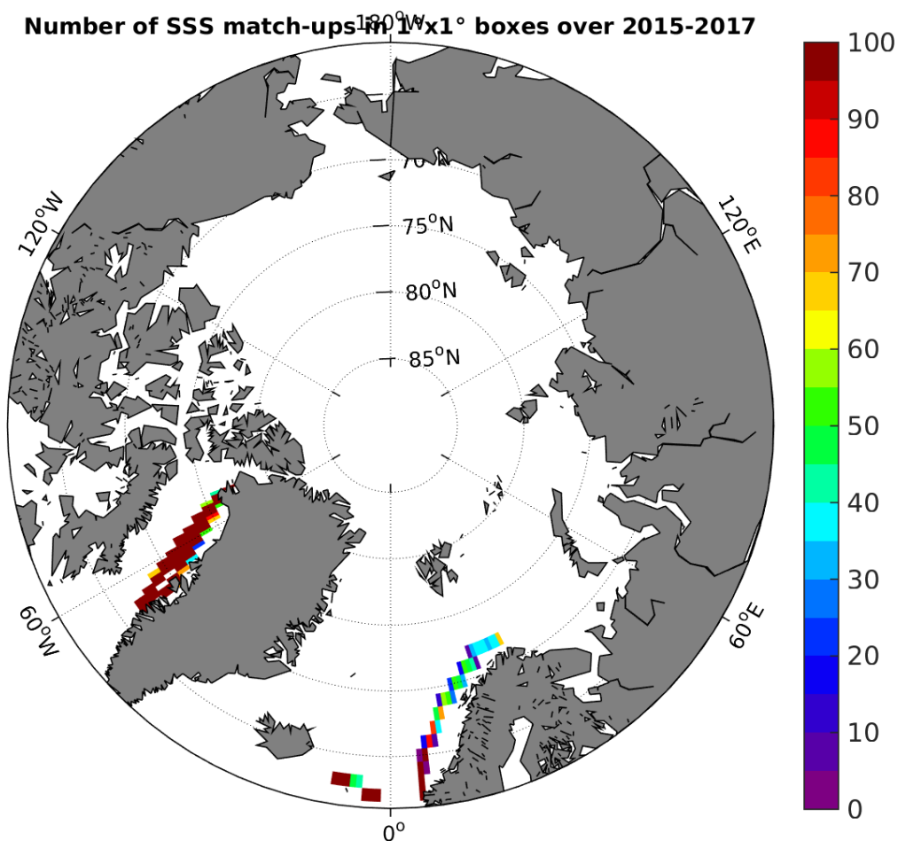
Figure 4: Number of SSS match-ups between TSG-LEGOS-DM SSS and the SMAP-L3-JPL-V4-MONTHLY-60KM SSS product for the Arctic Ocean Pi-MEP region over 1°x1° boxes and for the full satellite product period.
