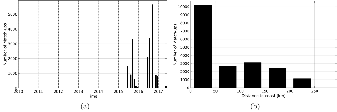
Figure 1: Number of match-ups between TSG-LEGOS-DM and SMAP-L3-JPL-V4-MONTHLY-60KM SSS as a function of time (a) and as function of the distance to coast (b) over the Arctic Ocean Pi-MEP region and for the full satellite product period.
