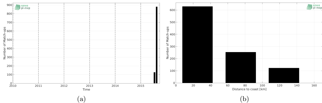
Figure 1: Number of match-ups between TSG-GOSUD-Sailing-ship and SMAP-L3-JPL-V4-MONTHLY-60KM SSS as a function of time (a) and as function of the distance to coast (b) over the Arctic Ocean Pi-MEP region and for the full satellite product period.
