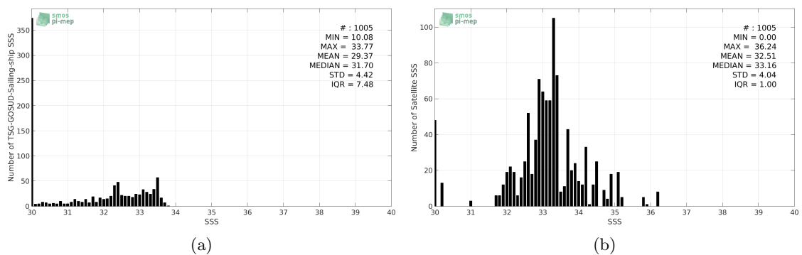
Figure 2: Histograms of SSS from TSG-GOSUD-Sailing-ship (a) and SMAP-L3-JPL-V4-MONTHLY-60KM (b) considering all match-up pairs per bins of 0.1 over the Arctic Ocean Pi-MEP region and for the full satellite product period.
