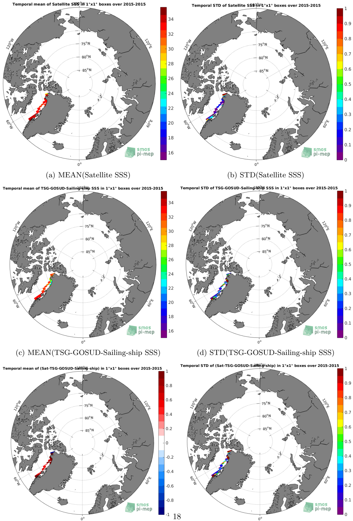
Figure 6: Temporal mean (left) and STD (right) of SSS from SMAP-L3-JPL-V4-MONTHLY-60KM (top), TSG-GOSUD-Sailing-ship (middle), and of \Delta SSS (Satellite - TSG-GOSUD-Sailing-ship). Only match-up pairs are used to generate these maps.
