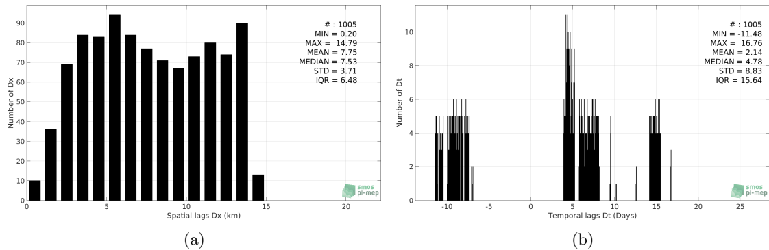
Figure 5: Histograms of the spatial (a) and temporal (b) lags between the time of the TSG-GOSUD-Sailing-ship measurements and the date of the corresponding SMAP-L3-JPL-V4-MONTHLY-60KM SSS product.
