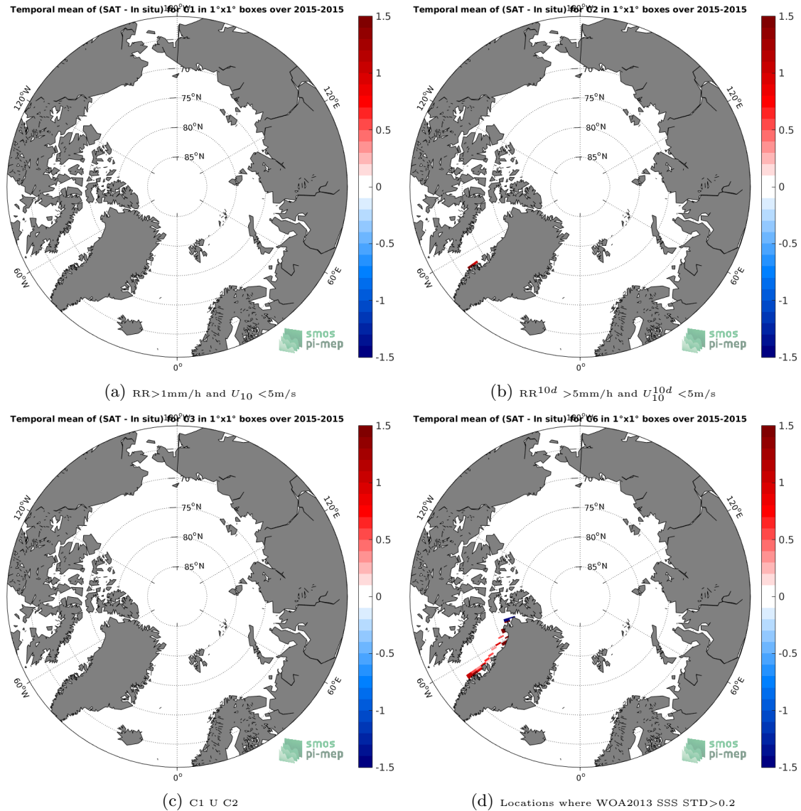
Figure 12: Temporal mean gridded over spatial boxes of size 1^\circ \times 1^\circ of \Delta SSS (SMAP-L3-JPL-V4-MONTHLY-60KM - TSG-GOSUD-Sailing-ship) for 4 different subdatasets corresponding to: RR > 1\text{mm/h} and U_{10} < 5\text{m/s} (a), RR^{10d} > 5\text{mm/h} and U_{10}^{10d} < 5\text{m/s} (b), C1 U C2 (c), Locations where WOA2013 SSS STD > 0.2 (d).
