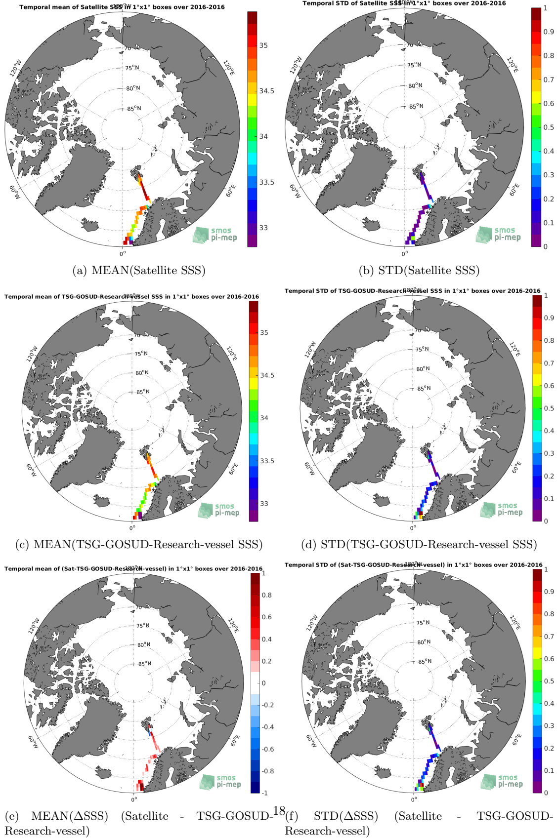
Figure 6: Temporal mean (left) and STD (right) of SSS from SMAP-L3-JPL-V4-MONTHLY-60KM (top), TSG-GOSUD-Research-vessel (middle), and of \Delta SSS (Satellite - TSG-GOSUD-Research-vessel). Only match-up pairs are used to generate these maps.
