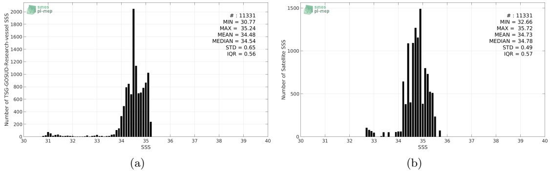
Figure 2: Histograms of SSS from TSG-GOSUD-Research-vessel (a) and SMAP-L3-JPL-V4-MONTHLY-60KM (b) considering all match-up pairs per bins of 0.1 over the Arctic Ocean Pi-MEP region and for the full satellite product period.
