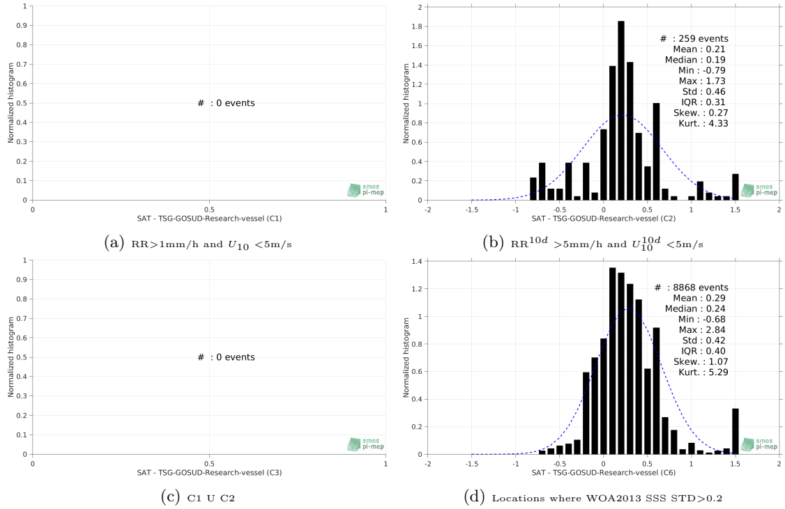
Figure 13: Normalized histogram of \Delta\text{SSS} (SMAP-L3-JPL-V4-MONTHLY-60KM - TSG-GOSUD-Research-vessel) for 6 different subdatasets corresponding to: RR > 1\text{mm/h} and U_{10} < 5\text{m/s} (a), RR^{10d} > 5\text{mm/h} and U_{10}^{10d} < 5\text{m/s} (b), C1 \cup C2 (c), Locations where WOA2013 SSS STD > 0.2 (d).
