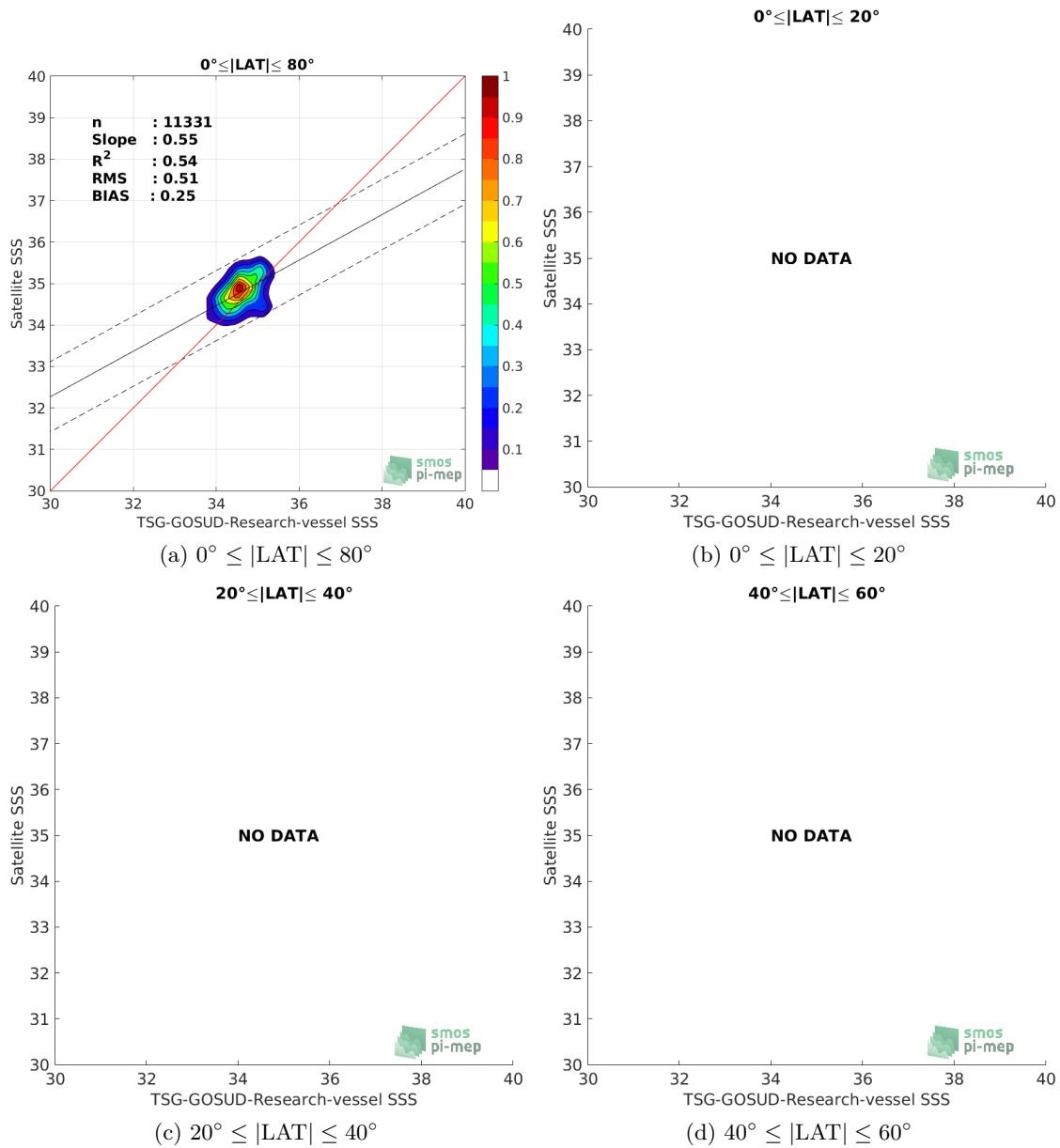
Figure 9: Contour maps of the concentration of SMAP-L3-JPL-V4-MONTHLY-60KM SSS (y-axis) versus TSG-GOSUD-Research-vessel SSS (x-axis) at match-up pairs for different latitude bands. For each plot, the red line shows x=y . The black thin and dashed lines indicate a linear fit through the data cloud and the \pm 95\% confidence levels, respectively. The number match-up pairs n , the slope and R^2 coefficient of the linear fit, the root mean square (RMS) and the mean bias between satellite and in situ data are indicated for each latitude band in each plots.
