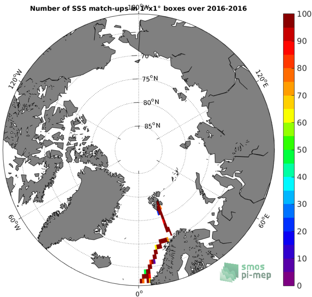
Figure 4: Number of SSS match-ups between TSG-GOSUD-Research-vessel SSS and the SMAP-L3-JPL-V4-MONTHLY-60KM SSS product for the Arctic Ocean Pi-MEP region over 1^{\circ} \times 1^{\circ} boxes and for the full satellite product period.
