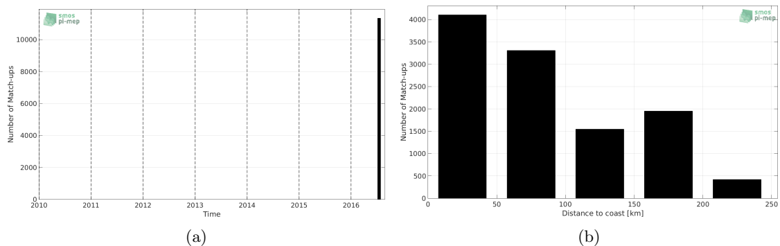
Figure 1: Number of match-ups between TSG-GOSUD-Research-vessel and SMAP-L3-JPL-V4-MONTHLY-60KM SSS as a function of time (a) and as function of the distance to coast (b) over the Arctic Ocean Pi-MEP region and for the full satellite product period.
