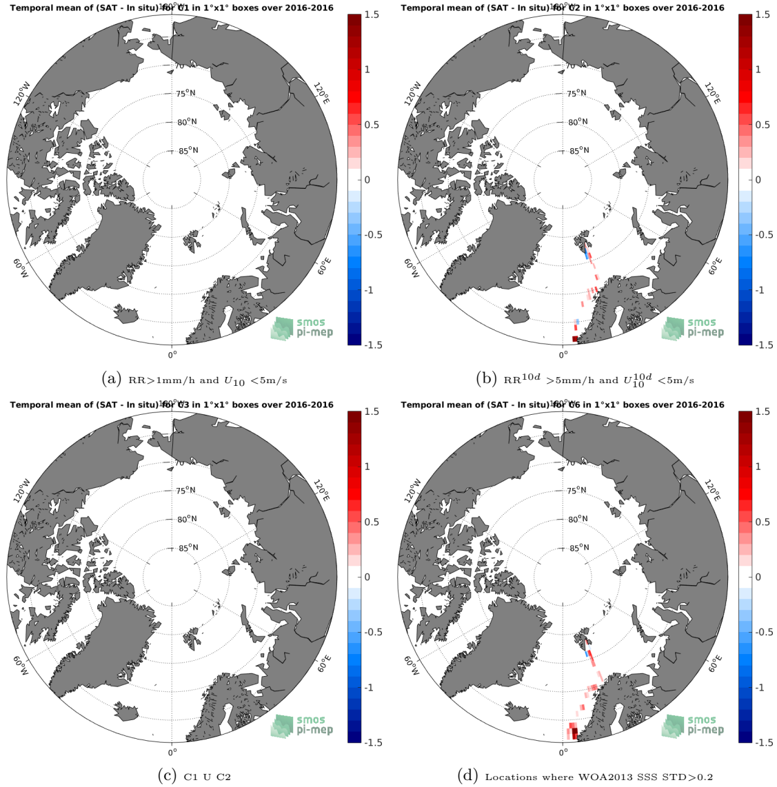
Figure 12: Temporal mean gridded over spatial boxes of size 1^\circ \times 1^\circ of \Delta SSS (SMAP-L3-JPL-V4-MONTHLY-60KM - TSG-GOSUD-Research-vessel) for 4 different subdatasets corresponding to: RR > 1\text{mm/h} and U_{10} < 5\text{m/s} (a), RR^{10d} > 5\text{mm/h} and U_{10}^{10d} < 5\text{m/s} (b), C1 U C2 (c), Locations where WOA2013 SSS STD > 0.2 (d).
