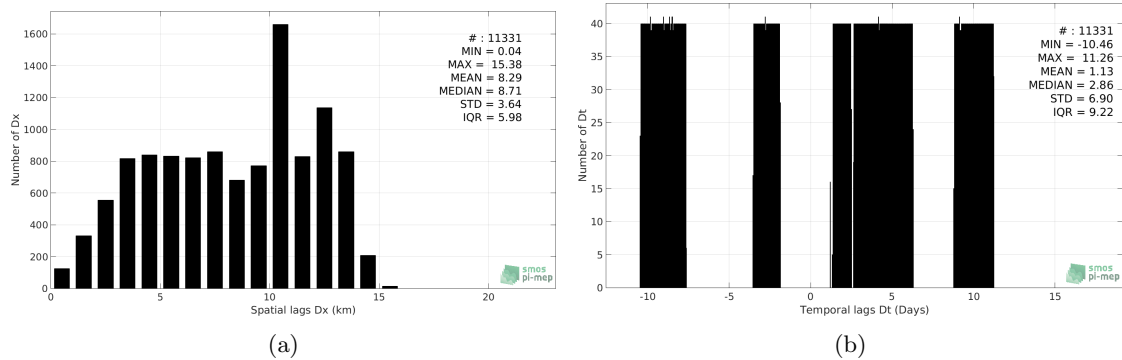
Figure 5: Histograms of the spatial (a) and temporal (b) lags between the time of the TSG-GOSUD-Research-vessel measurements and the date of the corresponding SMAP-L3-JPL-V4-MONTHLY-60KM SSS product.
