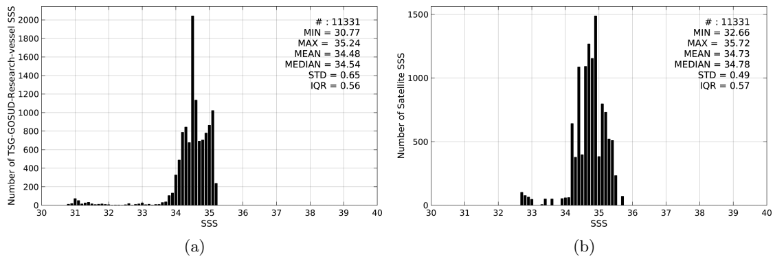
Figure 2: Histograms of SSS from TSG-GOSUD-Research-vessel (a) and SMAP-L3-JPL-V4-MONTHLY-60KM (b) considering all match-up pairs per bins of 0.1 over the Arctic Ocean Pi-MEP region and for the full satellite product period.
