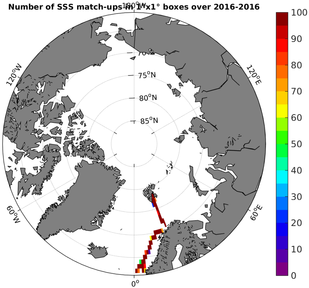
Figure 4: Number of SSS match-ups between TSG-GOSUD-Research-vessel SSS and the SMAP-L3-JPL-V4-MONTHLY-60KM SSS product for the Arctic Ocean Pi-MEP region over 1°x1° boxes and for the full satellite product period.
