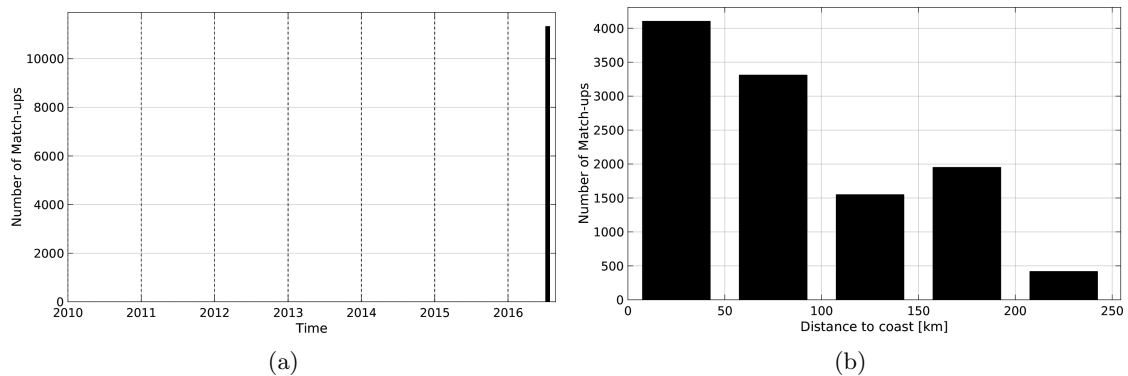
Figure 1: Number of match-ups between TSG-GOSUD-Research-vessel and SMAP-L3-JPL-V4-MONTHLY-60KM SSS as a function of time (a) and as function of the distance to coast (b) over the Arctic Ocean Pi-MEP region and for the full satellite product period.
