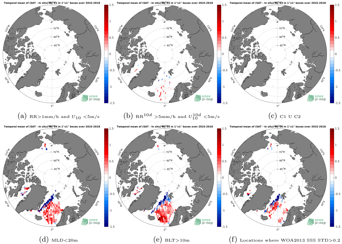
Figure 12: Temporal mean gridded over spatial boxes of size 1^\circ \times 1^\circ of \Delta SSS (SMAP-L3-JPL-V4-MONTHLY-60KM - Argo) for 6 different subdatasets corresponding to:RR>1mm/h and U_{10} < 5 m/s (a), RR^{10d} > 5 mm/h and U_{10}^{10d} < 5 m/s (b), C1 U C2 (c),MLD<20m (d),BLT>10m (e),Locations where WOA2013 SSS STD>0.2 (f).
