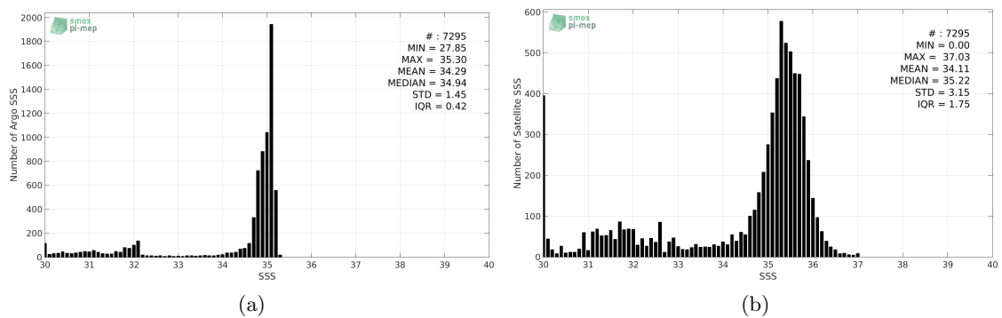
Figure 2: Histograms of SSS from Argo (a) and SMAP-L3-JPL-V4-MONTHLY-60KM (b) considering all match-up pairs per bins of 0.1 over the Arctic Ocean Pi-MEP region and for the full satellite product period.
