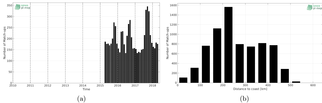
Figure 1: Number of match-ups between Argo and SMAP-L3-JPL-V4-MONTHLY-60KM SSS as a function of time (a) and as function of the distance to coast (b) over the Arctic Ocean Pi-MEP region and for the full satellite product period.
