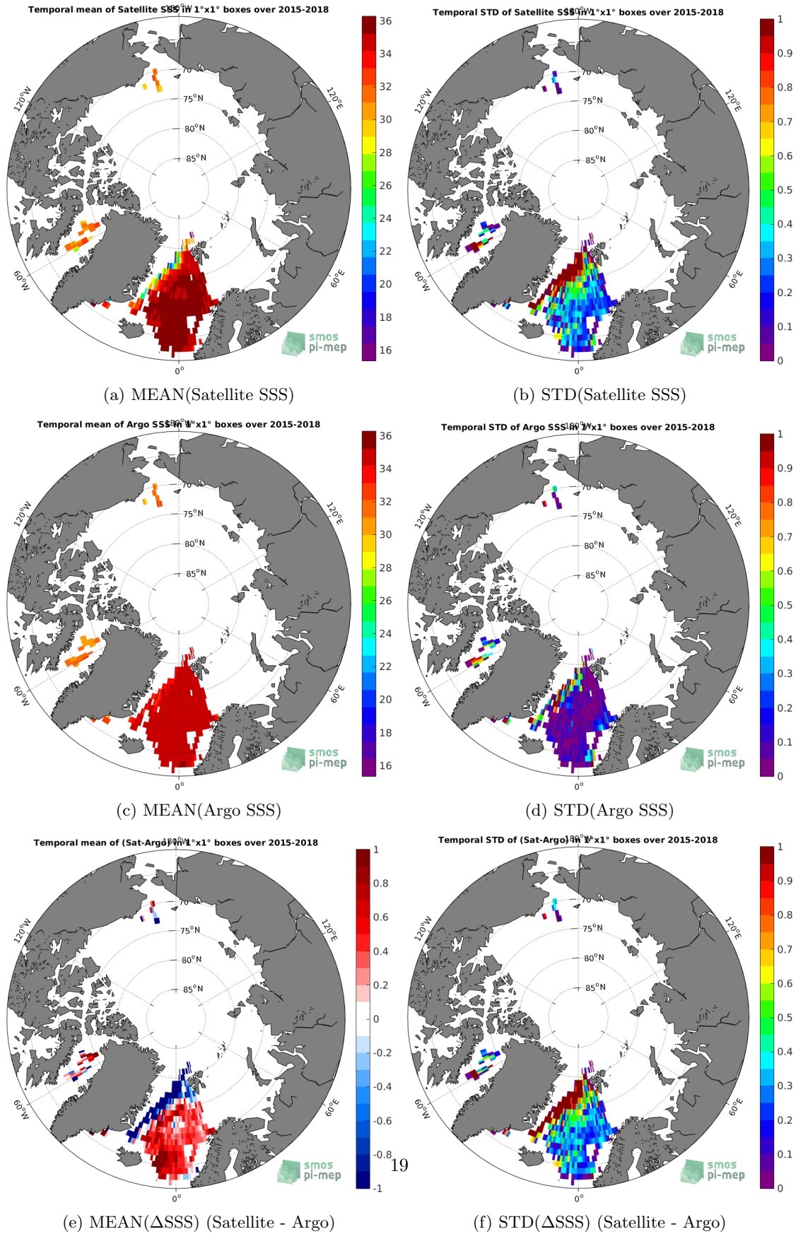
Figure 6: Temporal mean (left) and STD (right) of SSS from SMAP-L3-JPL-V4-MONTHLY-60KM (top), Argo (middle), and of \Delta SSS (Satellite - Argo). Only match-up pairs are used to generate these maps.
