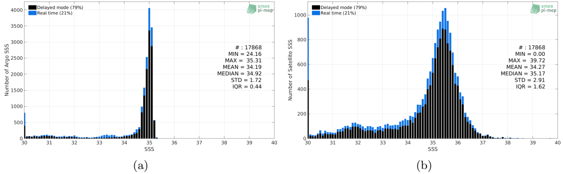
Figure 2: Histograms of SSS from Argo (a) and SMAP SSS L2-AVERAGED v5.0 (JPL) (b) considering all match-up pairs per bins of 0.1 over the Arctic Ocean Pi-MEP region and for the full satellite product period.
