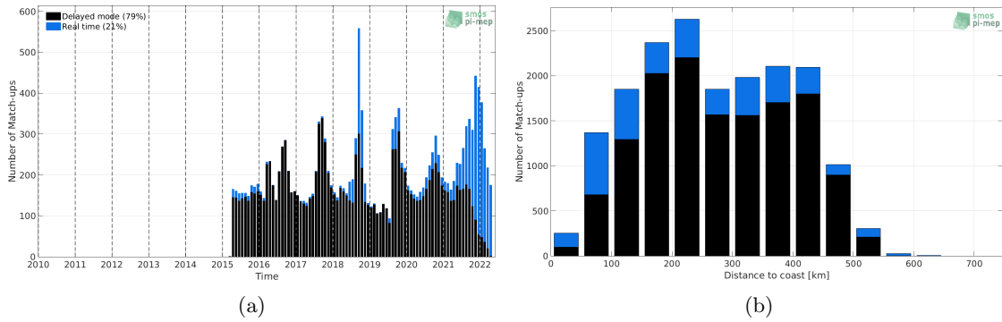
Figure 1: Number of match-ups between Argo and SMAP SSS L2-AVERAGED v5.0 (JPL) SSS as a function of time (a) and as function of the distance to coast (b) over the Arctic Ocean Pi-MEP region and for the full satellite product period.
