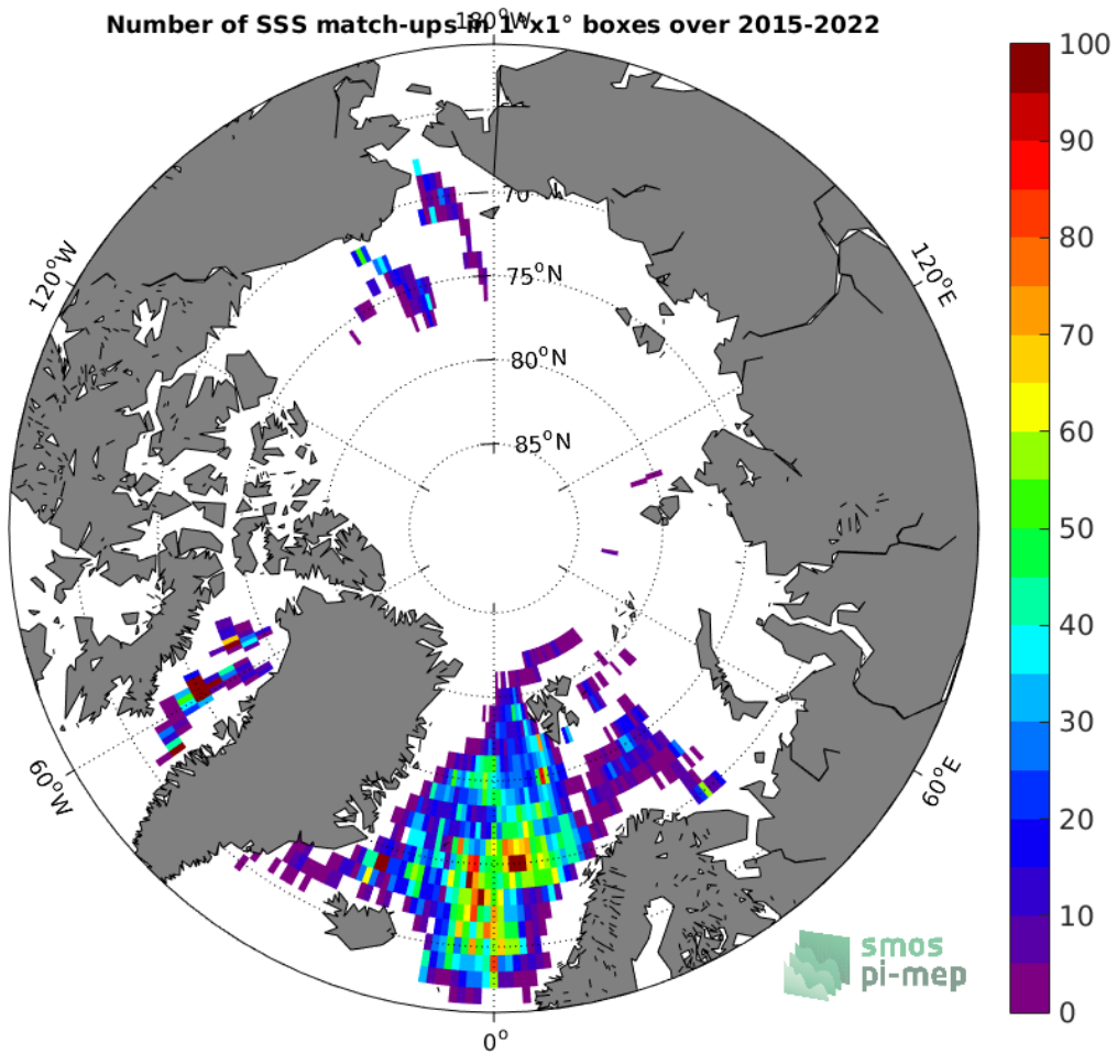
Figure 4: Number of SSS match-ups between Argo SSS and the SMAP SSS L2-AVERAGED v5.0 (JPL) SSS product for the Arctic Ocean Pi-MEP region over 1^\circ \times 1^\circ boxes and for the full satellite product period.
