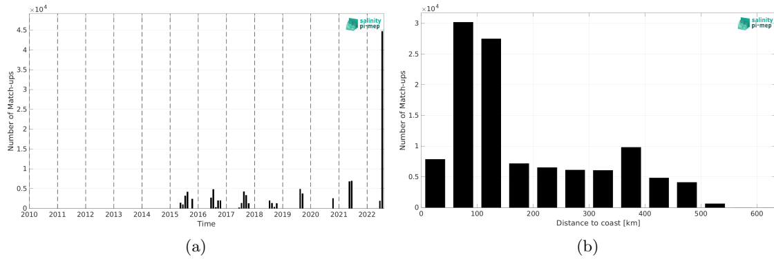
Figure 2: Number of match-ups between TSG (Polarstern) and SMAP SSS L2 v6 (RSS) SSS as a function of time (a) and as function of the distance to coast (b) over the Arctic Ocean Pi-MEP region and for the full satellite product period.
