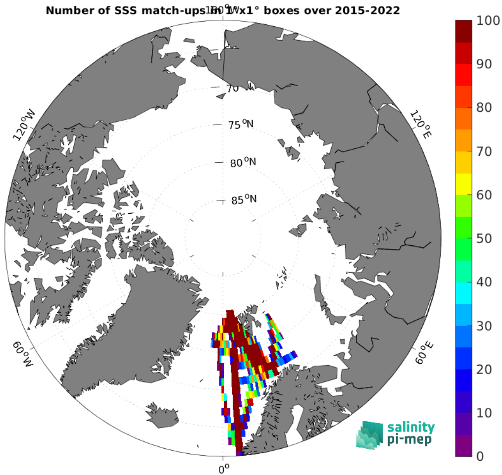
Figure 5: Number of SSS match-ups between TSG (Polarstern) SSS and the SMAP SSS L2 v6 (RSS) SSS product for the Arctic Ocean Pi-MEP region over 1^\circ \times 1^\circ boxes and for the full satellite product period.
