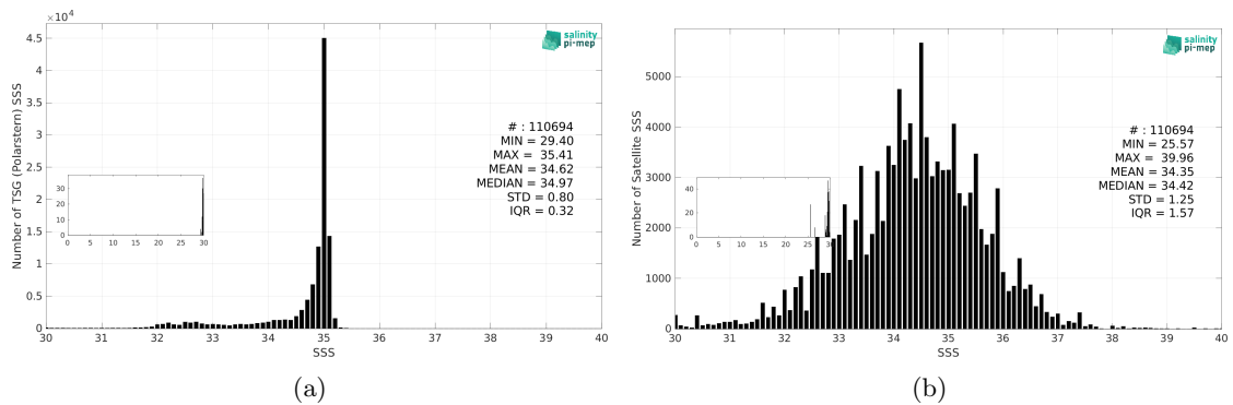
Figure 3: Histograms of SSS from TSG (Polarstern) (a) and SMAP SSS L2 v6 (RSS) (b) considering all match-up pairs per bins of 0.1 over the Arctic Ocean Pi-MEP region and for the full satellite product period.
