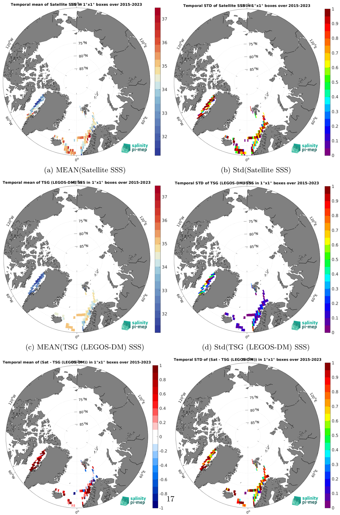
Figure 7: Temporal mean (left) and Std (right) of SSS from SMAP SSS L2 v6 (RSS) (top), TSG (LEGOS-DM) (middle), and of \Delta SSS (Satellite - TSG (LEGOS-DM)). Only match-up pairs are used to generate these maps.
