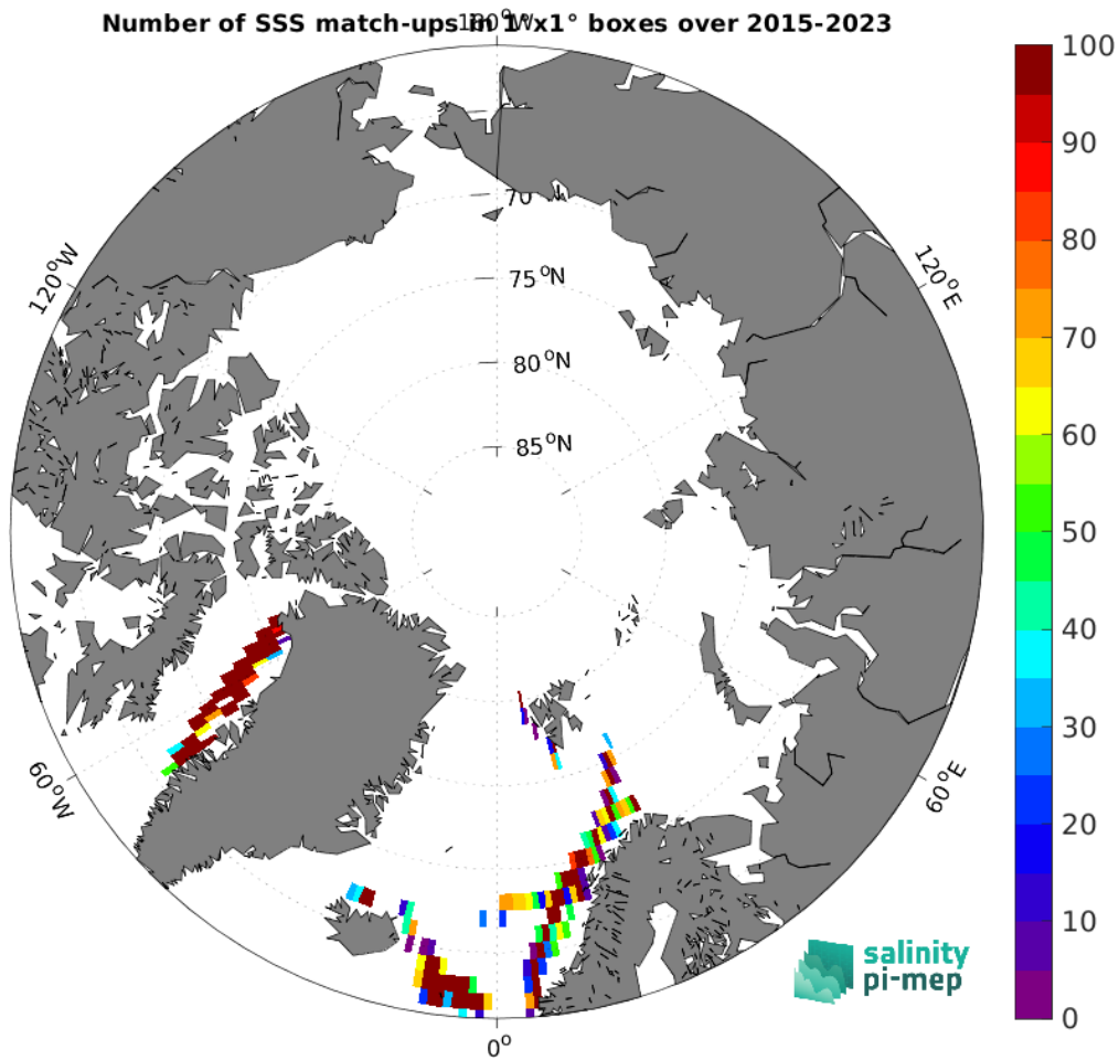
Figure 5: Number of SSS match-ups between TSG (LEGOS-DM) SSS and the SMAP SSS L2 v6 (RSS) SSS product for the Arctic Ocean Pi-MEP region over 1^\circ \times 1^\circ boxes and for the full satellite product period.
