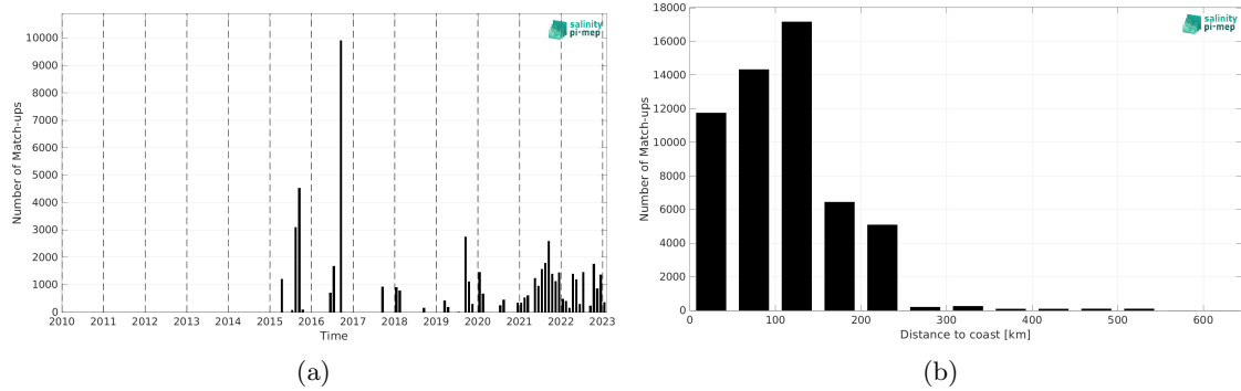
Figure 2: Number of match-ups between TSG (LEGOS-DM) and SMAP SSS L2 v6 (RSS) SSS as a function of time (a) and as function of the distance to coast (b) over the Arctic Ocean Pi-MEP region and for the full satellite product period.
