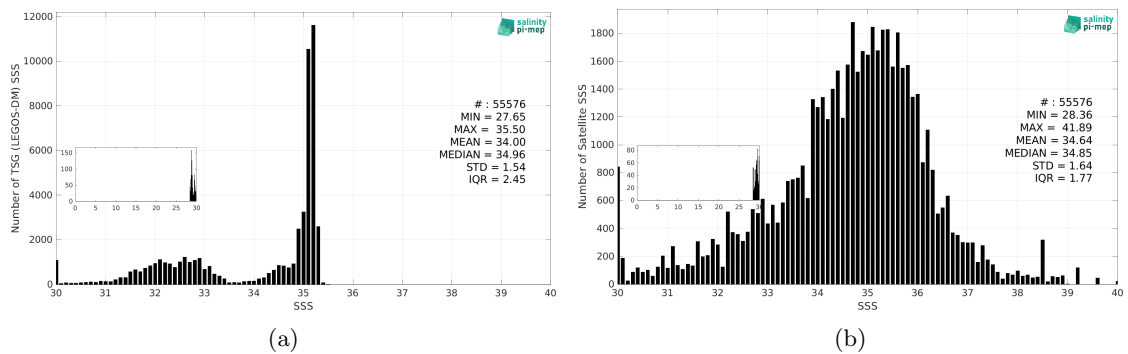
Figure 3: Histograms of SSS from TSG (LEGOS-DM) (a) and SMAP SSS L2 v6 (RSS) (b) considering all match-up pairs per bins of 0.1 over the Arctic Ocean Pi-MEP region and for the full satellite product period.
