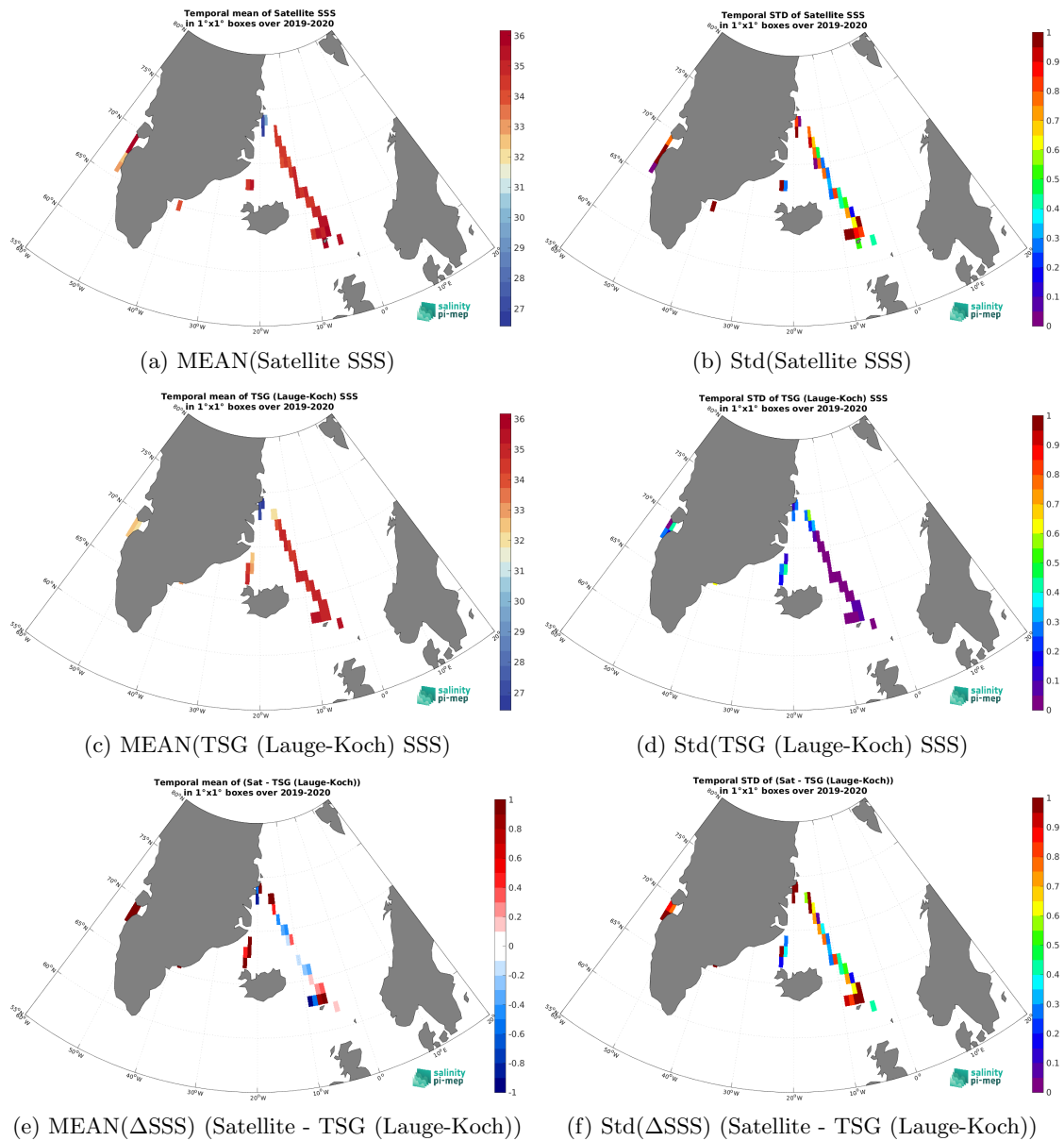
Figure 7: Temporal mean (left) and Std (right) of SSS from SMAP SSS L2 v6 (RSS) (top), TSG (Lauge-Koch) (middle), and of \Delta SSS (Satellite - TSG (Lauge-Koch)). Only match-up pairs are used to generate these maps.
