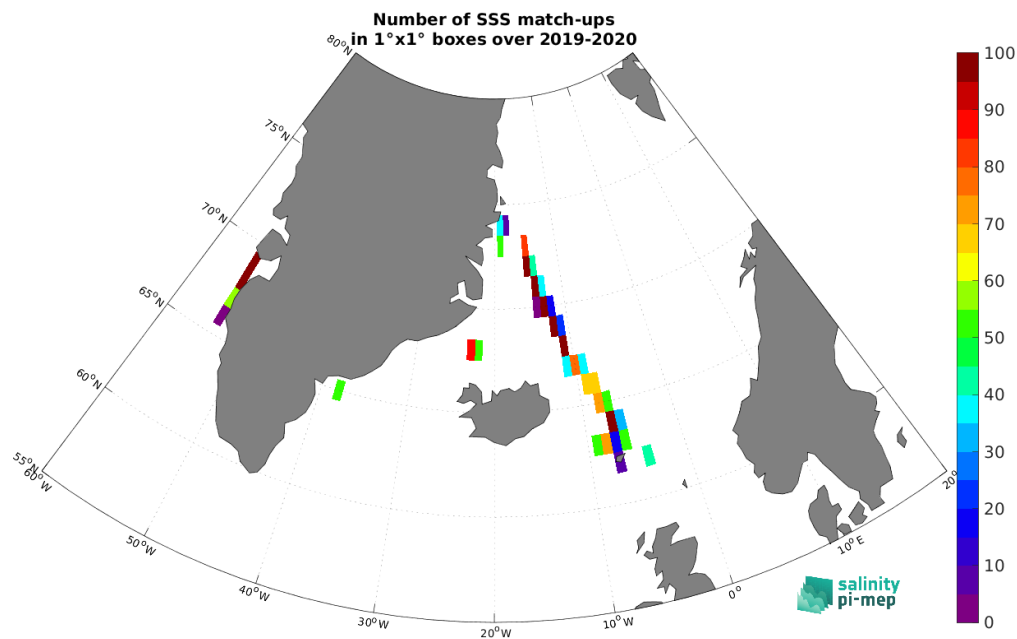
Figure 5: Number of SSS match-ups between TSG (Lauge-Koch) SSS and the SMAP SSS L2 v6 (RSS) SSS product for the Arctic Ocean Pi-MEP region over 1^\circ \times 1^\circ boxes and for the full satellite product period.
