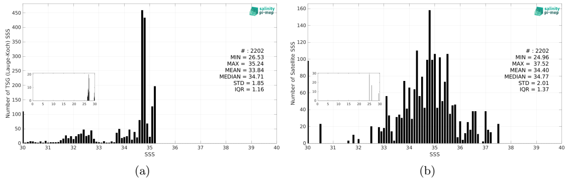
Figure 3: Histograms of SSS from TSG (Lauge-Koch) (a) and SMAP SSS L2 v6 (RSS) (b) considering all match-up pairs per bins of 0.1 over the Arctic Ocean Pi-MEP region and for the full satellite product period.
