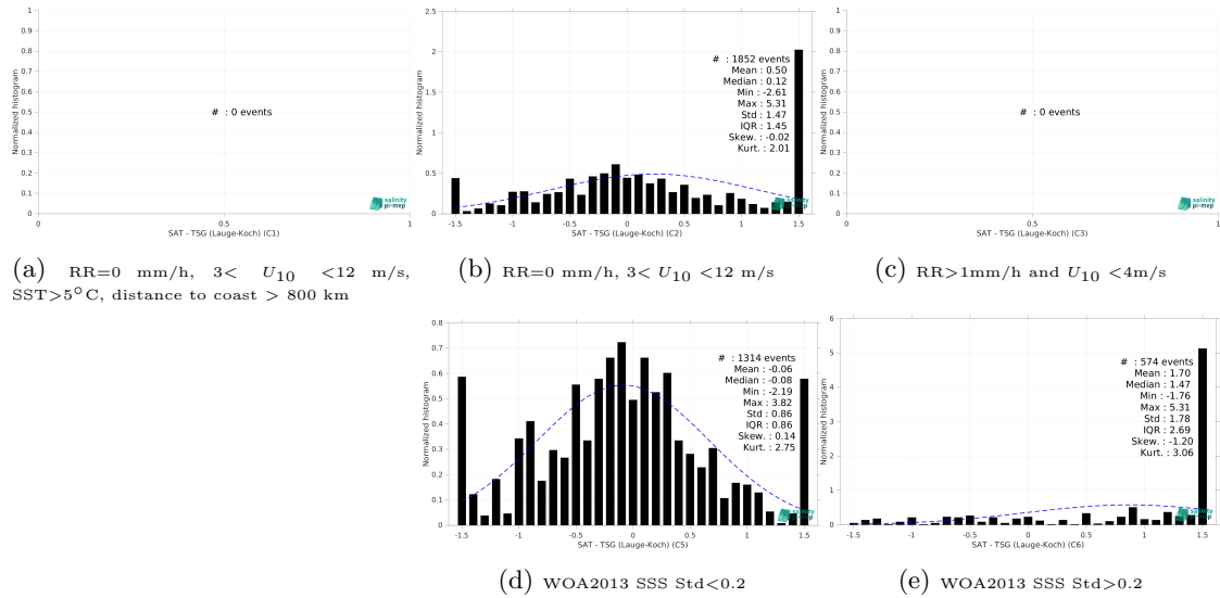
Figure 15: Normalized histogram of \Delta SSS (SMAP SSS L2 v6 (RSS) - TSG (Lauge-Koch)) for 5 different subdatasets corresponding to: RR=0 mm/h, 3 < U_{10} < 12 m/s, SST > 5°C, distance to coast > 800 km (a), RR=0 mm/h, 3 < U_{10} < 12 m/s (b), RR > 1mm/h and U_{10} < 4 m/s (c), WOA2013 SSS Std < 0.2 (d), WOA2013 SSS Std > 0.2 (e).
