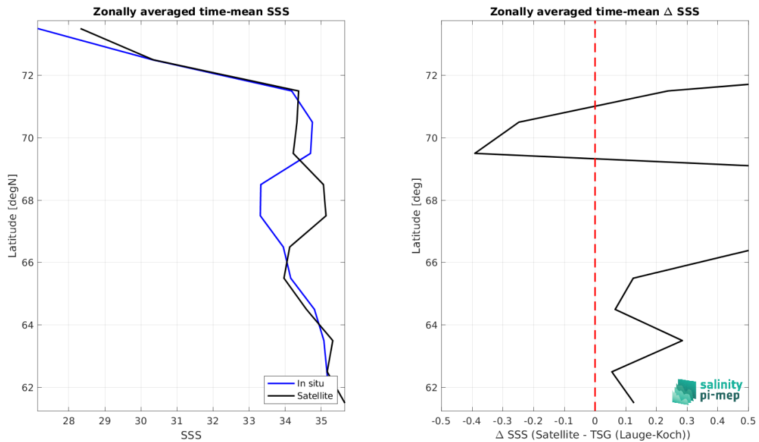
Figure 9: Left panel: Zonal mean SSS from SMAP SSS L2 v6 (RSS) satellite product (black) and from TSG (Lauge-Koch) (blue). Right panel: Zonal mean of \Delta SSS (Satellite - TSG (Lauge-Koch)) for all the collected Pi-MEP match-up pairs estimated over the full satellite product period.
