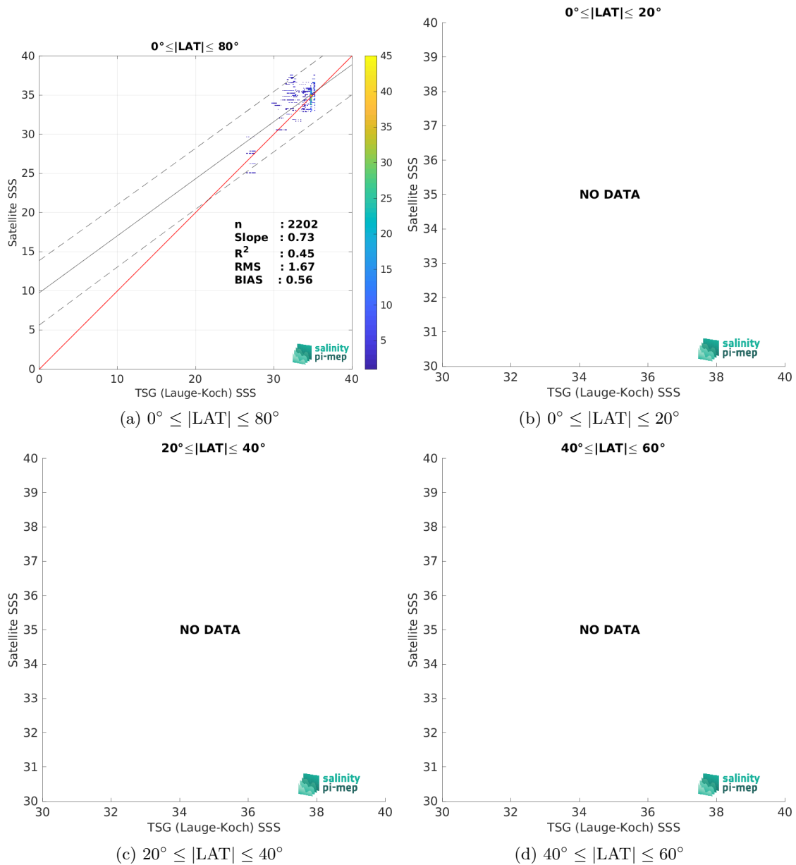
Figure 10: Contour maps of the concentration of SMAP SSS L2 v6 (RSS) SSS (y-axis) versus TSG (Laue-Koch) SSS (x-axis) at match-up pairs for different latitude bands. For each plot, the red line shows x=y . The black thin and dashed lines indicate a linear fit through the data cloud and the \pm 95\% confidence levels, respectively. The number match-up pairs n , the slope and R^2 coefficient of the linear fit, the root mean square (RMS) and the mean bias between satellite and in situ data are indicated for each latitude band in each plots.
