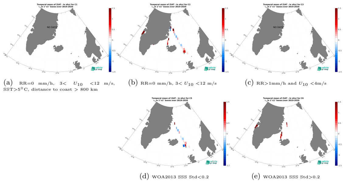
Figure 14: Temporal mean gridded over spatial boxes of size 1^\circ \times 1^\circ of \Delta SSS (SMAP SSS L2 v6 (RSS) - TSG (Lauge-Koch)) for 5 different subdatasets corresponding to:RR=0 mm/h, 3 < U_{10} < 12 m/s, SST > 5^\circ\text{C} , distance to coast > 800 km (a), RR=0 mm/h, 3 < U_{10} < 12 m/s (b), RR > 1 mm/h and U_{10} < 4 m/s (c), WOA2013 SSS Std < 0.2 (d), WOA2013 SSS Std > 0.2 (e).
