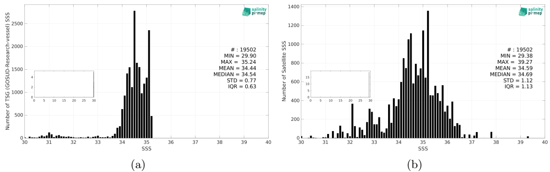
Figure 3: Histograms of SSS from TSG (GOSUD-Research-vessel) (a) and SMAP SSS L2 v6 (RSS) (b) considering all match-up pairs per bins of 0.1 over the Arctic Ocean Pi-MEP region and for the full satellite product period.
