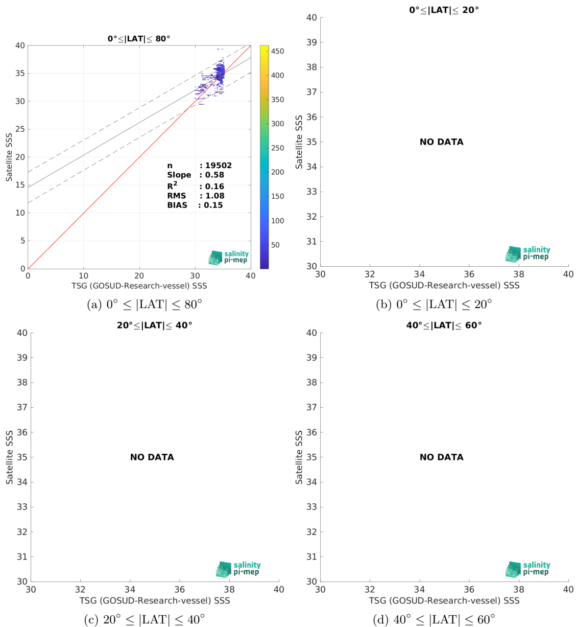
Figure 10: Contour maps of the concentration of SMAP SSS L2 v6 (RSS) SSS (y-axis) versus TSG (GOSUD-Research-vessel) SSS (x-axis) at match-up pairs for different latitude bands. For each plot, the red line shows x=y . The black thin and dashed lines indicate a linear fit through the data cloud and the \pm 95\% confidence levels, respectively. The number match-up pairs n , the slope and R^2 coefficient of the linear fit, the root mean square (RMS) and the mean bias between satellite and in situ data are indicated for each latitude band in each plots.
