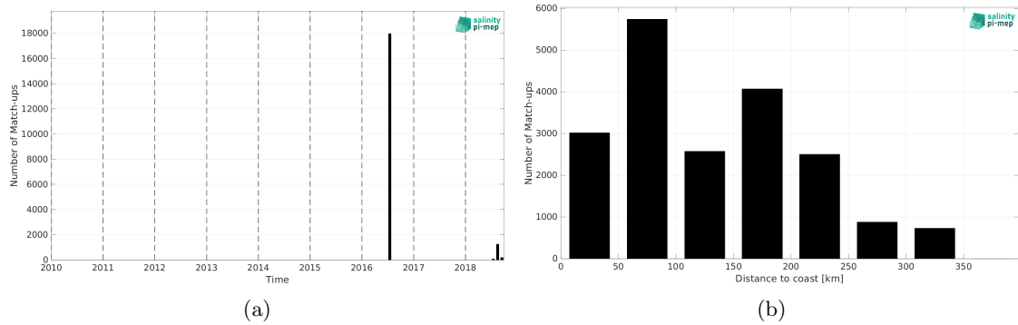
Figure 2: Number of match-ups between TSG (GOSUD-Research-vessel) and SMAP SSS L2 v6 (RSS) SSS as a function of time (a) and as function of the distance to coast (b) over the Arctic Ocean Pi-MEP region and for the full satellite product period.
