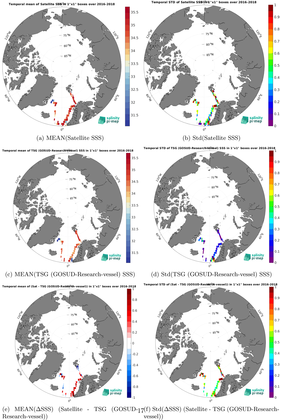
Figure 7: Temporal mean (left) and Std (right) of SSS from SMAP SSS L2 v6 (RSS) (top), TSG (GOSUD-Research-vessel) (middle), and of \Delta SSS (Satellite - TSG (GOSUD-Research-vessel)). Only match-up pairs are used to generate these maps.
