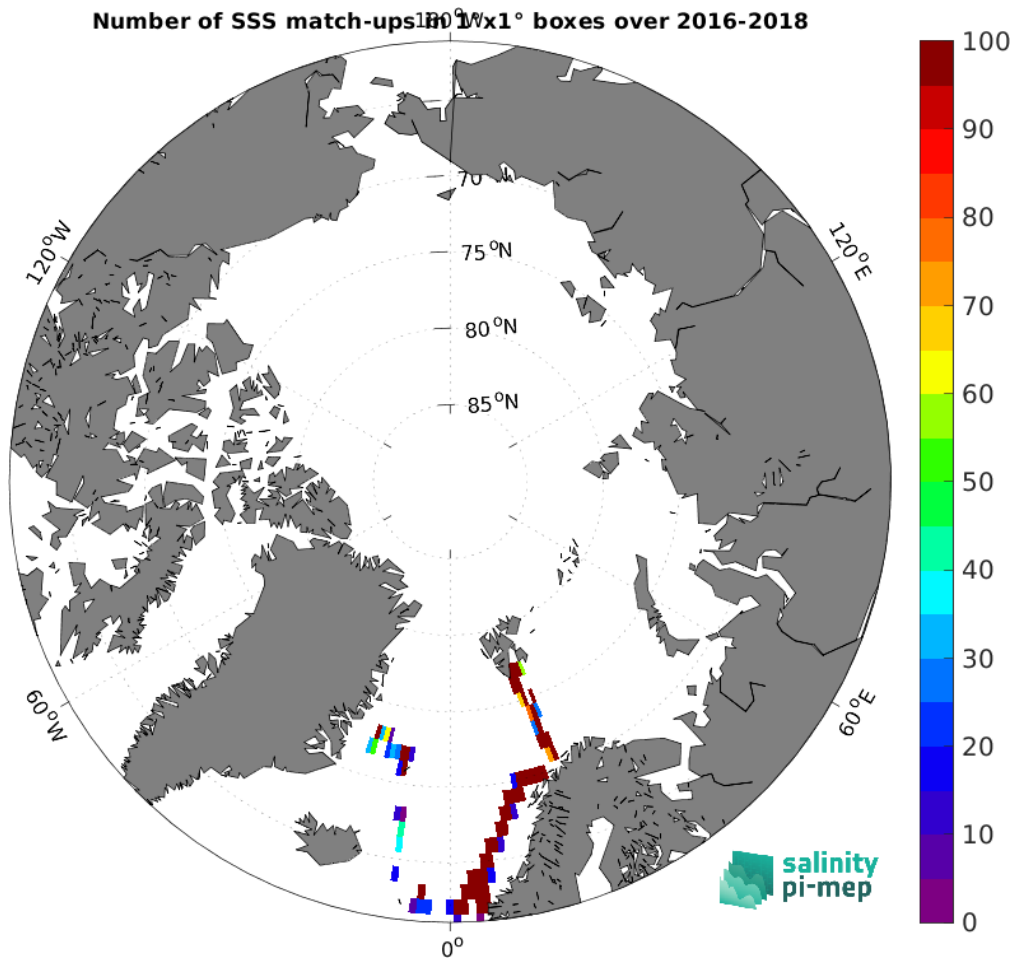
Figure 5: Number of SSS match-ups between TSG (GOSUD-Research-vessel) SSS and the SMAP SSS L2 v6 (RSS) SSS product for the Arctic Ocean Pi-MEP region over 1^{\circ} \times 1^{\circ} boxes and for the full satellite product period.
