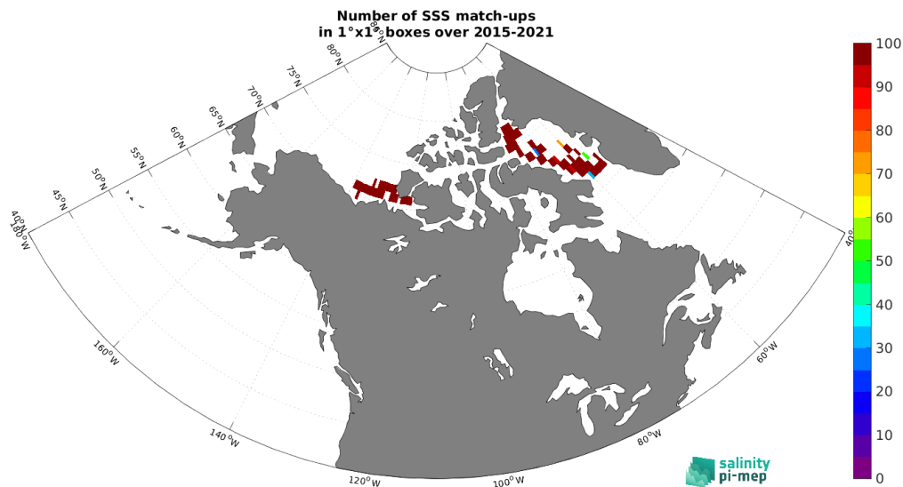
Figure 5: Number of SSS match-ups between TSG (Amundsen) SSS and the SMAP SSS L2 v6 (RSS) SSS product for the Arctic Ocean Pi-MEP region over 1^\circ \times 1^\circ boxes and for the full satellite product period.
