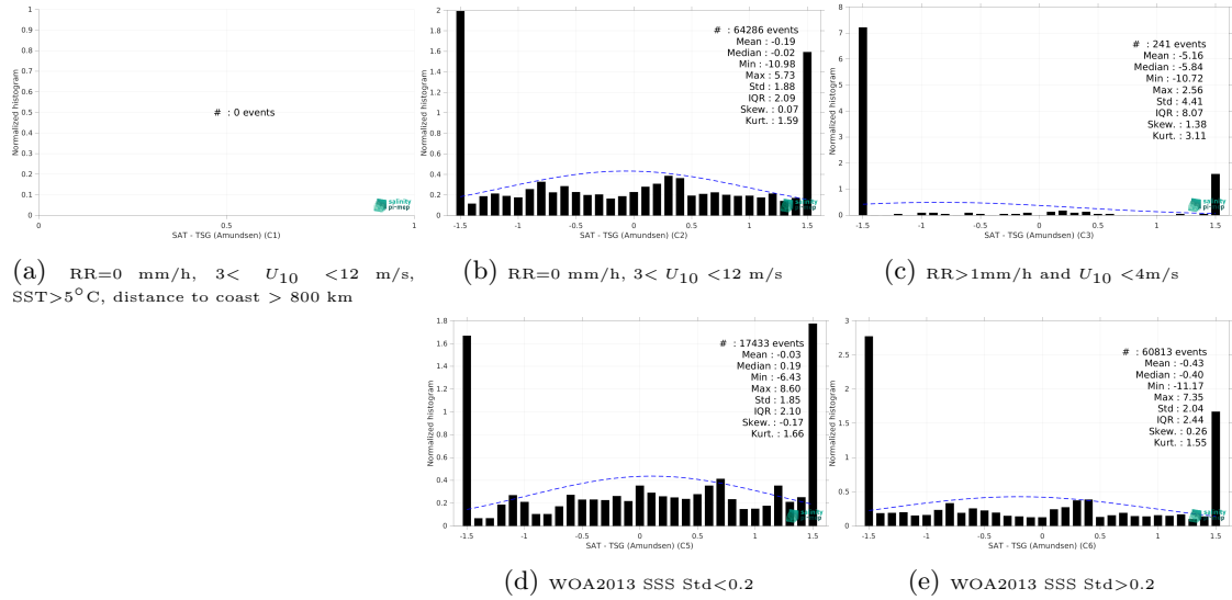
Figure 15: Normalized histogram of \Delta SSS (SMAP SSS L2 v6 (RSS) - TSG (Amundsen)) for 5 different subdatasets corresponding to: RR=0 mm/h, 3 < U_{10} < 12 m/s, SST > 5°C, distance to coast > 800 km (a), RR=0 mm/h, 3 < U_{10} < 12 m/s (b), RR > 1mm/h and U_{10} < 4 m/s (c), WOA2013 SSS Std < 0.2 (d), WOA2013 SSS Std > 0.2 (e).
