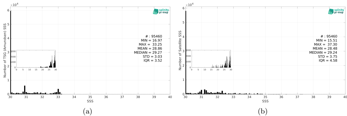
Figure 3: Histograms of SSS from TSG (Amundsen) (a) and SMAP SSS L2 v6 (RSS) (b) considering all match-up pairs per bins of 0.1 over the Arctic Ocean Pi-MEP region and for the full satellite product period.
