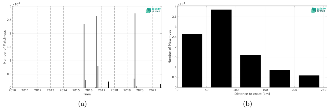
Figure 2: Number of match-ups between TSG (Amundsen) and SMAP SSS L2 v6 (RSS) SSS as a function of time (a) and as function of the distance to coast (b) over the Arctic Ocean Pi-MEP region and for the full satellite product period.
