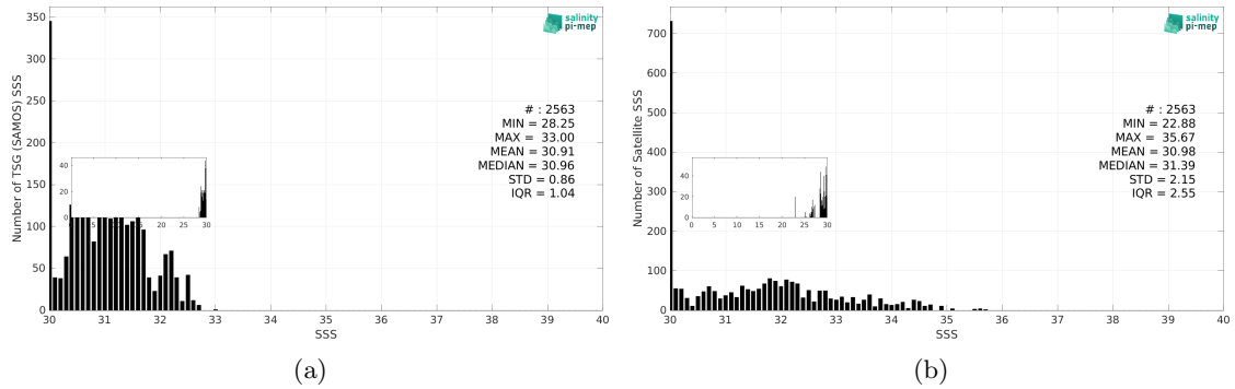
Figure 3: Histograms of SSS from TSG (SAMOS) (a) and SMAP SSS L2 v6 - 40 km (RSS) (b) considering all match-up pairs per bins of 0.1 over the Arctic Ocean Pi-MEP region and for the full satellite product period.
