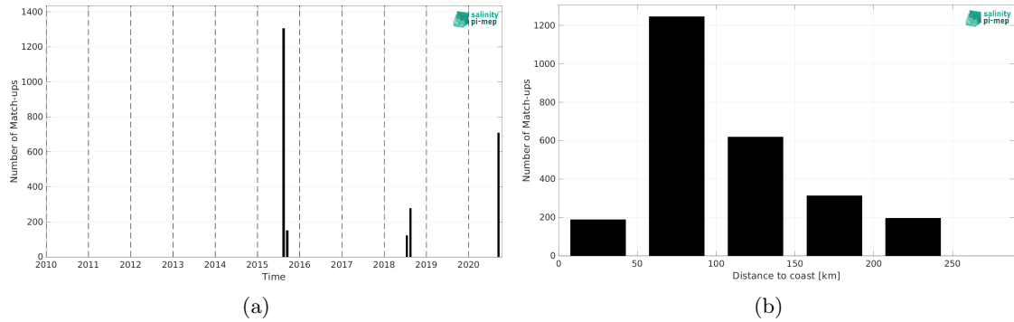
Figure 2: Number of match-ups between TSG (SAMOS) and SMAP SSS L2 v6 - 40 km (RSS) SSS as a function of time (a) and as function of the distance to coast (b) over the Arctic Ocean Pi-MEP region and for the full satellite product period.
