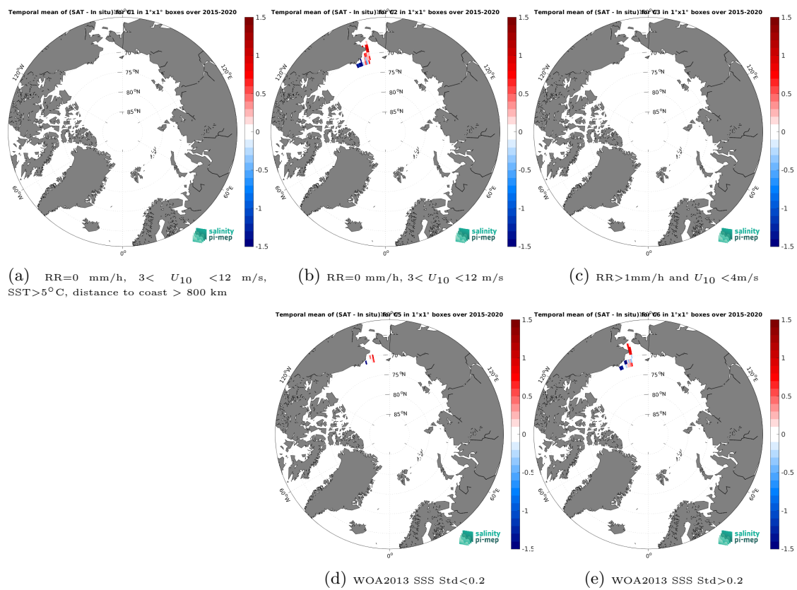
Figure 14: Temporal mean gridded over spatial boxes of size 1^\circ \times 1^\circ of \Delta\text{SSS} (SMAP SSS L2 v6 - 40 km (RSS) - TSG (SAMOS)) for 5 different subdatasets corresponding to:RR=0 mm/h, 3 < U_{10} < 12 m/s, SST>5°C, distance to coast > 800 km (a), RR=0 mm/h, 3 < U_{10} < 12 m/s (b), RR>1mm/h and U_{10} < 4 m/s (c), WOA2013 SSS Std<0.2 (d), WOA2013 SSS Std>0.2 (e).
