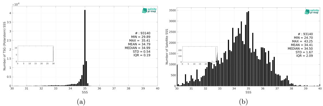
Figure 3: Histograms of SSS from TSG (Polarstern) (a) and SMAP SSS L2 v6 - 40 km (RSS) (b) considering all match-up pairs per bins of 0.1 over the Arctic Ocean Pi-MEP region and for the full satellite product period.
