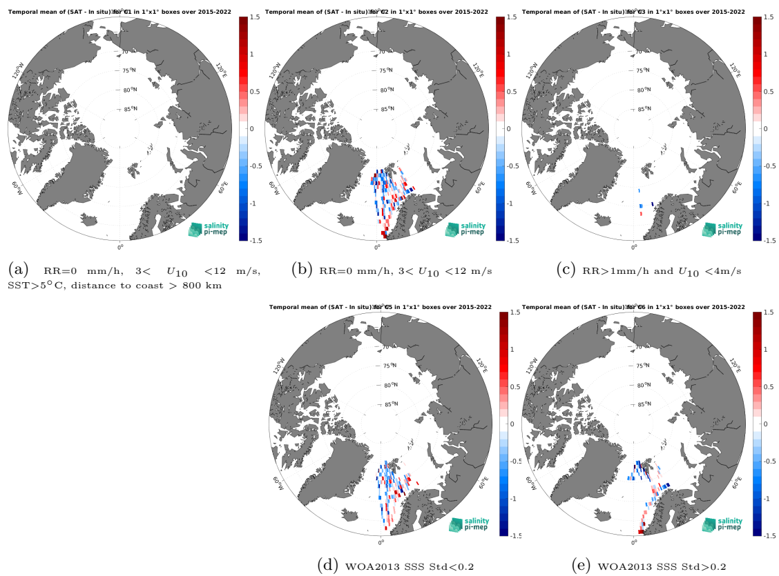
Figure 14: Temporal mean gridded over spatial boxes of size 1^\circ \times 1^\circ of \Delta SSS (SMAP SSS L2 v6 - 40 km (RSS) - TSG (Polarstern)) for 5 different subdatasets corresponding to: RR=0 mm/h, 3 < U_{10} < 12 m/s, SST > 5°C, distance to coast > 800 km (a), RR=0 mm/h, 3 < U_{10} < 12 m/s (b), RR > 1mm/h and U_{10} < 4 m/s (c), WOA2013 SSS Std < 0.2 (d), WOA2013 SSS Std > 0.2 (e).
