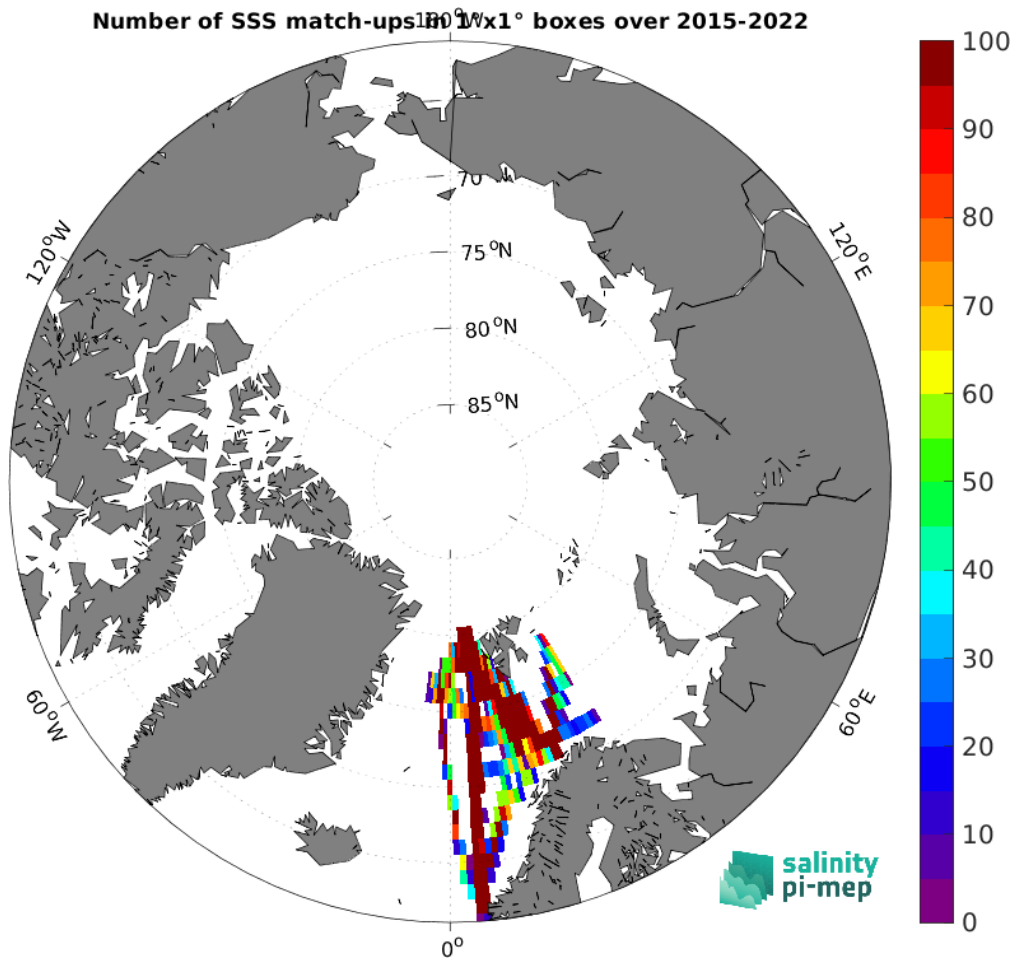
Figure 5: Number of SSS match-ups between TSG (Polarstern) SSS and the SMAP SSS L2 v6 - 40 km (RSS) SSS product for the Arctic Ocean Pi-MEP region over 1^\circ \times 1^\circ boxes and for the full satellite product period.
