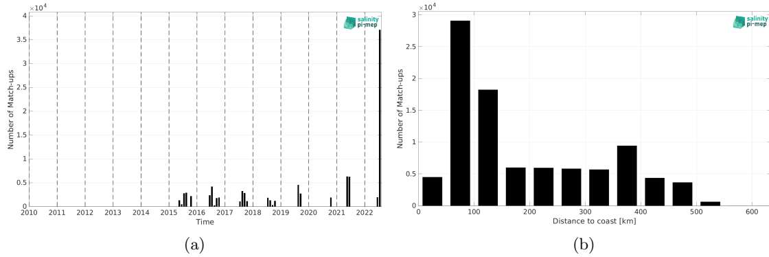
Figure 2: Number of match-ups between TSG (Polarstern) and SMAP SSS L2 v6 - 40 km (RSS) SSS as a function of time (a) and as function of the distance to coast (b) over the Arctic Ocean Pi-MEP region and for the full satellite product period.
