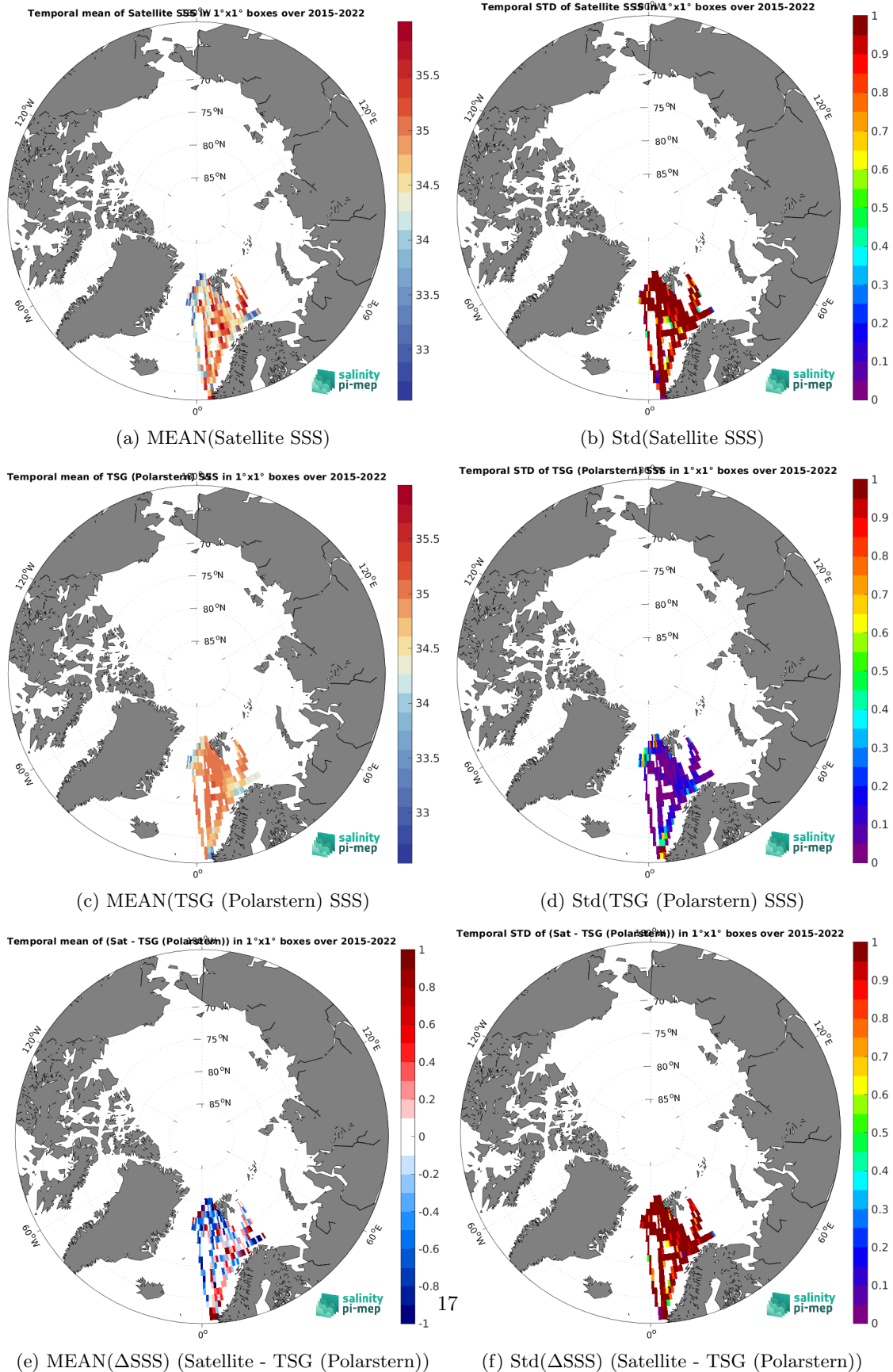
Figure 7: Temporal mean (left) and Std (right) of SSS from SMAP SSS L2 v6 - 40 km (RSS) (top), TSG (Polarstern) (middle), and of \Delta SSS (Satellite - TSG (Polarstern)). Only match-up pairs are used to generate these maps.
