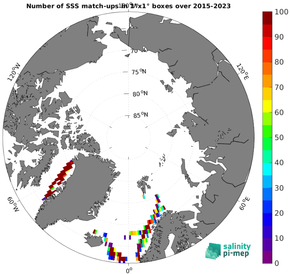
Figure 5: Number of SSS match-ups between TSG (LEGOS-DM) SSS and the SMAP SSS L2 v6 - 40 km (RSS) SSS product for the Arctic Ocean Pi-MEP region over 1^{\circ} \times 1^{\circ} boxes and for the full satellite product period.
