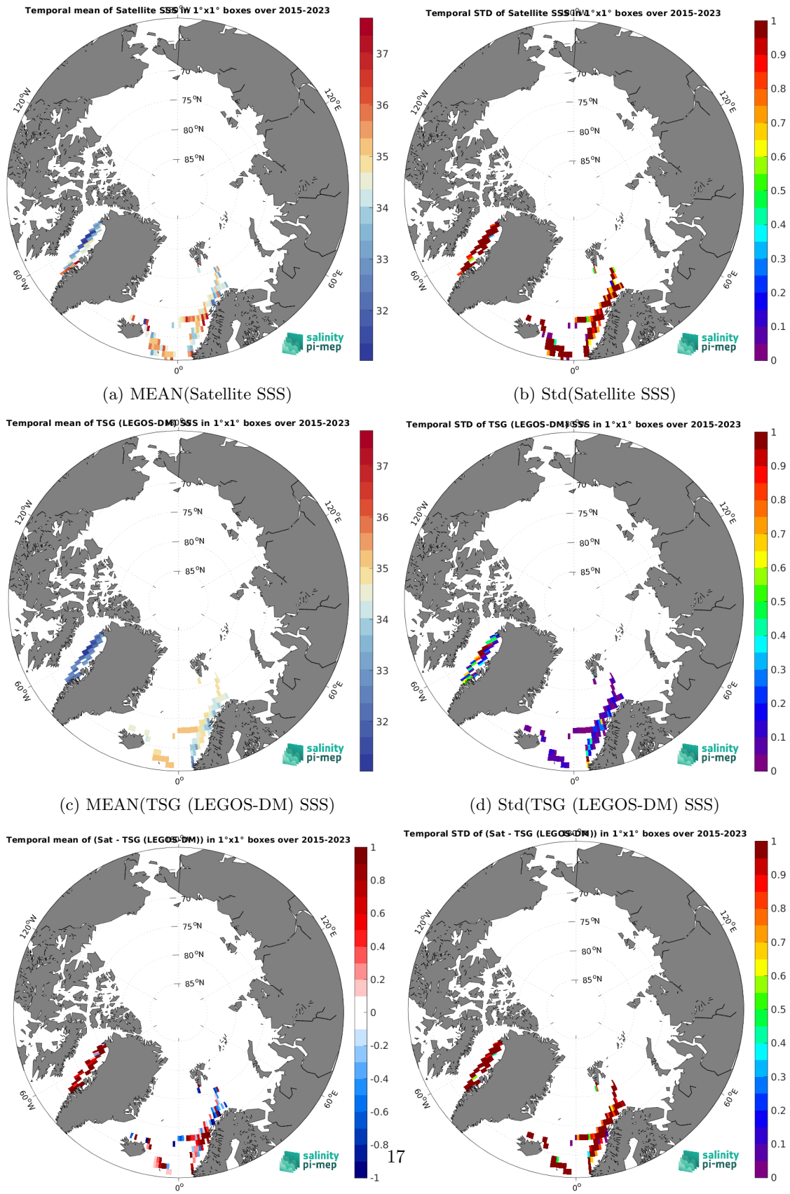
Figure 7: Temporal mean (left) and Std (right) of SSS from SMAP SSS L2 v6 - 40 km (RSS) (top), TSG (LEGOS-DM) (middle), and of \Delta SSS (Satellite - TSG (LEGOS-DM)). Only match-up pairs are used to generate these maps.
