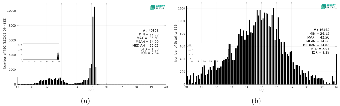
Figure 3: Histograms of SSS from TSG (LEGOS-DM) (a) and SMAP SSS L2 v6 - 40 km (RSS) (b) considering all match-up pairs per bins of 0.1 over the Arctic Ocean Pi-MEP region and for the full satellite product period.
