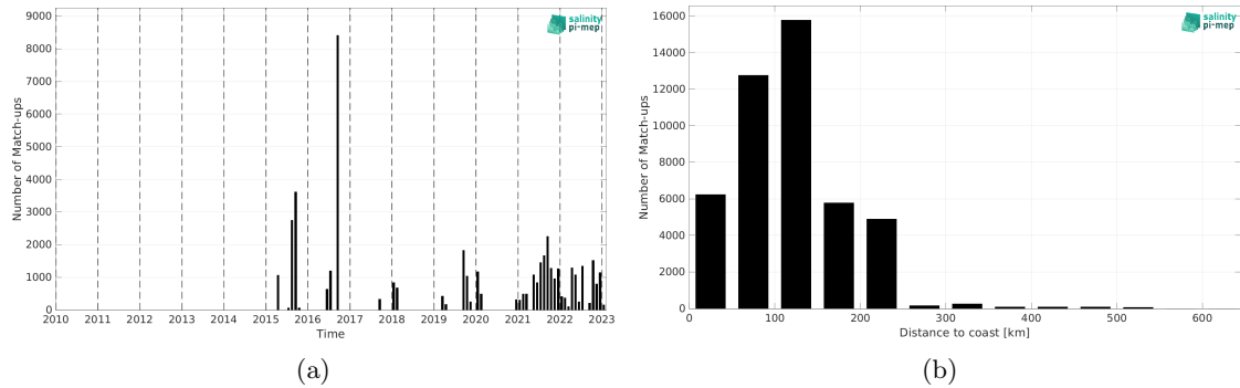
Figure 2: Number of match-ups between TSG (LEGOS-DM) and SMAP SSS L2 v6 - 40 km (RSS) SSS as a function of time (a) and as function of the distance to coast (b) over the Arctic Ocean Pi-MEP region and for the full satellite product period.
