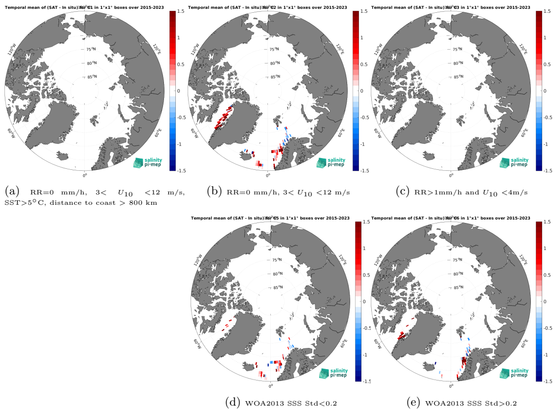
Figure 14: Temporal mean gridded over spatial boxes of size 1^\circ \times 1^\circ of \Delta SSS (SMAP SSS L2 v6 - 40 km (RSS) - TSG (LEGOS-DM)) for 5 different subdatasets corresponding to:RR=0 mm/h, 3 < U_{10} < 12 m/s, SST>5°C, distance to coast > 800 km (a), RR=0 mm/h, 3 < U_{10} < 12 m/s (b), RR>1mm/h and U_{10} < 4 m/s (c), WOA2013 SSS Std<0.2 (d), WOA2013 SSS Std>0.2 (e).
