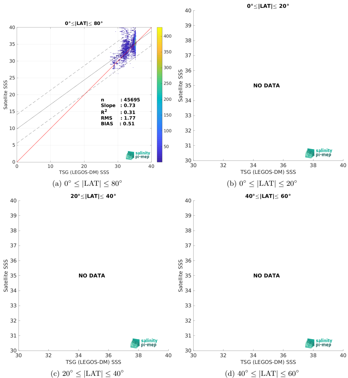
Figure 10: Contour maps of the concentration of SMAP SSS L2 v6 - 40 km (RSS) SSS (y-axis) versus TSG (LEGOS-DM) SSS (x-axis) at match-up pairs for different latitude bands. For each plot, the red line shows x=y . The black thin and dashed lines indicate a linear fit through the data cloud and the \pm 95\% confidence levels, respectively. The number match-up pairs n , the slope and R^2 coefficient of the linear fit, the root mean square (RMS) and the mean bias between satellite and in situ data are indicated for each latitude band in each plots.
