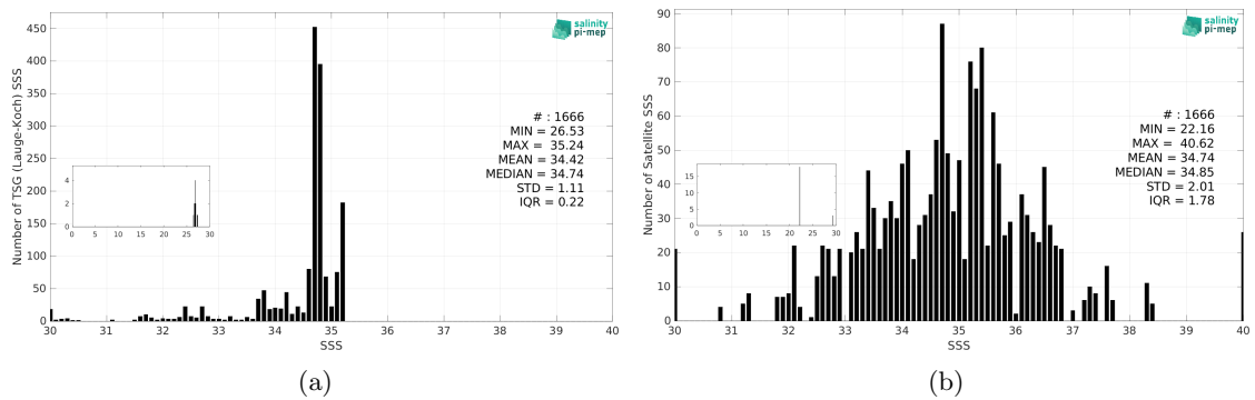
Figure 3: Histograms of SSS from TSG (Lauge-Koch) (a) and SMAP SSS L2 v6 - 40 km (RSS) (b) considering all match-up pairs per bins of 0.1 over the Arctic Ocean Pi-MEP region and for the full satellite product period.
