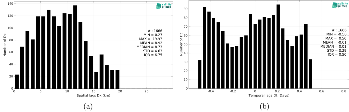
Figure 6: Histograms of the spatial (a) and temporal (b) lags between the location/time of the TSG (Lauge-Koch) measurement and the date of the corresponding SMAP SSS L2 v6 - 40 km (RSS) SSS pixel.
