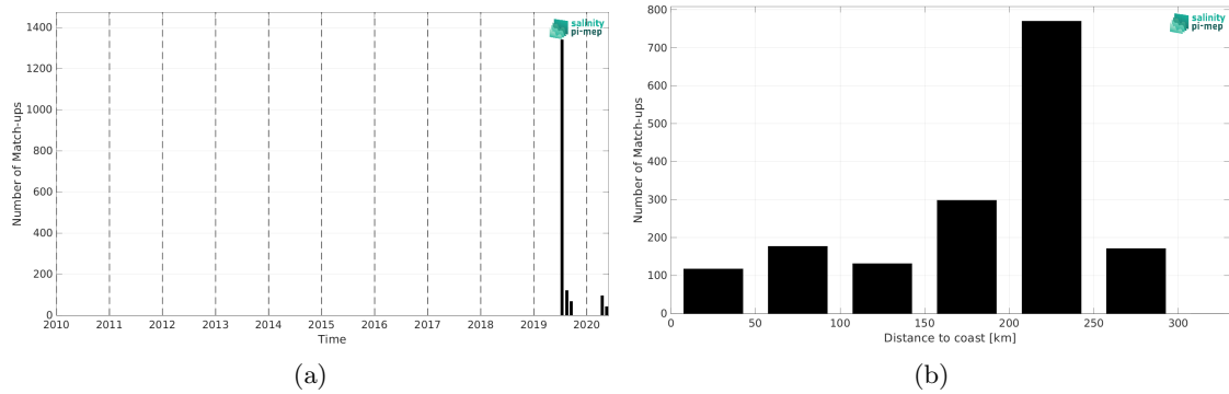
Figure 2: Number of match-ups between TSG (Lauge-Koch) and SMAP SSS L2 v6 - 40 km (RSS) SSS as a function of time (a) and as function of the distance to coast (b) over the Arctic Ocean Pi-MEP region and for the full satellite product period.
