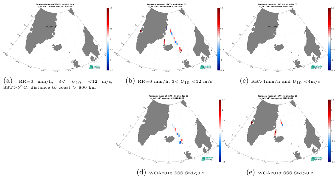
Figure 14: Temporal mean gridded over spatial boxes of size 1^\circ \times 1^\circ of \Delta SSS (SMAP SSS L2 v6 - 40 km (RSS) - TSG (Lauge-Koch)) for 5 different subdatasets corresponding to:RR=0 mm/h, 3 < U_{10} < 12 m/s, SST > 5^\circ\text{C} , distance to coast > 800 km (a), RR=0 mm/h, 3 < U_{10} < 12 m/s (b), RR > 1 mm/h and U_{10} < 4 m/s (c), WOA2013 SSS Std < 0.2 (d), WOA2013 SSS Std > 0.2 (e).
