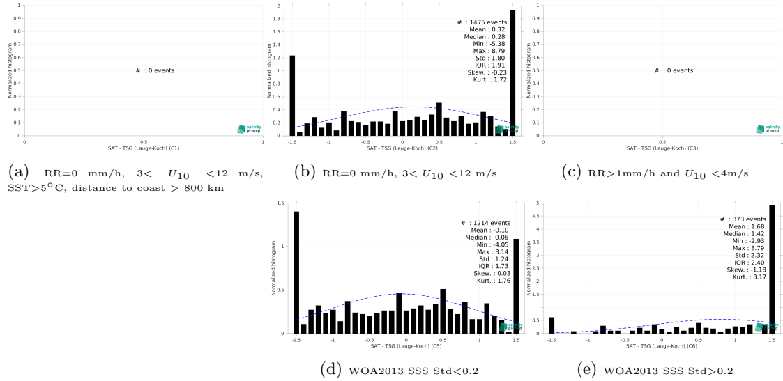
Figure 15: Normalized histogram of \Delta SSS (SMAP SSS L2 v6 - 40 km (RSS) - TSG (Lauge-Koch)) for 5 different subdatasets corresponding to: RR=0 mm/h, 3 < U_{10} < 12 m/s, SST > 5°C, distance to coast > 800 km (a), RR=0 mm/h, 3 < U_{10} < 12 m/s (b), RR > 1mm/h and U_{10} < 4 m/s (c), WOA2013 SSS Std < 0.2 (d), WOA2013 SSS Std > 0.2 (e).
