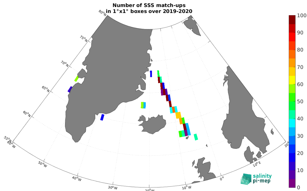
Figure 5: Number of SSS match-ups between TSG (Lauge-Koch) SSS and the SMAP SSS L2 v6 - 40 km (RSS) SSS product for the Arctic Ocean Pi-MEP region over 1^\circ \times 1^\circ boxes and for the full satellite product period.
