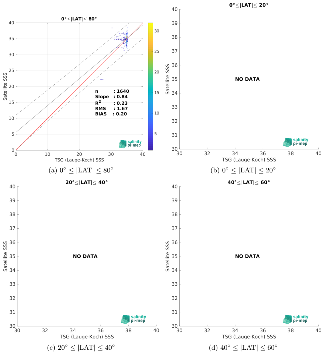
Figure 10: Contour maps of the concentration of SMAP SSS L2 v6 - 40 km (RSS) SSS (y-axis) versus TSG (Lauge-Koch) SSS (x-axis) at match-up pairs for different latitude bands. For each plot, the red line shows x=y . The black thin and dashed lines indicate a linear fit through the data cloud and the \pm 95\% confidence levels, respectively. The number match-up pairs n , the slope and R^2 coefficient of the linear fit, the root mean square (RMS) and the mean bias between satellite and in situ data are indicated for each latitude band in each plots.
