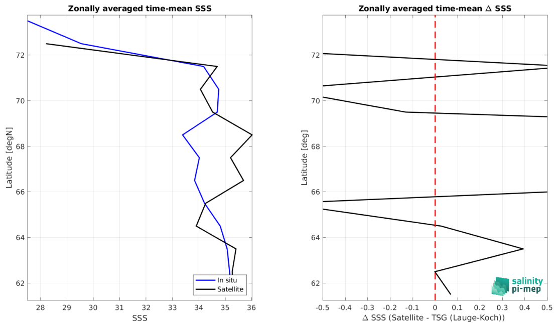
Figure 9: Left panel: Zonal mean SSS from SMAP SSS L2 v6 - 40 km (RSS) satellite product (black) and from TSG (Lauge-Koch) (blue). Right panel: Zonal mean of \Delta SSS (Satellite - TSG (Lauge-Koch)) for all the collected Pi-MEP match-up pairs estimated over the full satellite product period.
