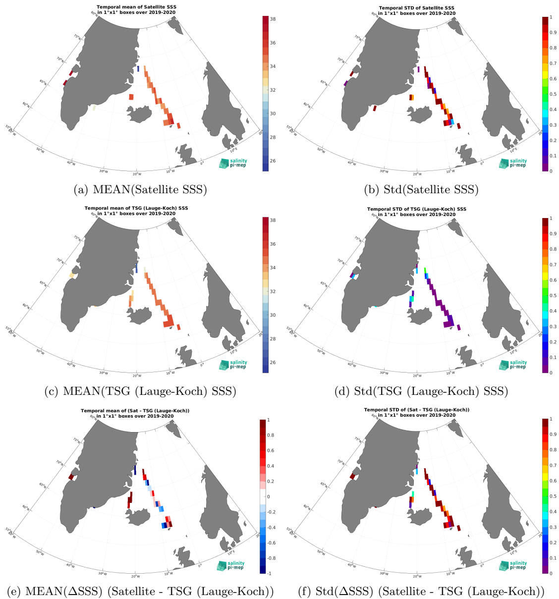
Figure 7: Temporal mean (left) and Std (right) of SSS from SMAP SSS L2 v6 - 40 km (RSS) (top), TSG (Lauge-Koch) (middle), and of \Delta SSS (Satellite - TSG (Lauge-Koch)). Only match-up pairs are used to generate these maps.
