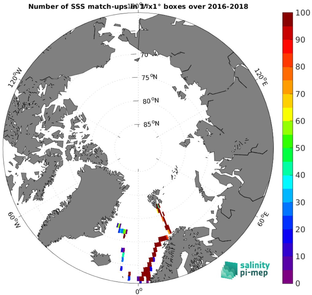
Figure 5: Number of SSS match-ups between TSG (GOSUD-Research-vessel) SSS and the SMAP SSS L2 v6 - 40 km (RSS) SSS product for the Arctic Ocean Pi-MEP region over 1^{\circ} \times 1^{\circ} boxes and for the full satellite product period.
