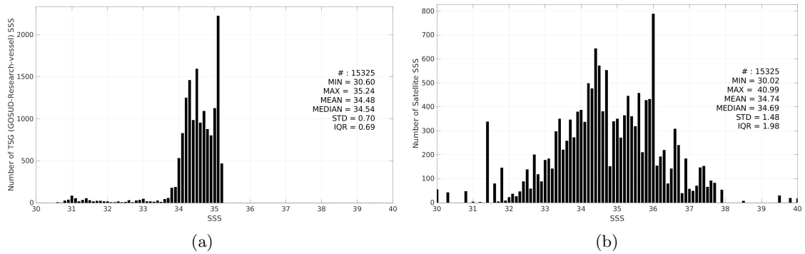
Figure 3: Histograms of SSS from TSG (GOSUD-Research-vessel) (a) and SMAP SSS L2 v6 - 40 km (RSS) (b) considering all match-up pairs per bins of 0.1 over the Arctic Ocean Pi-MEP region and for the full satellite product period.
