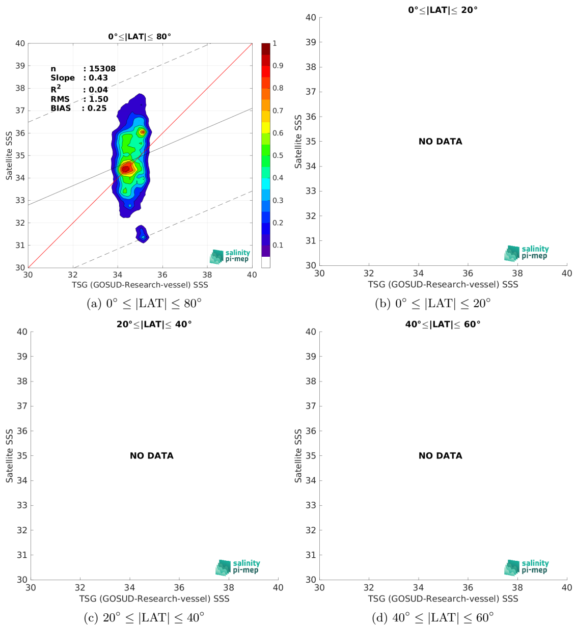
Figure 10: Contour maps of the concentration of SMAP SSS L2 v6 - 40 km (RSS) SSS (y-axis) versus TSG (GOSUD-Research-vessel) SSS (x-axis) at match-up pairs for different latitude bands. For each plot, the red line shows x=y . The black thin and dashed lines indicate a linear fit through the data cloud and the \pm 95\% confidence levels, respectively. The number match-up pairs n , the slope and R^2 coefficient of the linear fit, the root mean square (RMS) and the mean bias between satellite and in situ data are indicated for each latitude band in each plots.
