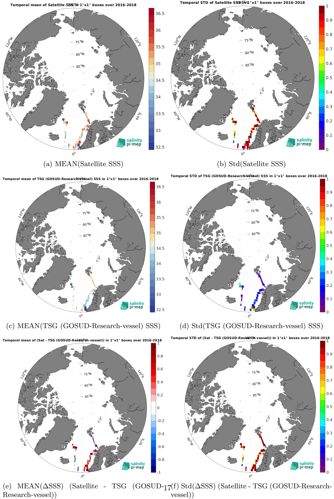
Figure 7: Temporal mean (left) and Std (right) of SSS from SMAP SSS L2 v6 - 40 km (RSS) (top), TSG (GOSUD-Research-vessel) (middle), and of \Delta SSS (Satellite - TSG (GOSUD-Research-vessel)). Only match-up pairs are used to generate these maps.
