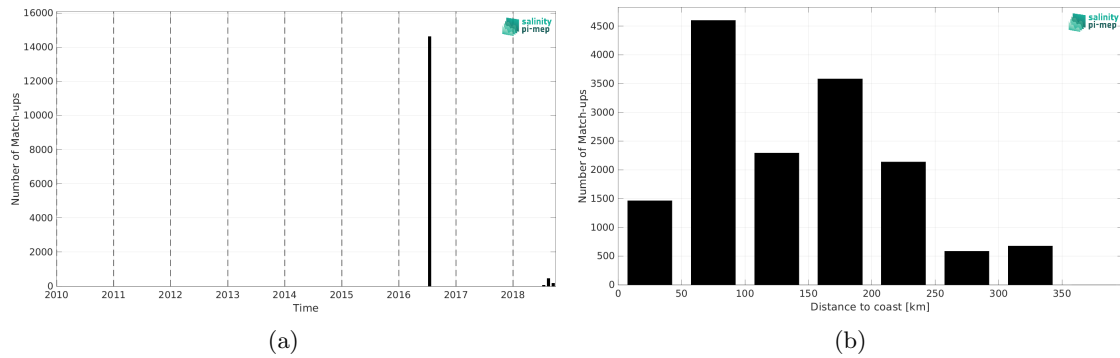
Figure 2: Number of match-ups between TSG (GOSUD-Research-vessel) and SMAP SSS L2 v6 - 40 km (RSS) SSS as a function of time (a) and as function of the distance to coast (b) over the Arctic Ocean Pi-MEP region and for the full satellite product period.
