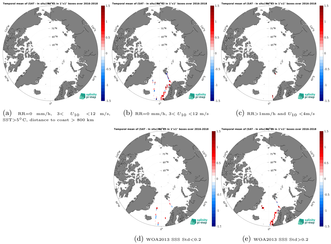
Figure 14: Temporal mean gridded over spatial boxes of size 1^\circ \times 1^\circ of \Delta SSS (SMAP SSS L2 v6 - 40 km (RSS) - TSG (GOSUD-Research-vessel)) for 5 different subdatasets corresponding to: RR=0 mm/h, 3 < U_{10} < 12 m/s, SST > 5°C, distance to coast > 800 km (a), RR=0 mm/h, 3 < U_{10} < 12 m/s (b), RR > 1mm/h and U_{10} < 4 m/s (c), WOA2013 SSS Std < 0.2 (d), WOA2013 SSS Std > 0.2 (e).
