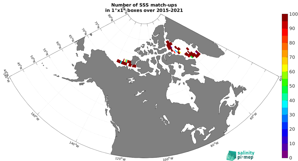
Figure 5: Number of SSS match-ups between TSG (Amundsen) SSS and the SMAP SSS L2 v6 - 40 km (RSS) SSS product for the Arctic Ocean Pi-MEP region over 1^\circ \times 1^\circ boxes and for the full satellite product period.
