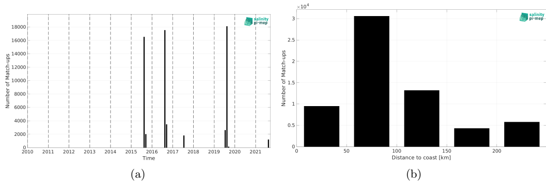
Figure 2: Number of match-ups between TSG (Amundsen) and SMAP SSS L2 v6 - 40 km (RSS) SSS as a function of time (a) and as function of the distance to coast (b) over the Arctic Ocean Pi-MEP region and for the full satellite product period.
