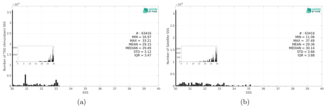
Figure 3: Histograms of SSS from TSG (Amundsen) (a) and SMAP SSS L2 v6 - 40 km (RSS) (b) considering all match-up pairs per bins of 0.1 over the Arctic Ocean Pi-MEP region and for the full satellite product period.
