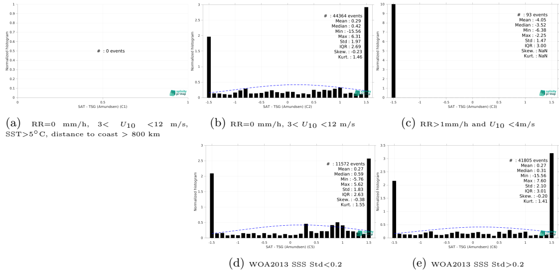
Figure 15: Normalized histogram of \Delta SSS (SMAP SSS L2 v6 - 40 km (RSS) - TSG (Amundsen)) for 5 different subdatasets corresponding to: RR=0 mm/h, 3 < U_{10} < 12 m/s, SST > 5°C, distance to coast > 800 km (a), RR=0 mm/h, 3 < U_{10} < 12 m/s (b), RR > 1mm/h and U_{10} < 4 m/s (c), WOA2013 SSS Std < 0.2 (d), WOA2013 SSS Std > 0.2 (e).
