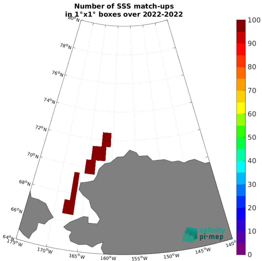
Figure 5: Number of SSS match-ups between SASSIE SSS and the SMAP SSS L2 v6 - 40 km (RSS) SSS product for the Arctic Ocean Pi-MEP region over 1^\circ \times 1^\circ boxes and for the full satellite product period.
