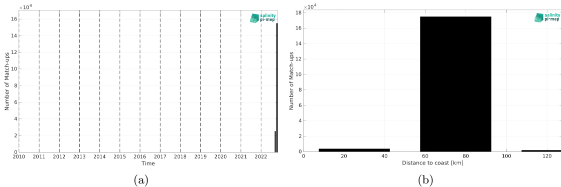
Figure 2: Number of match-ups between SASSIE and SMAP SSS L2 v6 - 40 km (RSS) SSS as a function of time (a) and as function of the distance to coast (b) over the Arctic Ocean Pi-MEP region and for the full satellite product period.
