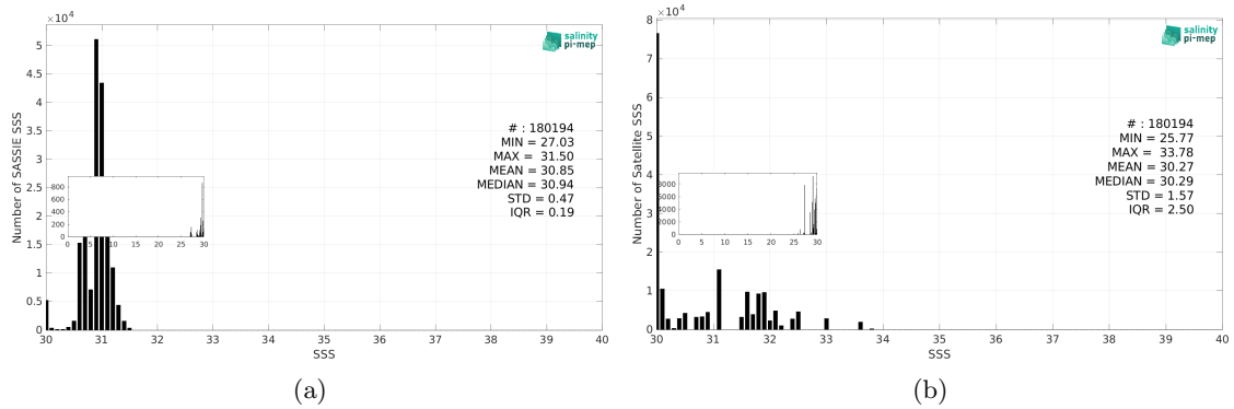
Figure 3: Histograms of SSS from SASSIE (a) and SMAP SSS L2 v6 - 40 km (RSS) (b) considering all match-up pairs per bins of 0.1 over the Arctic Ocean Pi-MEP region and for the full satellite product period.
