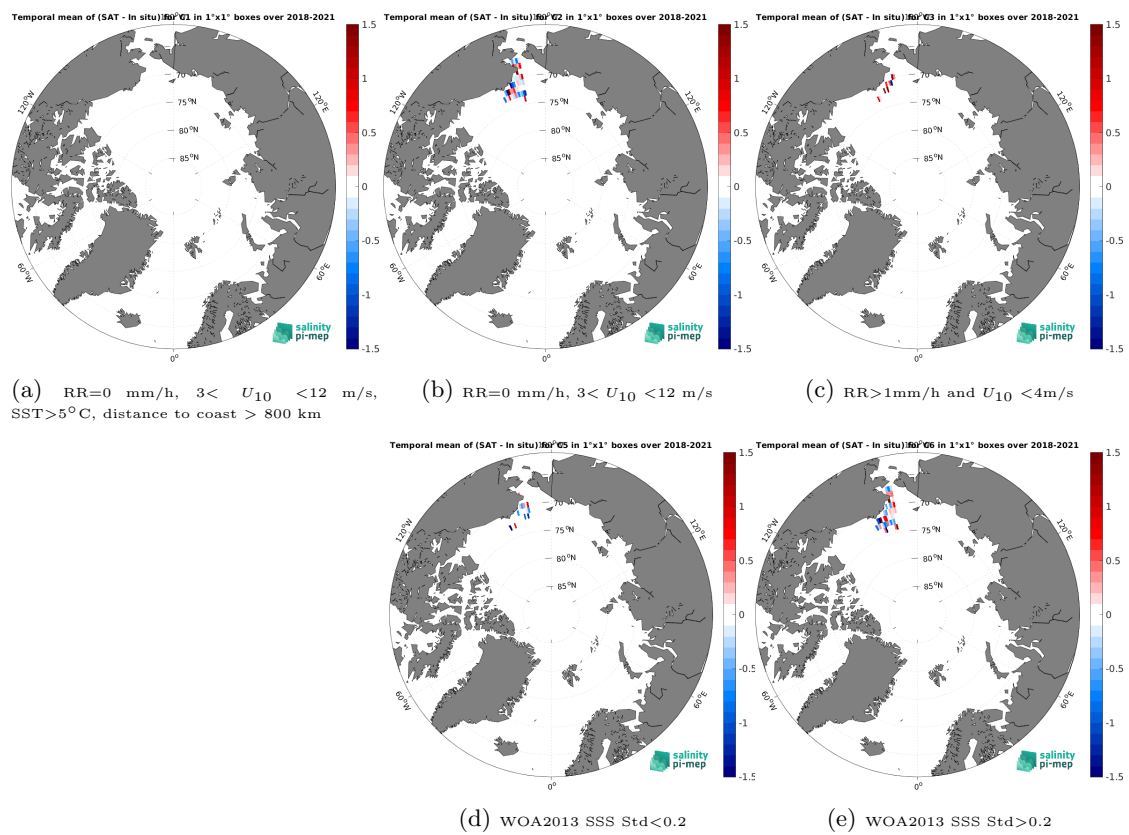
Figure 14: Temporal mean gridded over spatial boxes of size 1^\circ \times 1^\circ of \Delta SSS (SMAP SSS L2 v6 - 40 km (RSS) - Sailability) for 5 different subdatasets corresponding to:RR=0 mm/h, 3 < U_{10} < 12 m/s, SST>5°C, distance to coast > 800 km (a), RR=0 mm/h, 3 < U_{10} < 12 m/s (b), RR>1mm/h and U_{10} < 4 m/s (c), WOA2013 SSS Std<0.2 (d), WOA2013 SSS Std>0.2 (e).
