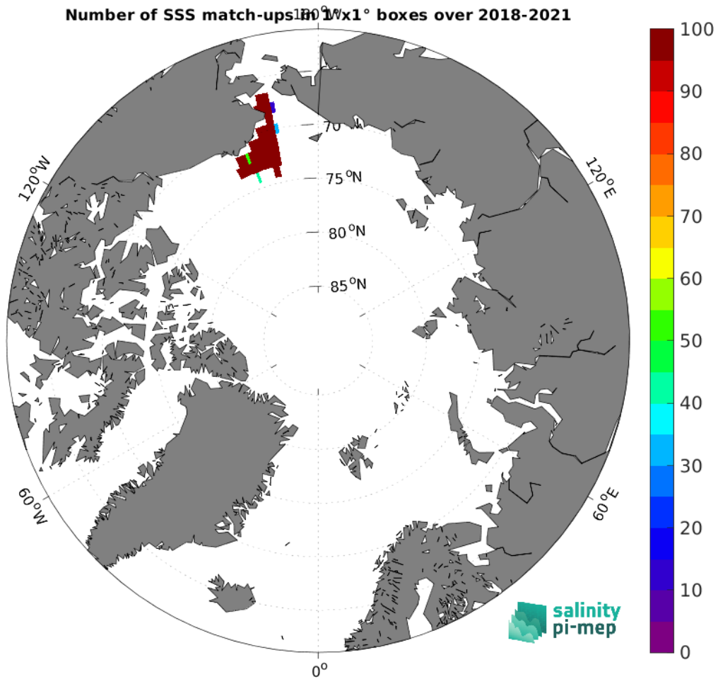
Figure 5: Number of SSS match-ups between Sairdrone SSS and the SMAP SSS L2 v6 - 40 km (RSS) SSS product for the Arctic Ocean Pi-MEP region over 1^\circ \times 1^\circ boxes and for the full satellite product period.
