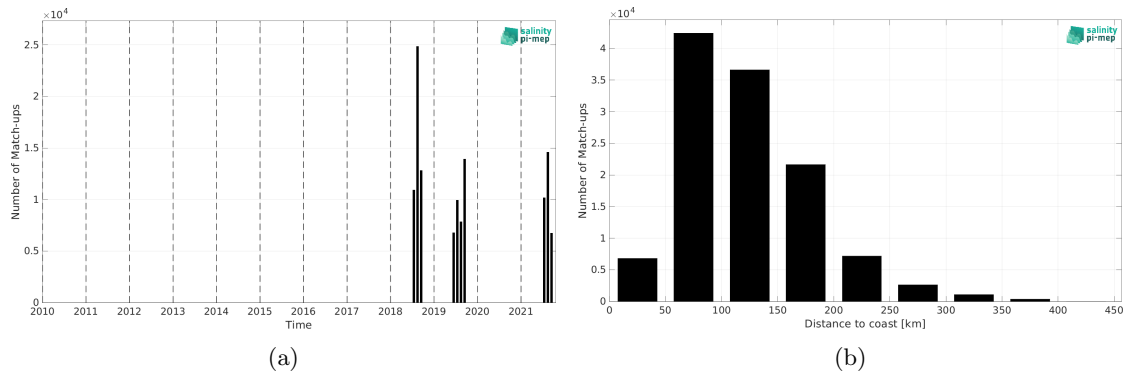
Figure 2: Number of match-ups between Sairdrone and SMAP SSS L2 v6 - 40 km (RSS) SSS as a function of time (a) and as function of the distance to coast (b) over the Arctic Ocean Pi-MEP region and for the full satellite product period.
