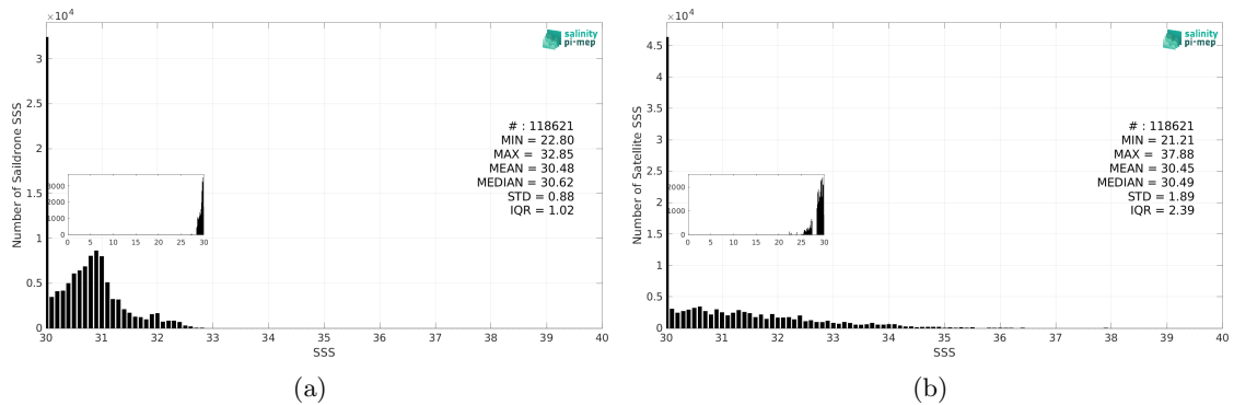
Figure 3: Histograms of SSS from Sairdrone (a) and SMAP SSS L2 v6 - 40 km (RSS) (b) considering all match-up pairs per bins of 0.1 over the Arctic Ocean Pi-MEP region and for the full satellite product period.
