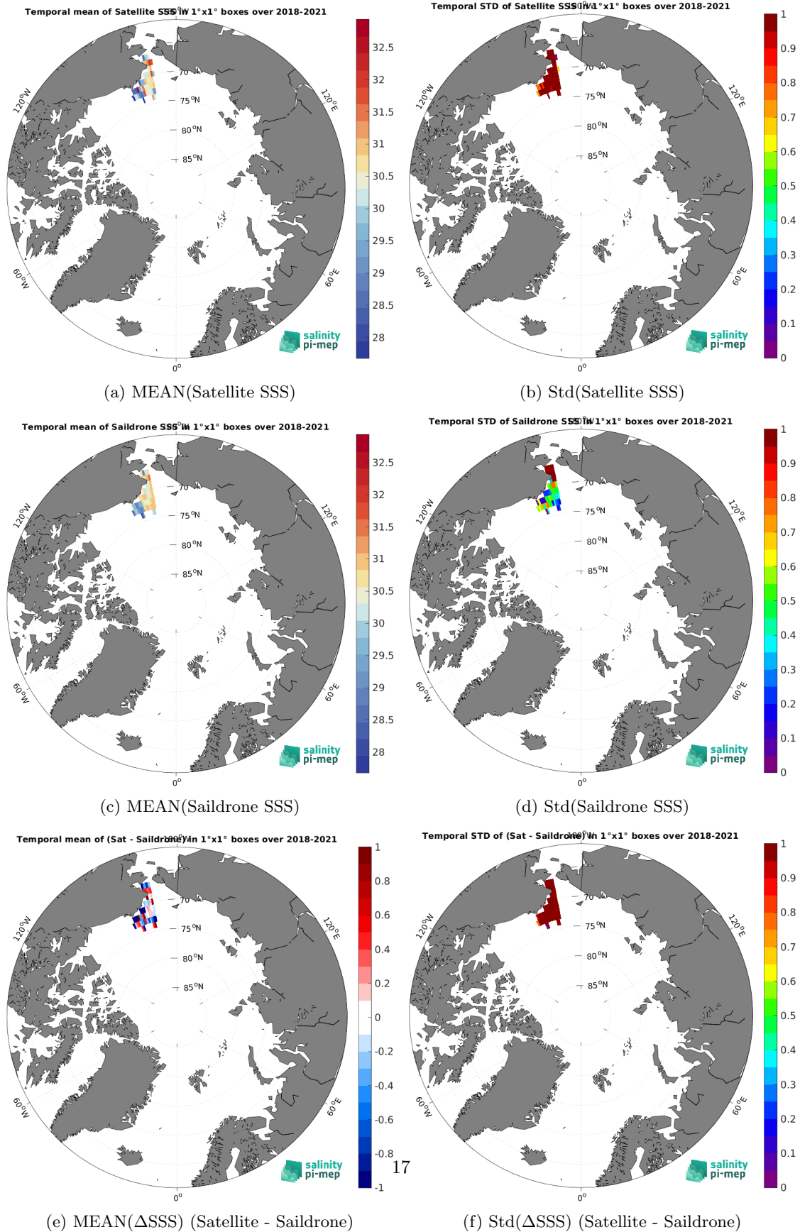
Figure 7: Temporal mean (left) and Std (right) of SSS from SMAP SSS L2 v6 - 40 km (RSS) (top), Saildrone (middle), and of \Delta SSS (Satellite - Saildrone). Only match-up pairs are used to generate these maps.
