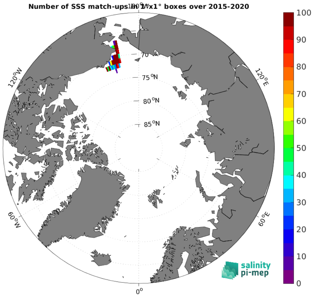
Figure 4: Number of SSS match-ups between TSG (SAMOS) SSS and the SMAP SSS L2 v5 (RSS) SSS product for the Arctic Ocean Pi-MEP region over 1^\circ \times 1^\circ boxes and for the full satellite product period.
