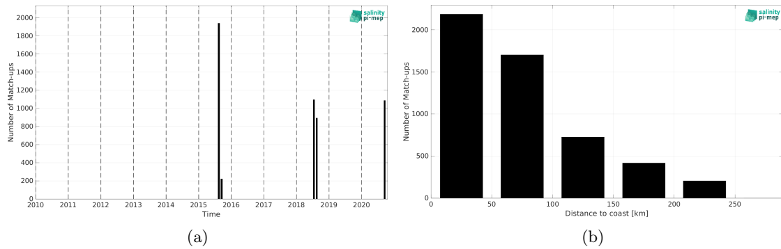
Figure 1: Number of match-ups between TSG (SAMOS) and SMAP SSS L2 v5 (RSS) SSS as a function of time (a) and as function of the distance to coast (b) over the Arctic Ocean Pi-MEP region and for the full satellite product period.
