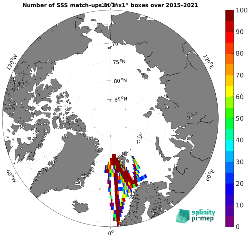
Figure 4: Number of SSS match-ups between TSG (Polarstern) SSS and the SMAP SSS L2 v5 (RSS) SSS product for the Arctic Ocean Pi-MEP region over 1^\circ \times 1^\circ boxes and for the full satellite product period.
