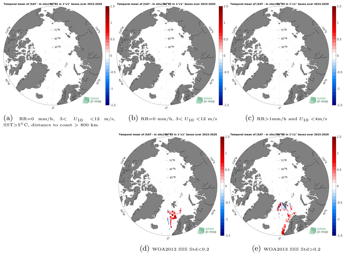
Figure 12: Temporal mean gridded over spatial boxes of size 1^{\circ}\times 1^{\circ} of \Delta\text{SSS} (SMAP SSS L2 v5 (RSS) - TSG (Polarstern)) for 5 different subdatasets corresponding to:RR=0 mm/h, 3 < U_{10} < 12 m/s, SST >5^{\circ}\text{C} , distance to coast > 800 km (a), RR=0 mm/h, 3 < U_{10} < 12 m/s (b), RR >1 mm/h and U_{10} < 4 m/s (c), WOA2013 SSS Std <0.2 (d), WOA2013 SSS Std >0.2 (e).
