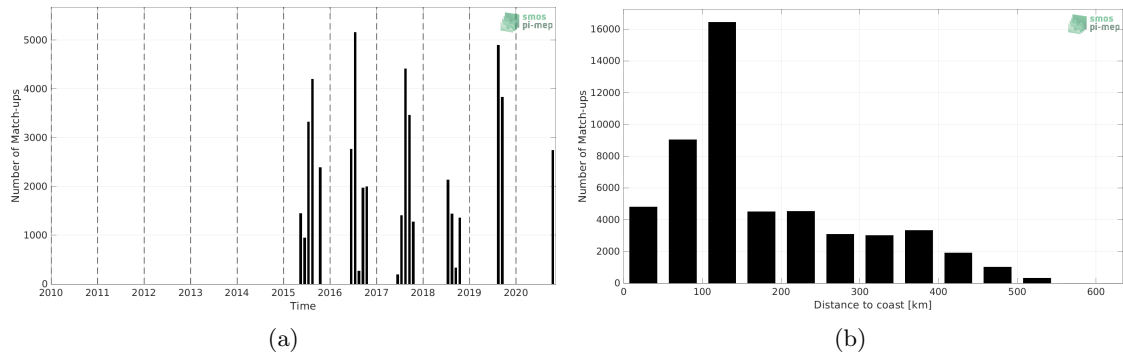
Figure 1: Number of match-ups between TSG (Polarstern) and SMAP SSS L2 v5 (RSS) SSS as a function of time (a) and as function of the distance to coast (b) over the Arctic Ocean Pi-MEP region and for the full satellite product period.
