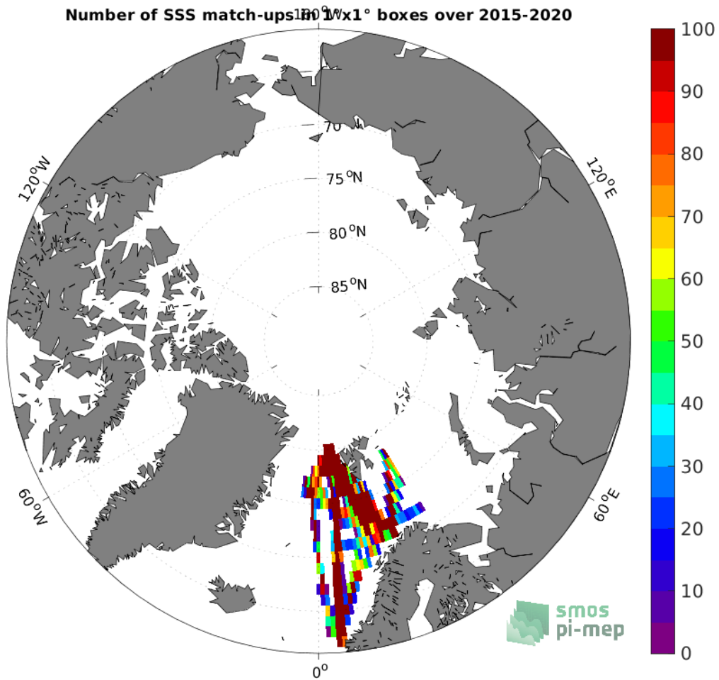
Figure 4: Number of SSS match-ups between TSG (Polarstern) SSS and the SMAP SSS L2 v5 (RSS) SSS product for the Arctic Ocean Pi-MEP region over 1^{\circ} \times 1^{\circ} boxes and for the full satellite product period.
