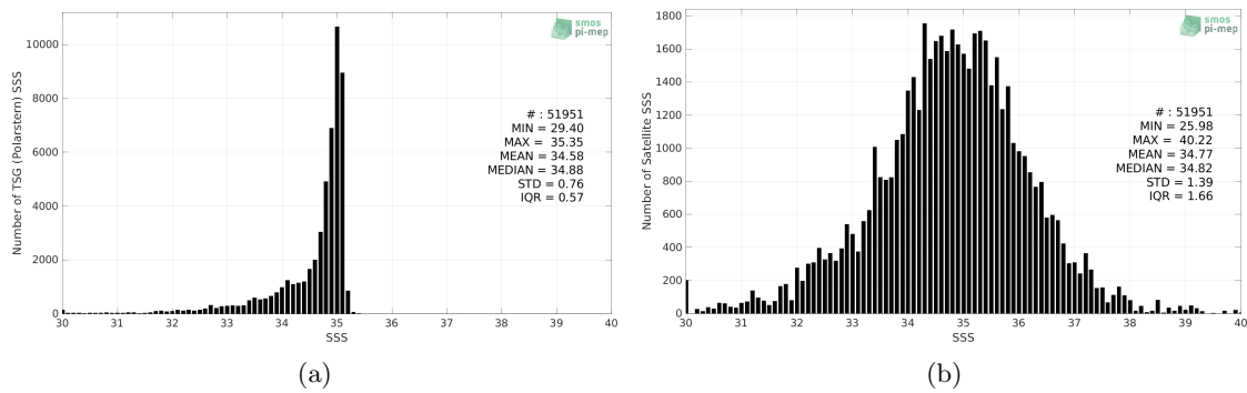
Figure 2: Histograms of SSS from TSG (Polarstern) (a) and SMAP SSS L2 v5 (RSS) (b) considering all match-up pairs per bins of 0.1 over the Arctic Ocean Pi-MEP region and for the full satellite product period.
