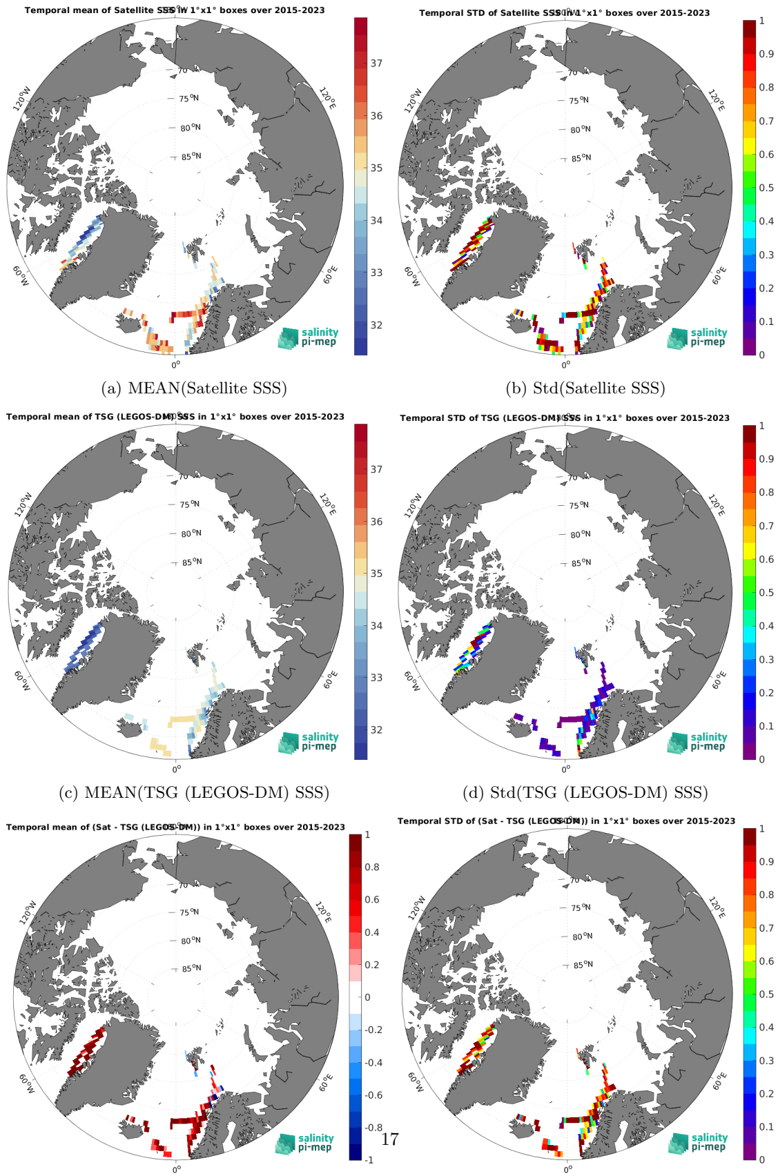
Figure 6: Temporal mean (left) and Std (right) of SSS from SMAP SSS L2 v5 (RSS) (top), TSG (LEGOS-DM) (middle), and of \Delta SSS (Satellite - TSG (LEGOS-DM)). Only match-up pairs are used to generate these maps.
