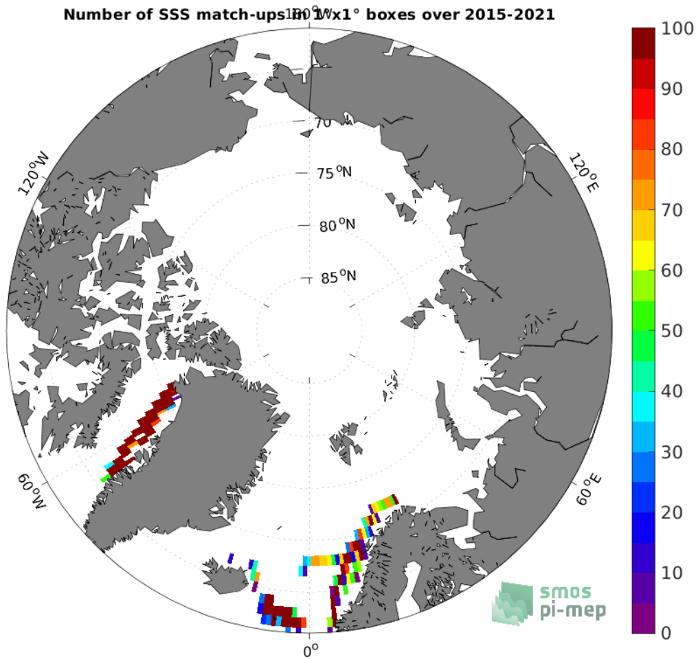
Figure 4: Number of SSS match-ups between TSG (LEGOS-DM) SSS and the SMAP SSS L2 v5 (RSS) SSS product for the Arctic Ocean Pi-MEP region over 1^{\circ} \times 1^{\circ} boxes and for the full satellite product period.
