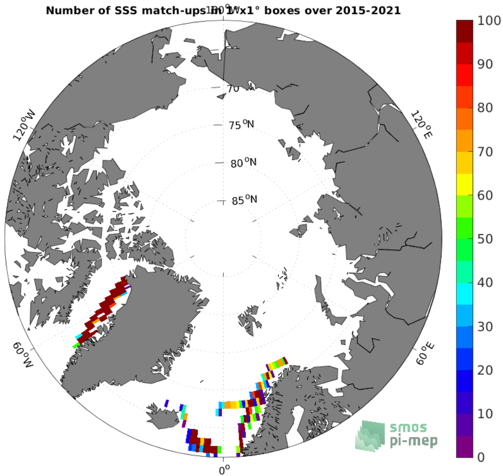
Figure 4: Number of SSS match-ups between TSG (LEGOS-DM) SSS and the SMAP SSS L2 v5 (RSS) SSS product for the Arctic Ocean Pi-MEP region over 1^\circ \times 1^\circ boxes and for the full satellite product period.
