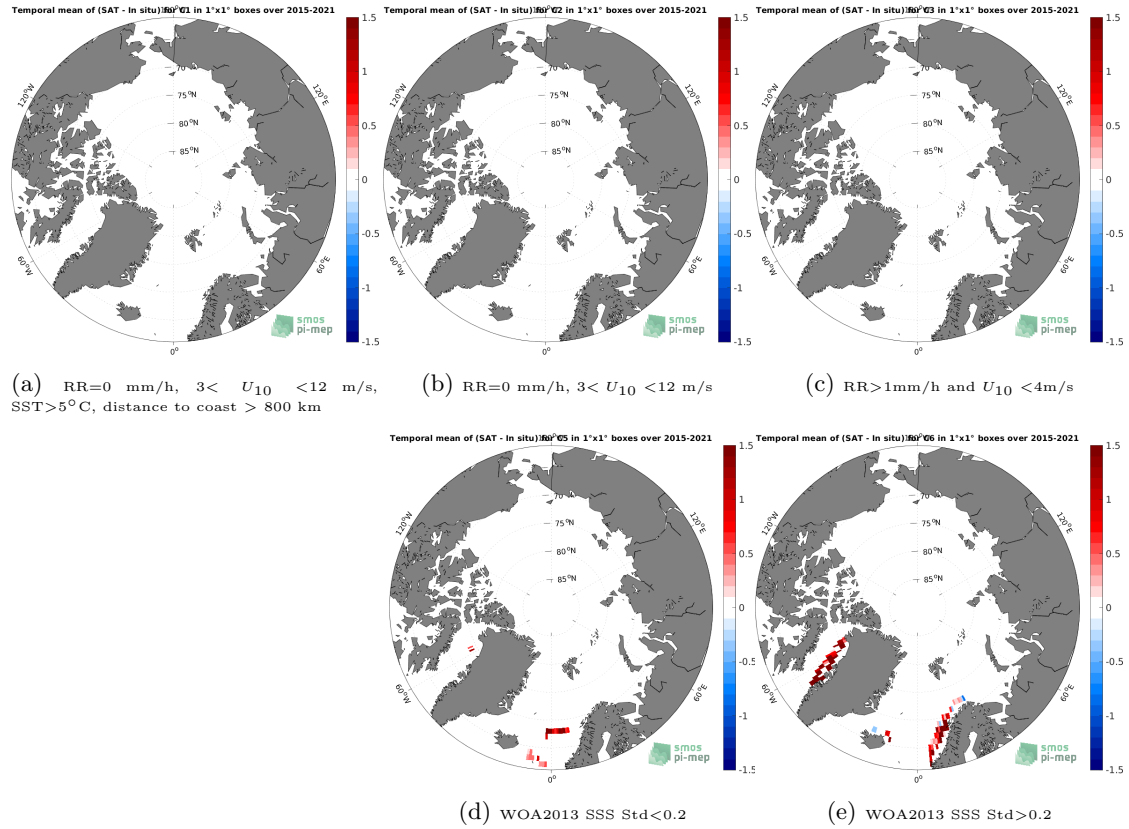
Figure 12: Temporal mean gridded over spatial boxes of size 1^{\circ}\times 1^{\circ} of \Delta\text{SSS} (SMAP SSS L2 v5 (RSS) - TSG (LEGOS-DM)) for 5 different subdatasets corresponding to:RR=0 mm/h, 3 < U_{10} < 12 m/s, SST > 5^{\circ}\text{C} , distance to coast > 800 km (a), RR=0 mm/h, 3 < U_{10} < 12 m/s (b), RR > 1 mm/h and U_{10} < 4 m/s (c), WOA2013 SSS Std < 0.2 (d), WOA2013 SSS Std > 0.2 (e).
