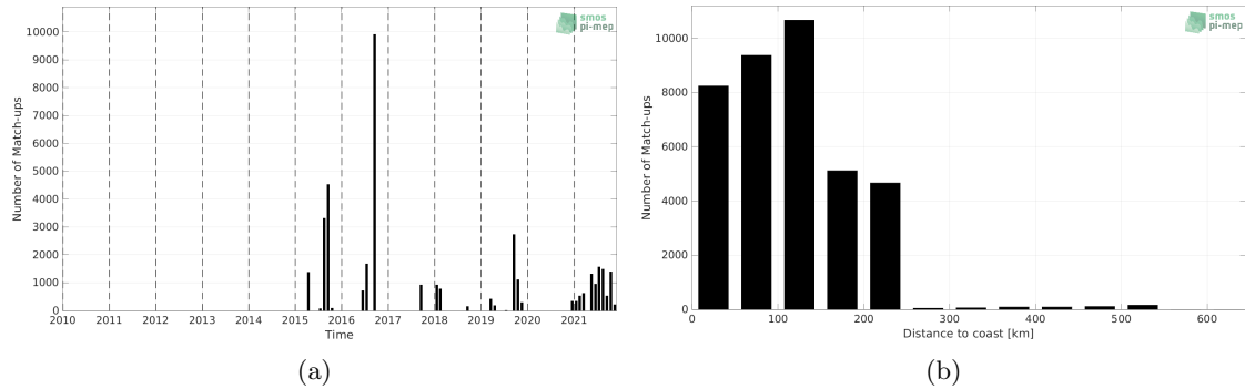
Figure 1: Number of match-ups between TSG (LEGOS-DM) and SMAP SSS L2 v5 (RSS) SSS as a function of time (a) and as function of the distance to coast (b) over the Arctic Ocean Pi-MEP region and for the full satellite product period.
