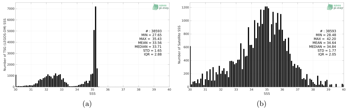
Figure 2: Histograms of SSS from TSG (LEGOS-DM) (a) and SMAP SSS L2 v5 (RSS) (b) considering all match-up pairs per bins of 0.1 over the Arctic Ocean Pi-MEP region and for the full satellite product period.
