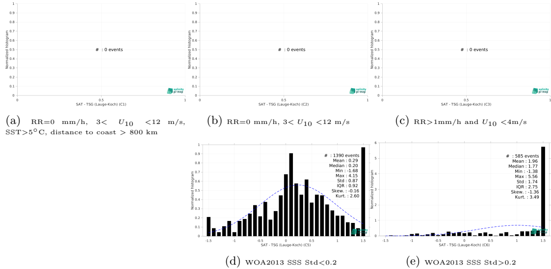
Figure 13: Normalized histogram of \Delta SSS (SMAP SSS L2 v5 (RSS) - TSG (Lauge-Koch)) for 5 different subdatasets corresponding to: RR=0 mm/h, 3 < U_{10} < 12 m/s, SST > 5°C, distance to coast > 800 km (a), RR=0 mm/h, 3 < U_{10} < 12 m/s (b), RR > 1mm/h and U_{10} < 4 m/s (c), WOA2013 SSS Std < 0.2 (d), WOA2013 SSS Std > 0.2 (e).
