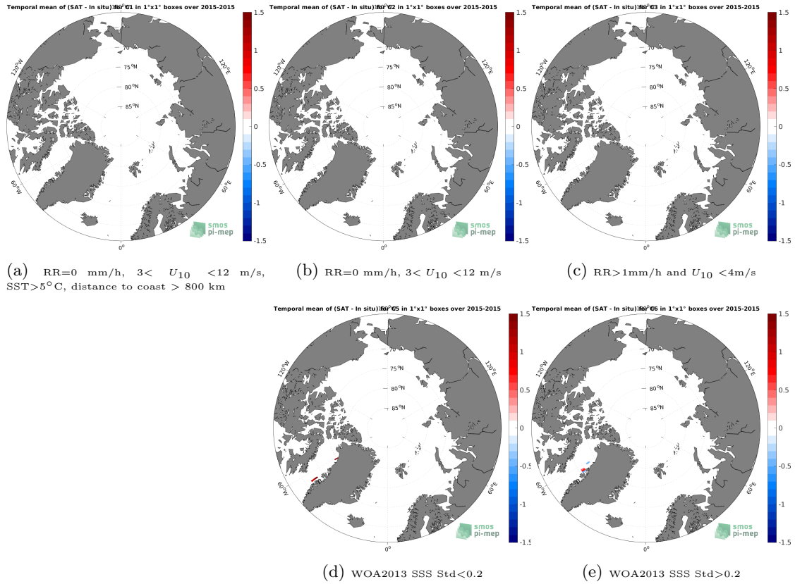
Figure 12: Temporal mean gridded over spatial boxes of size 1^\circ \times 1^\circ of \Delta SSS (SMAP SSS L2 v5 (RSS) - TSG (GOSUD-Sailing-ship)) for 5 different subdatasets corresponding to: RR=0 mm/h, 3 < U_{10} < 12 m/s, SST > 5°C, distance to coast > 800 km (a), RR=0 mm/h, 3 < U_{10} < 12 m/s (b), RR > 1mm/h and U_{10} < 4 m/s (c), WOA2013 SSS Std < 0.2 (d), WOA2013 SSS Std > 0.2 (e).
