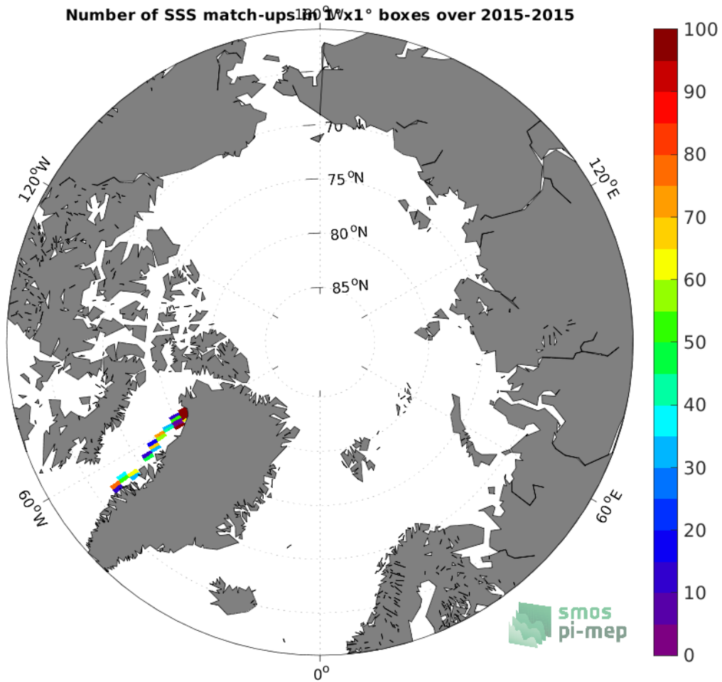
Figure 4: Number of SSS match-ups between TSG (GOSUD-Sailing-ship) SSS and the SMAP SSS L2 v5 (RSS) SSS product for the Arctic Ocean Pi-MEP region over 1^{\circ} \times 1^{\circ} boxes and for the full satellite product period.
