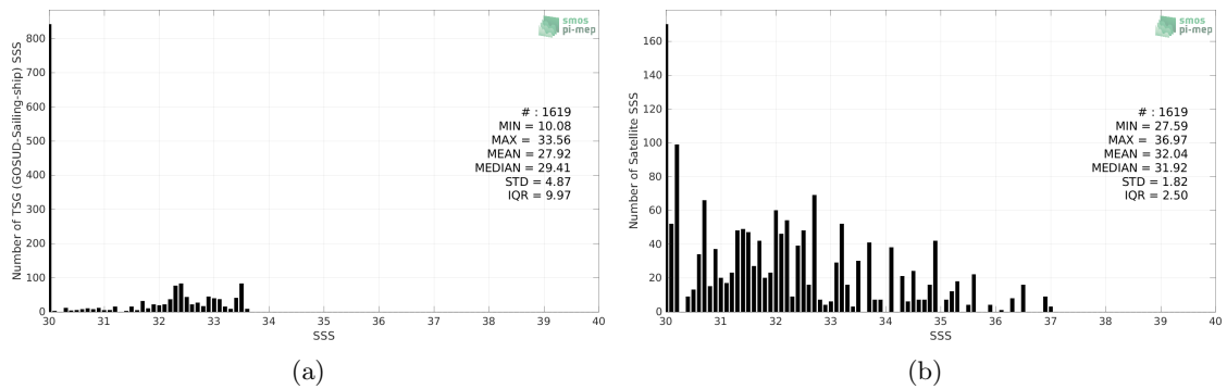
Figure 2: Histograms of SSS from TSG (GOSUD-Sailing-ship) (a) and SMAP SSS L2 v5 (RSS) (b) considering all match-up pairs per bins of 0.1 over the Arctic Ocean Pi-MEP region and for the full satellite product period.
