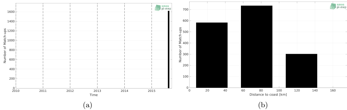
Figure 1: Number of match-ups between TSG (GOSUD-Sailing-ship) and SMAP SSS L2 v5 (RSS) SSS as a function of time (a) and as function of the distance to coast (b) over the Arctic Ocean Pi-MEP region and for the full satellite product period.
