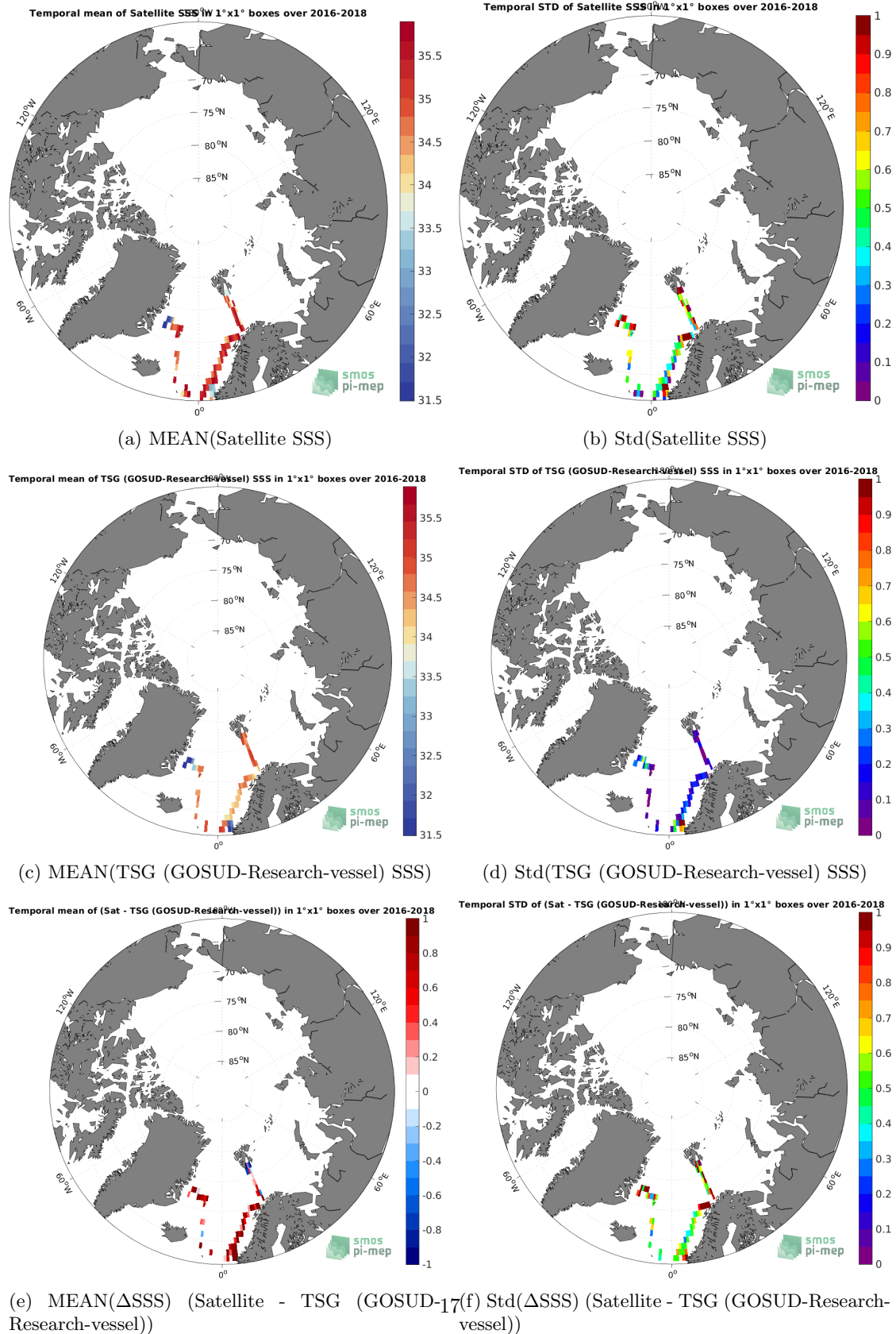
Figure 6: Temporal mean (left) and Std (right) of SSS from SMAP SSS L2 v5 (RSS) (top), TSG (GOSUD-Research-vessel) (middle), and of \Delta SSS (Satellite - TSG (GOSUD-Research-vessel)). Only match-up pairs are used to generate these maps.
