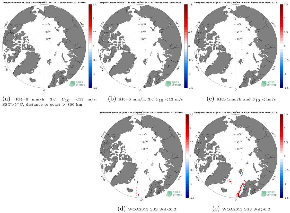
Figure 12: Temporal mean gridded over spatial boxes of size 1^\circ \times 1^\circ of \Delta\text{SSS} (SMAP SSS L2 v5 (RSS) - TSG (GOSUD-Research-vessel)) for 5 different subdatasets corresponding to: RR=0 mm/h, 3 < U_{10} < 12 m/s, SST > 5^\circ\text{C} , distance to coast > 800 km (a), RR=0 mm/h, 3 < U_{10} < 12 m/s (b), RR > 1 mm/h and U_{10} < 4 m/s (c), WOA2013 SSS Std < 0.2 (d), WOA2013 SSS Std > 0.2 (e).
