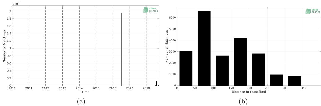
Figure 1: Number of match-ups between TSG (GOSUD-Research-vessel) and SMAP SSS L2 v5 (RSS) SSS as a function of time (a) and as function of the distance to coast (b) over the Arctic Ocean Pi-MEP region and for the full satellite product period.
