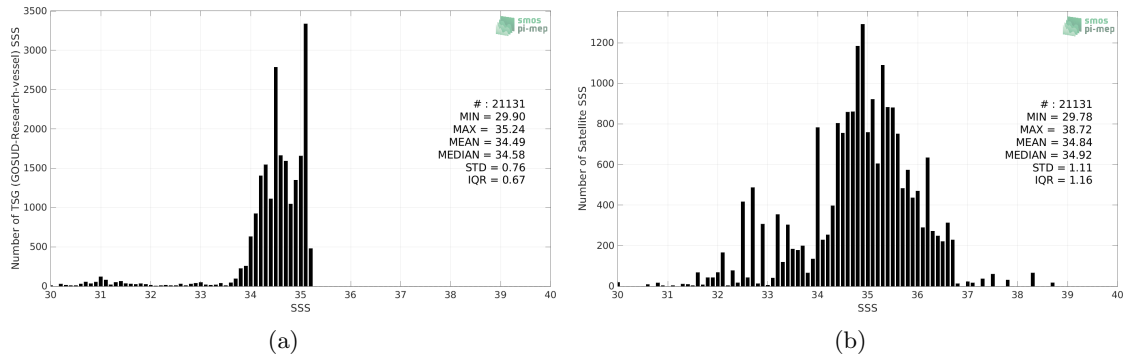
Figure 2: Histograms of SSS from TSG (GOSUD-Research-vessel) (a) and SMAP SSS L2 v5 (RSS) (b) considering all match-up pairs per bins of 0.1 over the Arctic Ocean Pi-MEP region and for the full satellite product period.
