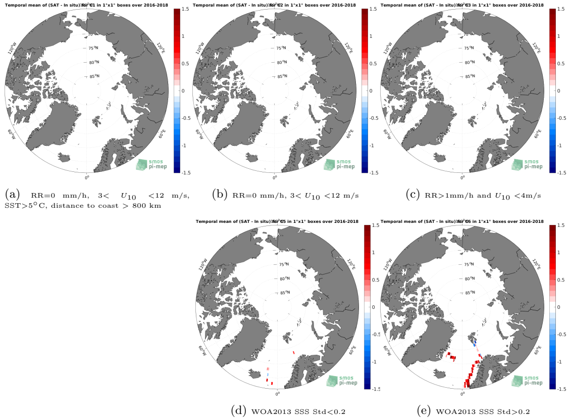
Figure 12: Temporal mean gridded over spatial boxes of size 1^\circ \times 1^\circ of \Delta SSS (SMAP SSS L2 v5 (RSS) - TSG (GOSUD-Research-vessel)) for 5 different subdatasets corresponding to:RR=0 mm/h, 3 < U_{10} < 12 m/s, SST>5°C, distance to coast > 800 km (a), RR=0 mm/h, 3 < U_{10} < 12 m/s (b), RR>1mm/h and U_{10} < 4 m/s (c), WOA2013 SSS Std<0.2 (d), WOA2013 SSS Std>0.2 (e).
