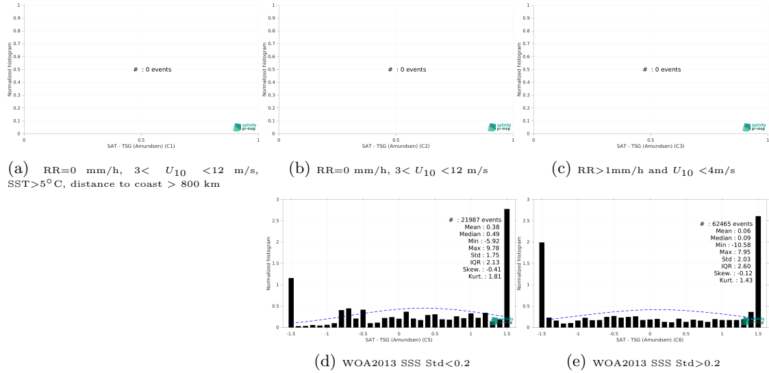
Figure 13: Normalized histogram of \Delta SSS (SMAP SSS L2 v5 (RSS) - TSG (Amundsen)) for 5 different subdatasets corresponding to: RR=0 mm/h, 3 < U_{10} < 12 m/s, SST>5°C, distance to coast > 800 km (a), RR=0 mm/h, 3 < U_{10} < 12 m/s (b), RR>1mm/h and U_{10} < 4 m/s (c), WOA2013 SSS Std<0.2 (d), WOA2013 SSS Std>0.2 (e).
