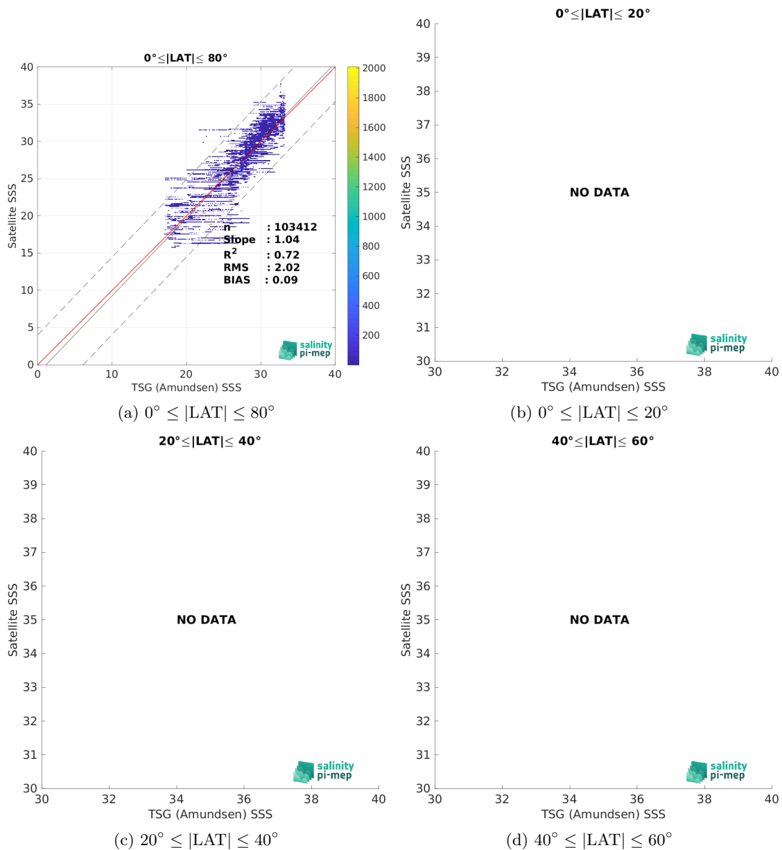
Figure 9: Contour maps of the concentration of SMAP SSS L2 v5 (RSS) SSS (y-axis) versus TSG (Amundsen) SSS (x-axis) at match-up pairs for different latitude bands. For each plot, the red line shows x=y . The black thin and dashed lines indicate a linear fit through the data cloud and the \pm 95\% confidence levels, respectively. The number match-up pairs n , the slope and R^2 coefficient of the linear fit, the root mean square (RMS) and the mean bias between satellite and in situ data are indicated for each latitude band in each plots.
