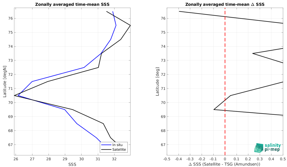
Figure 8: Left panel: Zonal mean SSS from SMAP SSS L2 v5 (RSS) satellite product (black) and from TSG (Amundsen) (blue). Right panel: Zonal mean of \Delta SSS (Satellite - TSG (Amundsen)) for all the collected Pi-MEP match-up pairs estimated over the full satellite product period.
