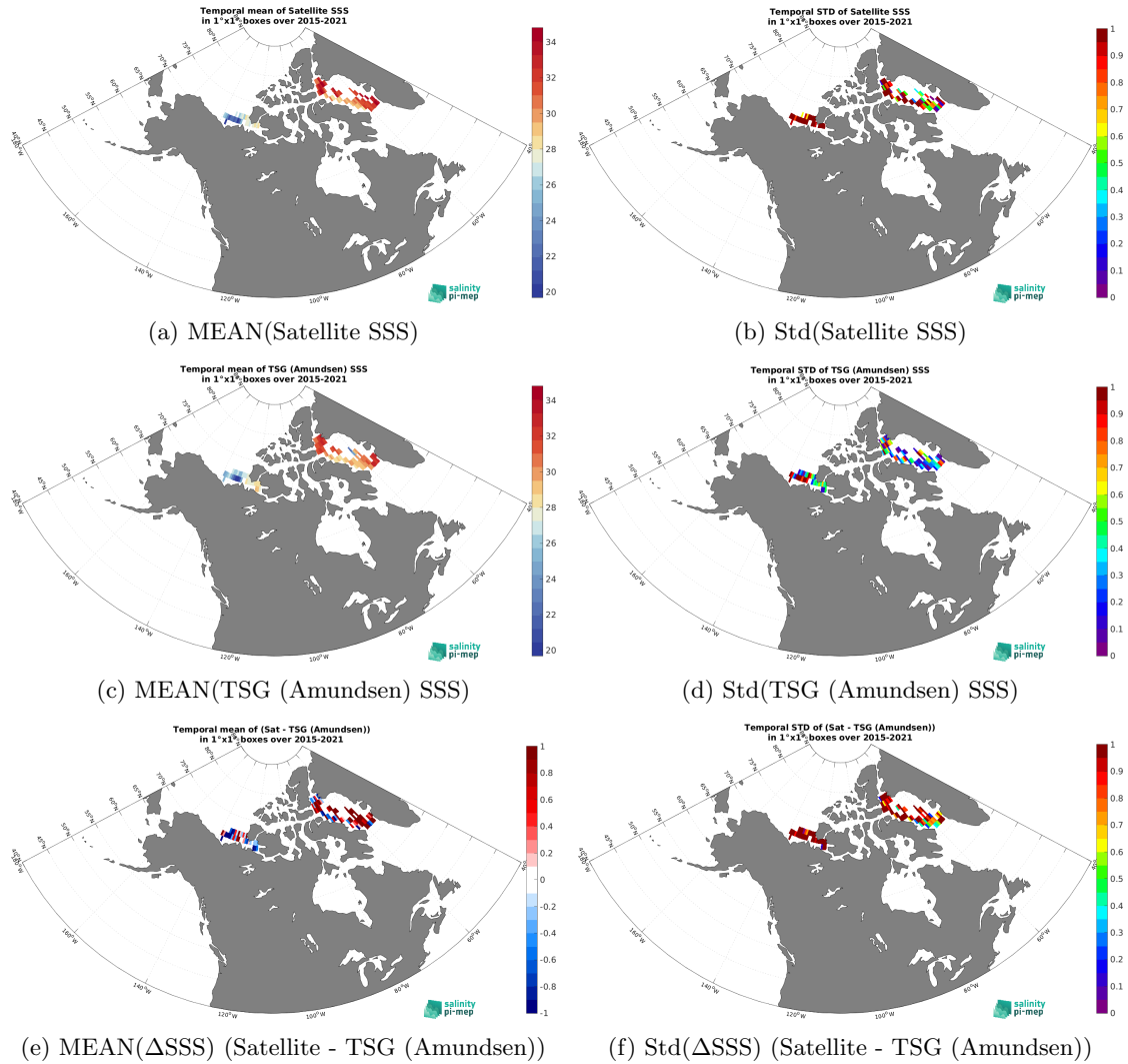
Figure 6: Temporal mean (left) and Std (right) of SSS from SMAP SSS L2 v5 (RSS) (top), TSG (Amundsen) (middle), and of \Delta SSS (Satellite - TSG (Amundsen)). Only match-up pairs are used to generate these maps.
