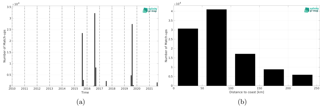
Figure 1: Number of match-ups between TSG (Amundsen) and SMAP SSS L2 v5 (RSS) SSS as a function of time (a) and as function of the distance to coast (b) over the Arctic Ocean Pi-MEP region and for the full satellite product period.
