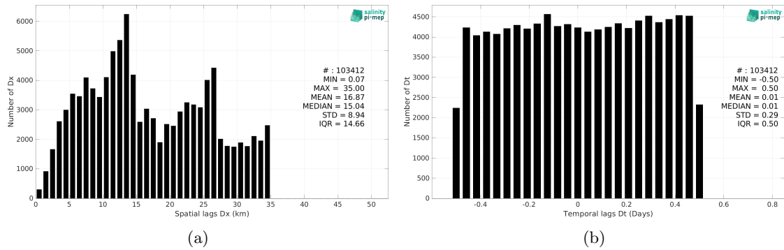
Figure 5: Histograms of the spatial (a) and temporal (b) lags between the location/time of the TSG (Amundsen) measurement and the date of the corresponding SMAP SSS L2 v5 (RSS) SSS pixel.
