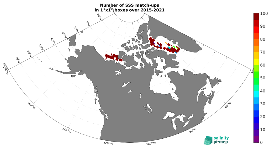
Figure 4: Number of SSS match-ups between TSG (Amundsen) SSS and the SMAP SSS L2 v5 (RSS) SSS product for the Arctic Ocean Pi-MEP region over 1^\circ \times 1^\circ boxes and for the full satellite product period.
