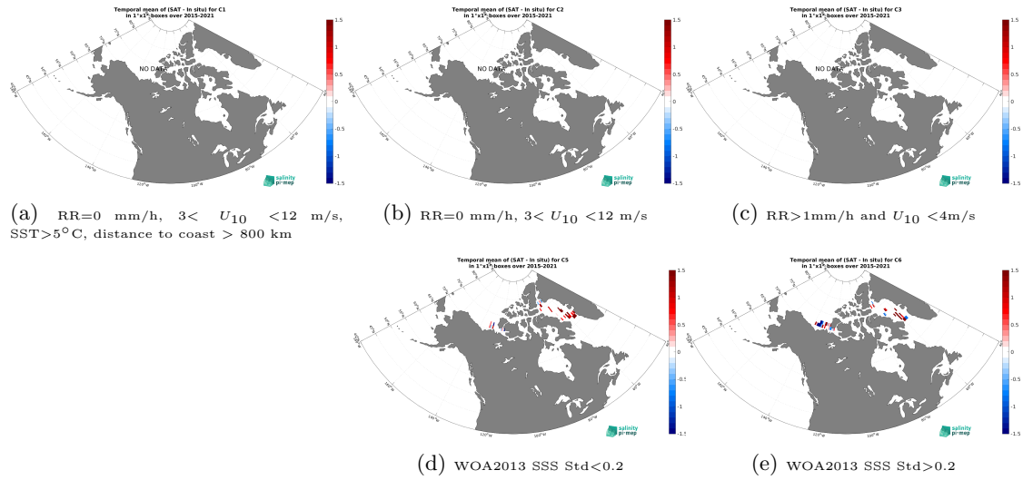
Figure 12: Temporal mean gridded over spatial boxes of size 1^{\circ}\times 1^{\circ} of \Delta\text{SSS} (SMAP SSS L2 v5 (RSS) - TSG (Amundsen)) for 5 different subdatasets corresponding to: RR=0 mm/h, 3 < U_{10} < 12 m/s, SST > 5^{\circ}\text{C} , distance to coast > 800 km (a), RR=0 mm/h, 3 < U_{10} < 12 m/s (b), RR > 1 mm/h and U_{10} < 4 m/s (c), WOA2013 SSS Std < 0.2 (d), WOA2013 SSS Std > 0.2 (e).
