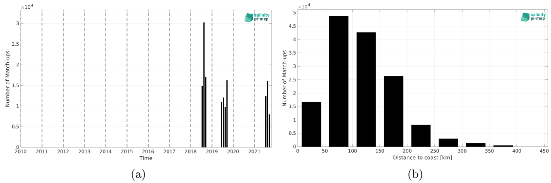
Figure 1: Number of match-ups between Saildrone and SMAP SSS L2 v5 (RSS) SSS as a function of time (a) and as function of the distance to coast (b) over the Arctic Ocean Pi-MEP region and for the full satellite product period.
