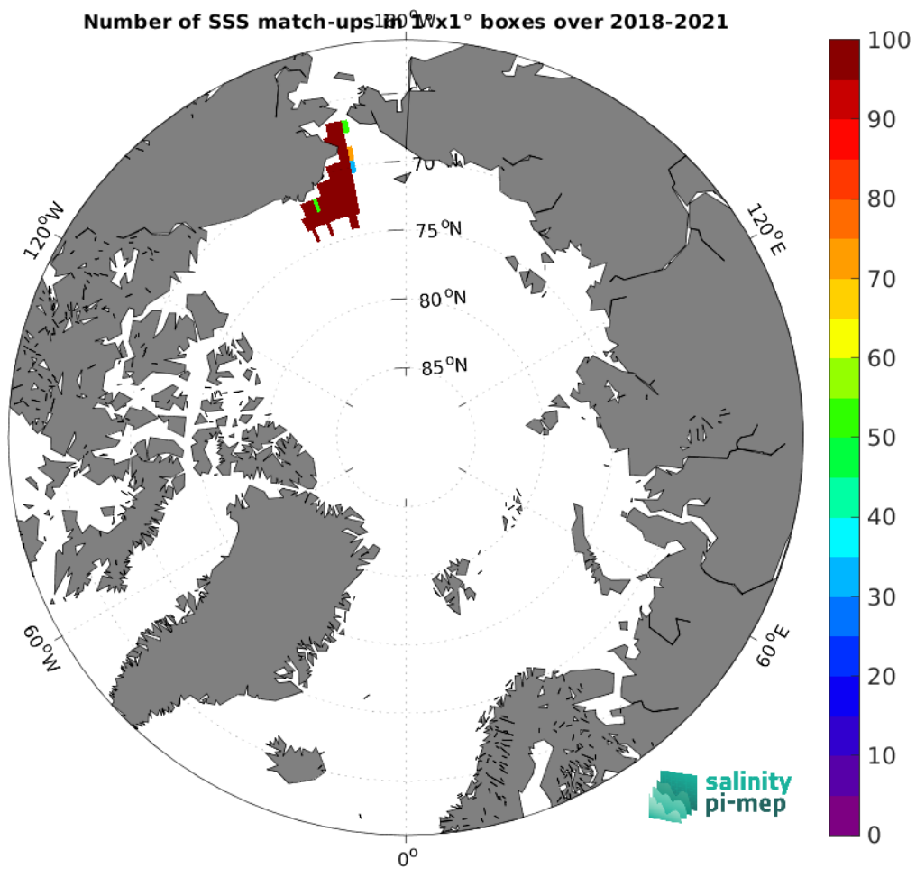
Figure 4: Number of SSS match-ups between Saildrone SSS and the SMAP SSS L2 v5 (RSS) SSS product for the Arctic Ocean Pi-MEP region over 1^\circ \times 1^\circ boxes and for the full satellite product period.
