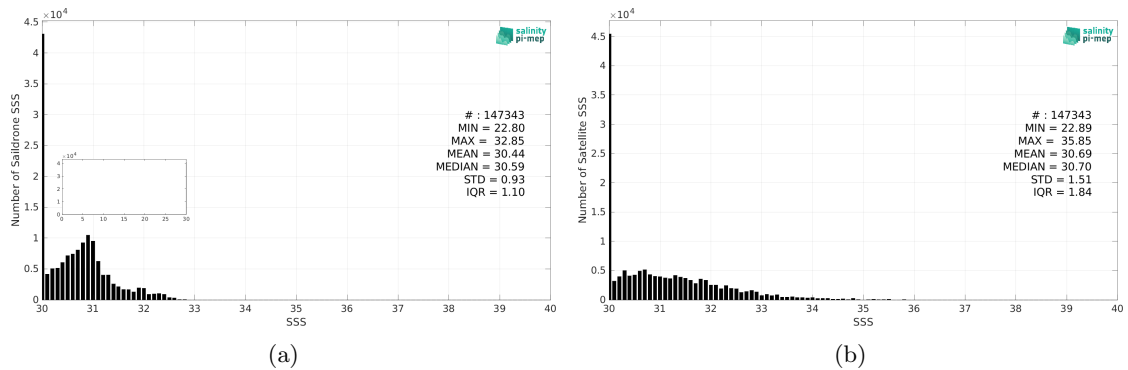
Figure 2: Histograms of SSS from Saildrone (a) and SMAP SSS L2 v5 (RSS) (b) considering all match-up pairs per bins of 0.1 over the Arctic Ocean Pi-MEP region and for the full satellite product period.
