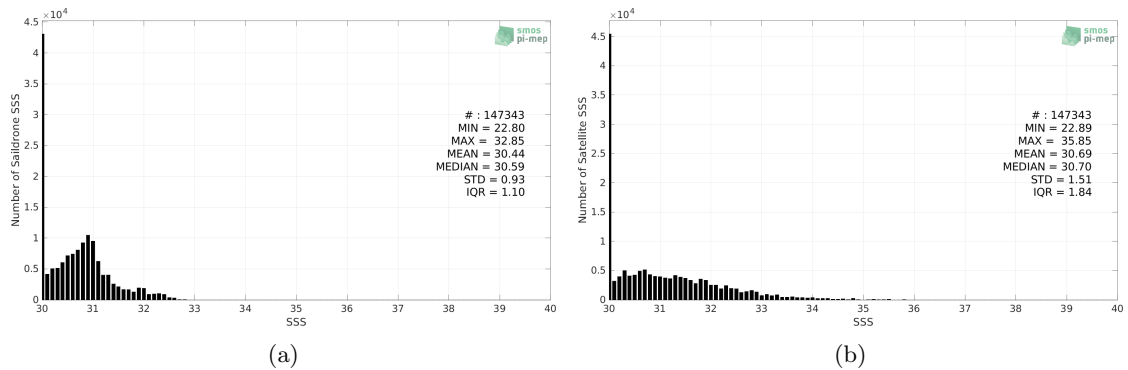
Figure 2: Histograms of SSS from Sairdrone (a) and SMAP SSS L2 v5 (RSS) (b) considering all match-up pairs per bins of 0.1 over the Arctic Ocean Pi-MEP region and for the full satellite product period.
