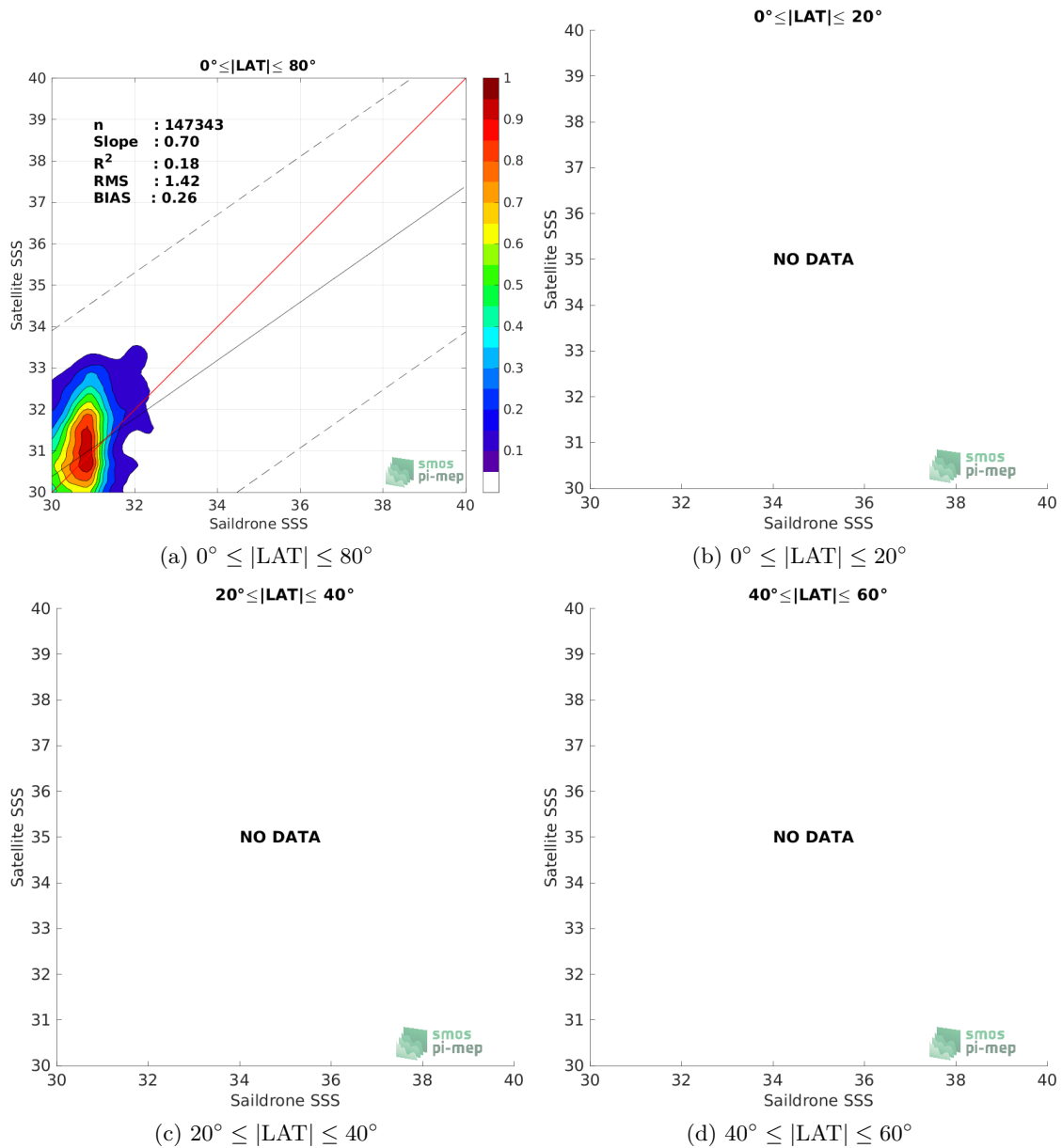
Figure 9: Contour maps of the concentration of SMAP SSS L2 v5 (RSS) SSS (y-axis) versus Sailldrone SSS (x-axis) at match-up pairs for different latitude bands. For each plot, the red line shows x=y . The black thin and dashed lines indicate a linear fit through the data cloud and the \pm 95\% confidence levels, respectively. The number match-up pairs n , the slope and R^2 coefficient of the linear fit, the root mean square (RMS) and the mean bias between satellite and in situ data are indicated for each latitude band in each plots.
