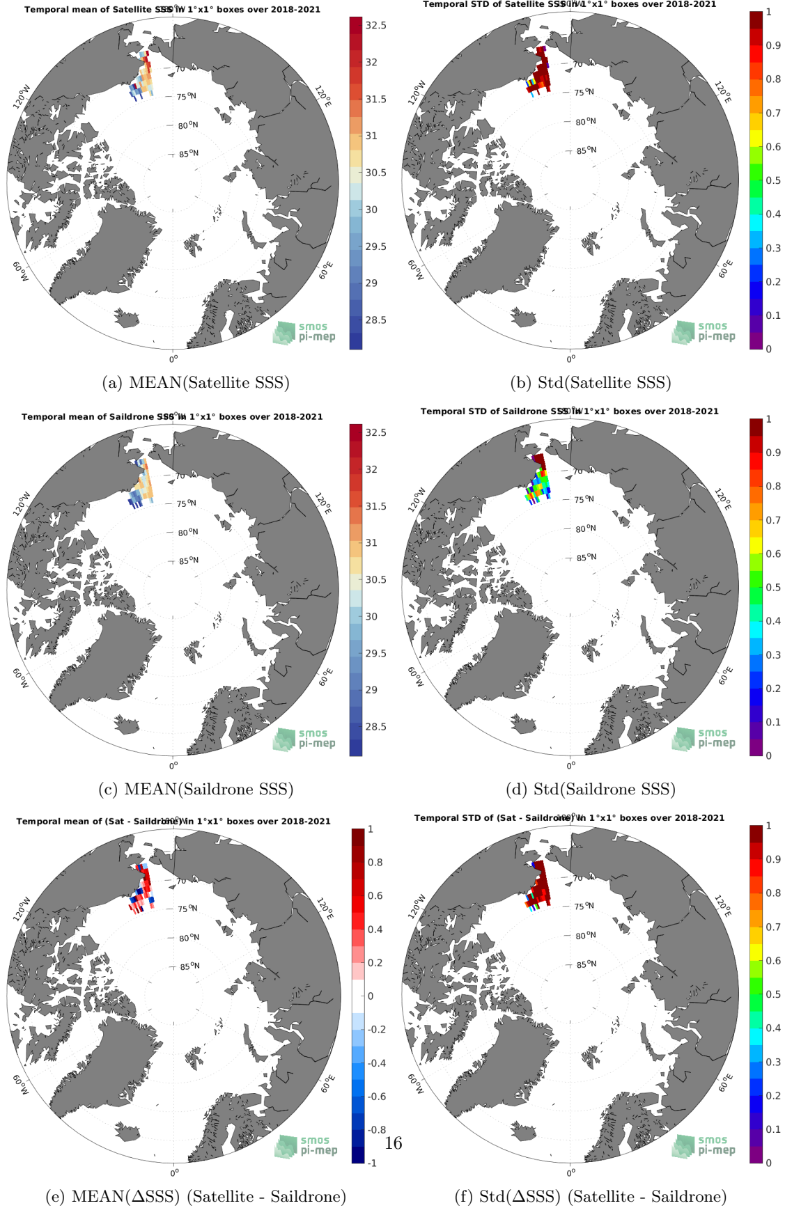
Figure 6: Temporal mean (left) and Std (right) of SSS from SMAP SSS L2 v5 (RSS) (top), Saildrone (middle), and of \Delta SSS (Satellite - Saildrone). Only match-up pairs are used to generate these maps.
