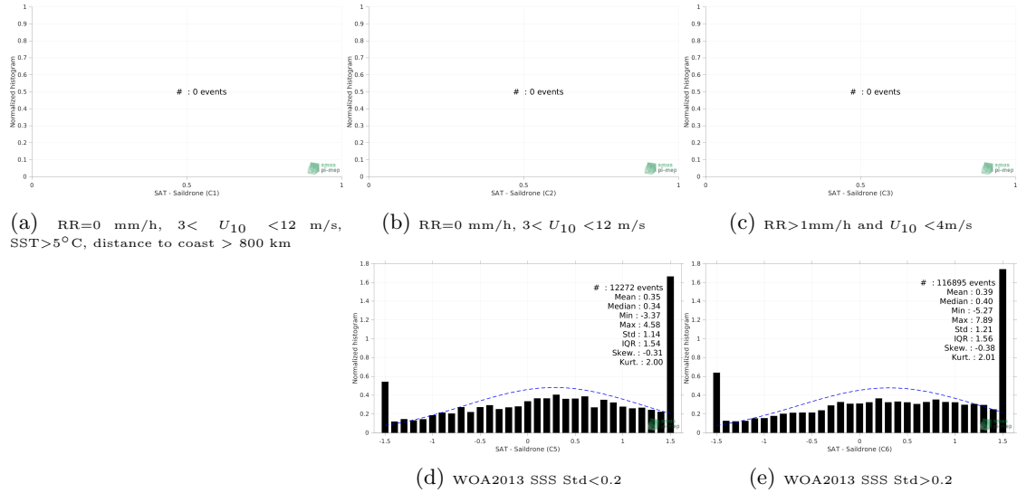
Figure 13: Normalized histogram of \Delta SSS (SMAP SSS L2 v5 (RSS) - Sailldrone) for 5 different subdatasets corresponding to: RR=0 mm/h, 3 < U_{10} < 12 m/s, SST > 5°C, distance to coast > 800 km (a), RR=0 mm/h, 3 < U_{10} < 12 m/s (b), RR > 1mm/h and U_{10} < 4 m/s (c), WOA2013 SSS Std < 0.2 (d), WOA2013 SSS Std > 0.2 (e).
