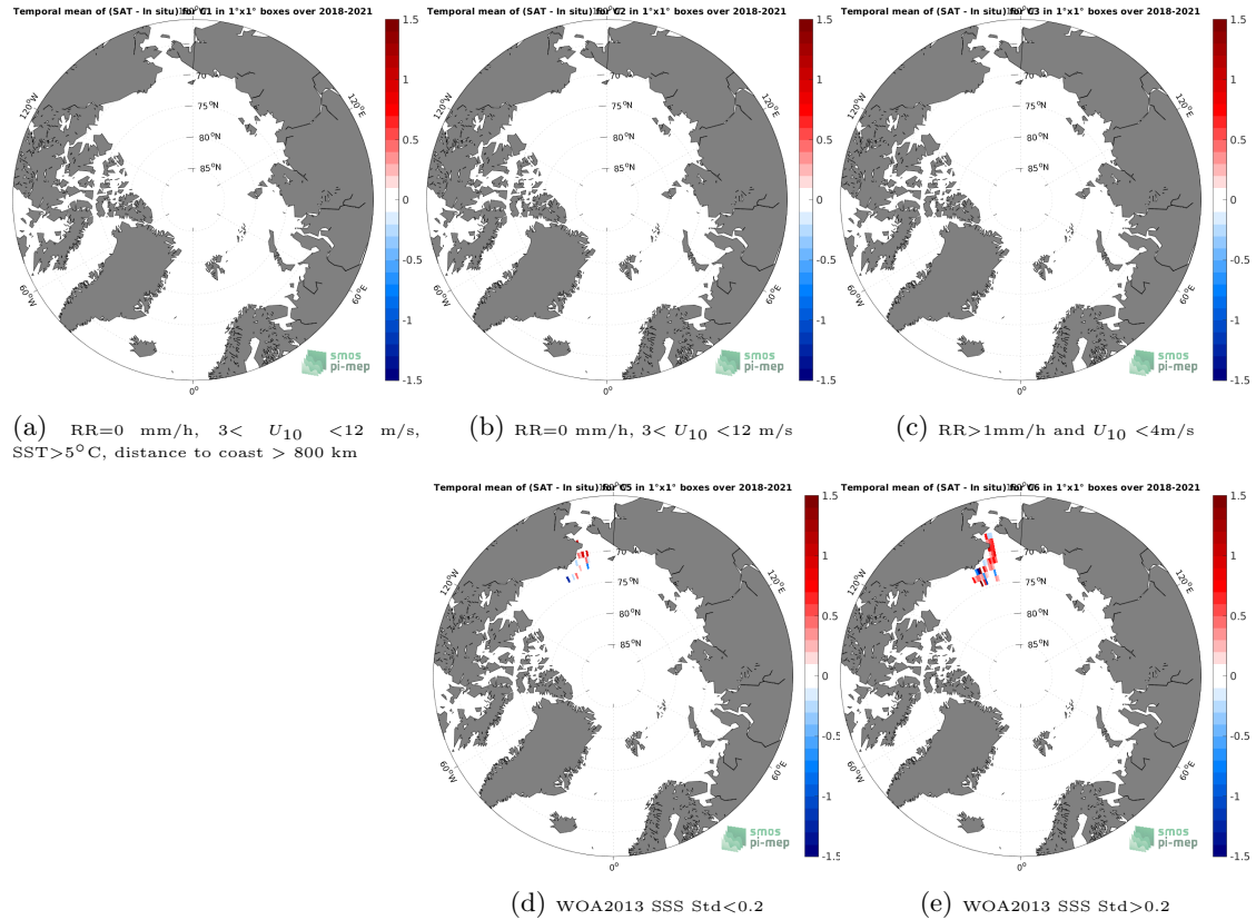
Figure 12: Temporal mean gridded over spatial boxes of size 1^{\circ}\times 1^{\circ} of \Delta\text{SSS} (SMAP SSS L2 v5 (RSS) - Saikrone) for 5 different subdatasets corresponding to:RR=0 mm/h, 3 < U_{10} < 12 m/s, SST > 5^{\circ}\text{C} , distance to coast > 800 km (a), RR=0 mm/h, 3 < U_{10} < 12 m/s (b), RR > 1 mm/h and U_{10} < 4 m/s (c), WOA2013 SSS Std < 0.2 (d), WOA2013 SSS Std > 0.2 (e).
