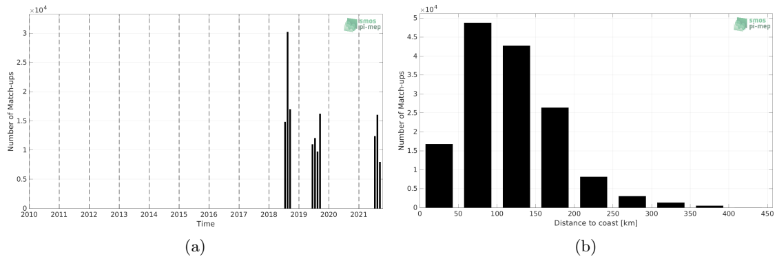
Figure 1: Number of match-ups between Sairdrone and SMAP SSS L2 v5 (RSS) SSS as a function of time (a) and as function of the distance to coast (b) over the Arctic Ocean Pi-MEP region and for the full satellite product period.
