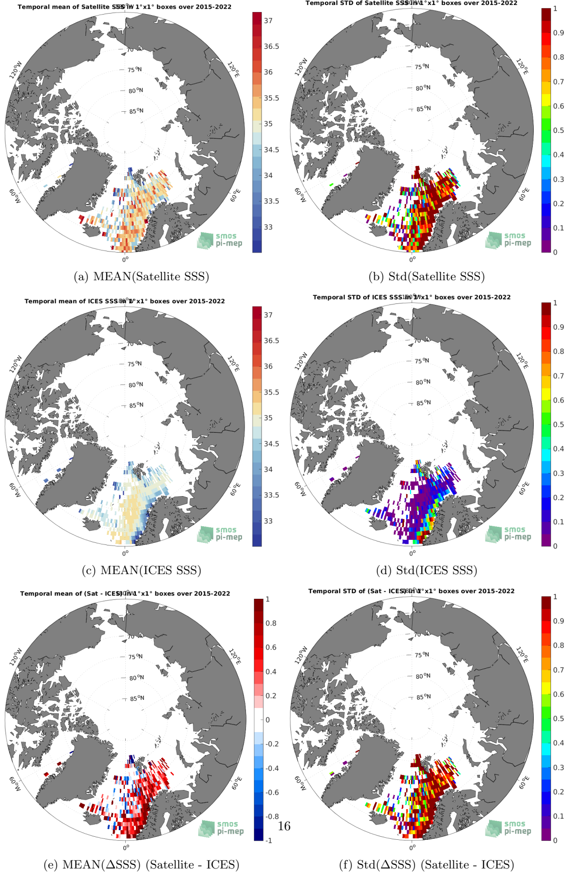
Figure 6: Temporal mean (left) and Std (right) of SSS from SMAP SSS L2 v5 (RSS) (top), ICES (middle), and of \Delta SSS (Satellite - ICES). Only match-up pairs are used to generate these maps.
