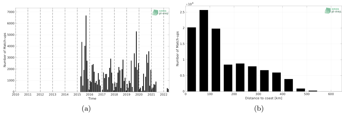
Figure 1: Number of match-ups between ICES and SMAP SSS L2 v5 (RSS) SSS as a function of time (a) and as function of the distance to coast (b) over the Arctic Ocean Pi-MEP region and for the full satellite product period.
