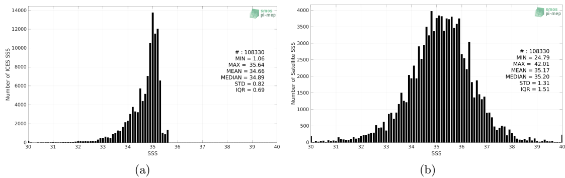
Figure 2: Histograms of SSS from ICES (a) and SMAP SSS L2 v5 (RSS) (b) considering all match-up pairs per bins of 0.1 over the Arctic Ocean Pi-MEP region and for the full satellite product period.
