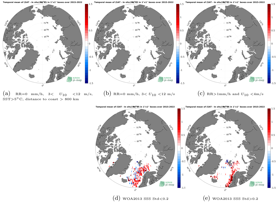
Figure 12: Temporal mean gridded over spatial boxes of size 1^{\circ}\times 1^{\circ} of \Delta\text{SSS} (SMAP SSS L2 v5 (RSS) - ICES) for 5 different subdatasets corresponding to:RR=0 mm/h, 3 < U_{10} < 12 m/s, SST > 5^{\circ}\text{C} , distance to coast > 800 km (a), RR=0 mm/h, 3 < U_{10} < 12 m/s (b), RR > 1 mm/h and U_{10} < 4 m/s (c), WOA2013 SSS Std < 0.2 (d), WOA2013 SSS Std > 0.2 (e).
