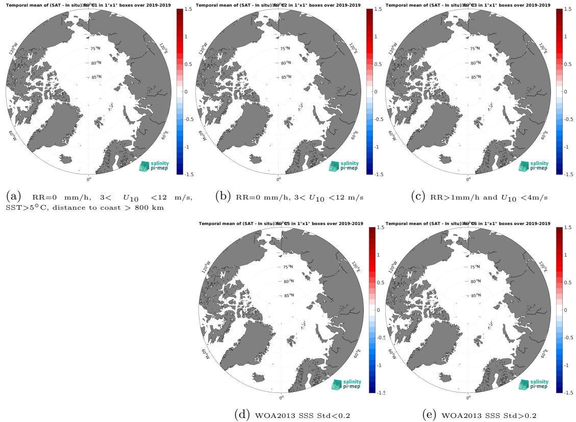
Figure 11: Temporal mean gridded over spatial boxes of size 1^{\circ}\times 1^{\circ} of \Delta\text{SSS} (SMAP SSS L2 v5 (RSS) - Surface drifters) for 5 different subdatasets corresponding to: RR=0 mm/h, 3 < U_{10} < 12 m/s, SST > 5^{\circ}\text{C} , distance to coast > 800 km (a), RR=0 mm/h, 3 < U_{10} < 12 m/s (b), RR > 1 mm/h and U_{10} < 4 m/s (c), WOA2013 SSS Std < 0.2 (d), WOA2013 SSS Std > 0.2 (e).
