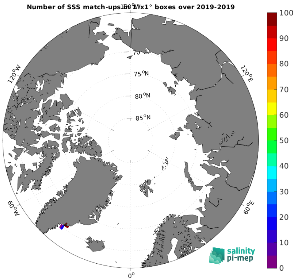
Figure 3: Number of SSS match-ups between Surface drifters SSS and the SMAP SSS L2 v5 (RSS) SSS product for the Arctic Ocean Pi-MEP region over 1^\circ \times 1^\circ boxes and for the full satellite product period.
