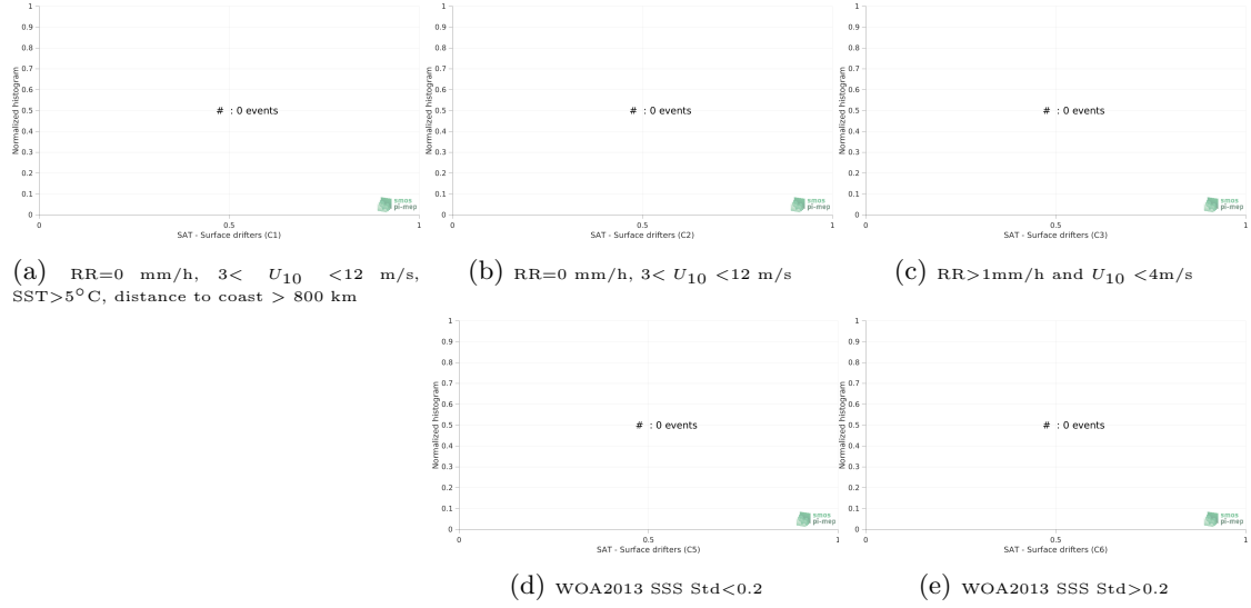
Figure 12: Normalized histogram of \Delta\text{SSS} (SMAP SSS L2 v5 (RSS) - Surface drifters) for 5 different subdatasets corresponding to: RR=0 mm/h, 3 < U_{10} < 12 m/s, SST > 5^\circ\text{C} , distance to coast > 800 km (a), RR=0 mm/h, 3 < U_{10} < 12 m/s (b), RR > 1 mm/h and U_{10} < 4 m/s (c), WOA2013 SSS Std < 0.2 (d), WOA2013 SSS Std > 0.2 (e).
