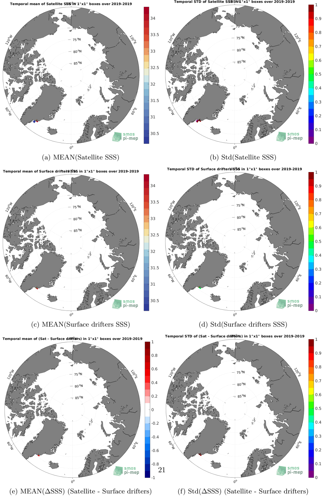
Figure 5: Temporal mean (left) and Std (right) of SSS from SMAP SSS L2 v5 (RSS) (top), Surface drifters (middle), and of \Delta SSS (Satellite - Surface drifters). Only match-up pairs are used to generate these maps.
