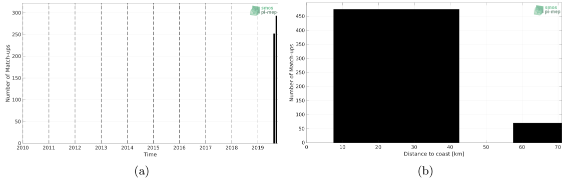
Figure 1: Number of match-ups between Surface drifters and SMAP SSS L2 v5 (RSS) SSS as a function of time (a) and as function of the distance to coast (b) over the Arctic Ocean Pi-MEP region and for the full satellite product period.
