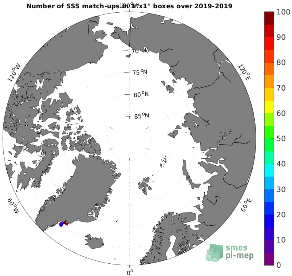
Figure 3: Number of SSS match-ups between Surface drifters SSS and the SMAP SSS L2 v5 (RSS) SSS product for the Arctic Ocean Pi-MEP region over 1^{\circ} \times 1^{\circ} boxes and for the full satellite product period.
