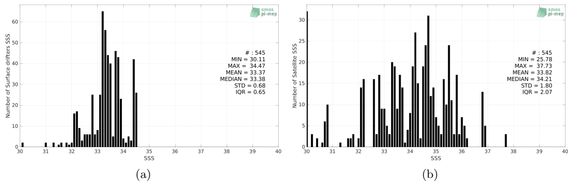
Figure 2: Histograms of SSS from Surface drifters (a) and SMAP SSS L2 v5 (RSS) (b) considering all match-up pairs per bins of 0.1 over the Arctic Ocean Pi-MEP region and for the full satellite product period.
