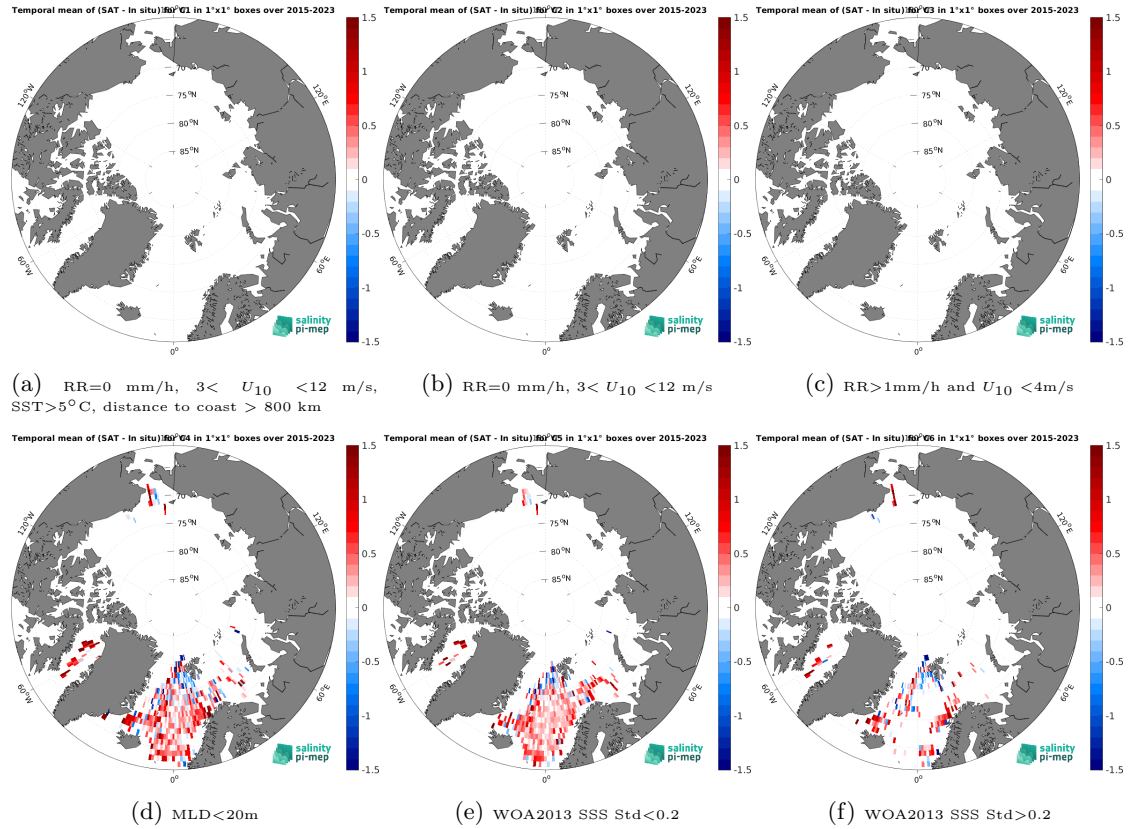
Figure 12: Temporal mean gridded over spatial boxes of size 1^{\circ}\times 1^{\circ} of \Delta\text{SSS} (SMAP SSS L2 v5 (RSS) - Argo) for 6 different subdatasets corresponding to: RR=0 mm/h, 3 < U_{10} < 12 m/s, SST > 5^{\circ}\text{C} , distance to coast > 800 km (a), RR=0 mm/h, 3 < U_{10} < 12 m/s (b), RR > 1 mm/h and U_{10} < 4 m/s (c), MLD < 20\text{m} (d), WOA2013 SSS Std < 0.2 (e), WOA2013 SSS Std > 0.2 (f).
