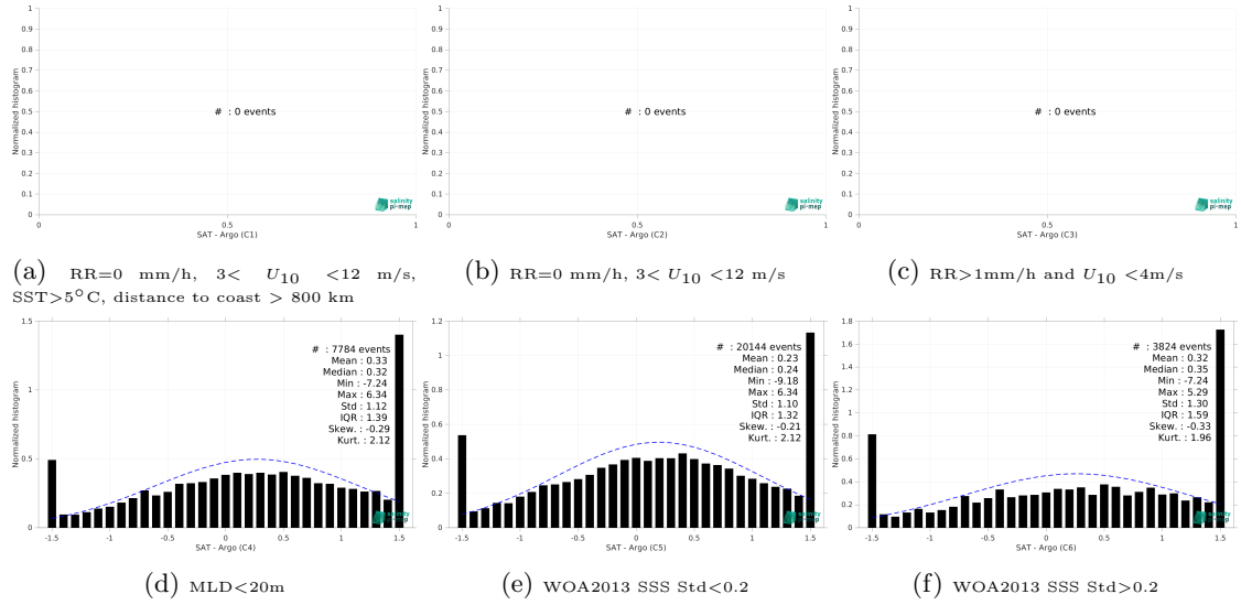
Figure 13: Normalized histogram of \Delta SSS (SMAP SSS L2 v5 (RSS) - Argo) for 6 different subdatasets corresponding to: RR=0 mm/h, 3 < U_{10} < 12 m/s, SST > 5^{\circ}C , distance to coast > 800 km (a), RR=0 mm/h, 3 < U_{10} < 12 m/s (b), RR > 1 mm/h and U_{10} < 4 m/s (c), MLD < 20 m (d), WOA2013 SSS Std < 0.2 (e), WOA2013 SSS Std > 0.2 (f).
