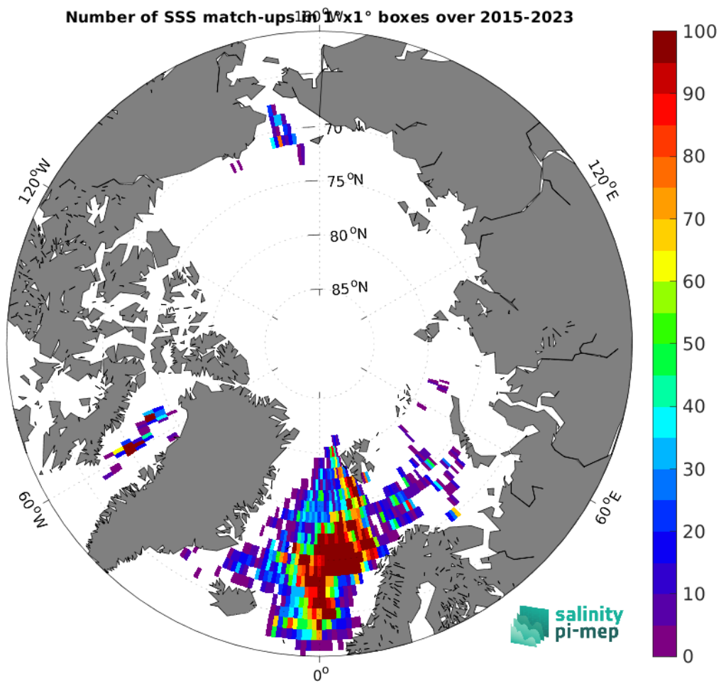
Figure 4: Number of SSS match-ups between Argo SSS and the SMAP SSS L2 v5 (RSS) SSS product for the Arctic Ocean Pi-MEP region over 1^\circ \times 1^\circ boxes and for the full satellite product period.
