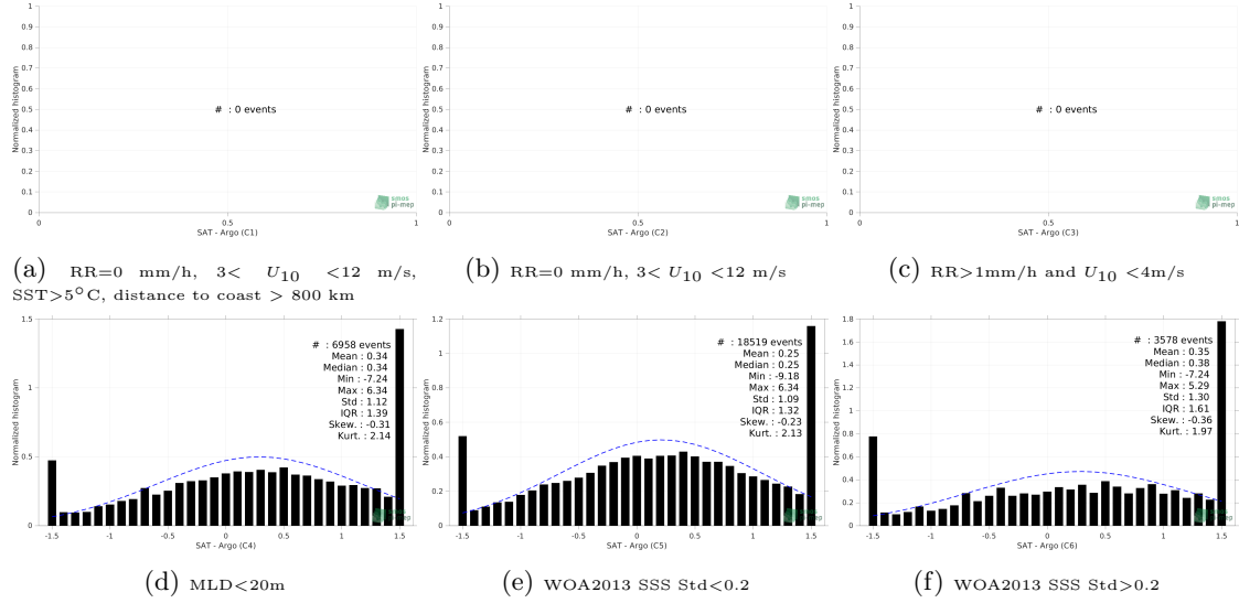
Figure 13: Normalized histogram of \Delta\text{SSS} (SMAP SSS L2 v5 (RSS) - Argo) for 6 different subdatasets corresponding to: RR=0 mm/h, 3 < U_{10} < 12 m/s, SST > 5^{\circ}\text{C} , distance to coast > 800 km (a), RR=0 mm/h, 3 < U_{10} < 12 m/s (b), RR > 1\text{mm/h} and U_{10} < 4\text{m/s} (c), MLD < 20\text{m} (d), WOA2013 SSS Std < 0.2 (e), WOA2013 SSS Std > 0.2 (f).
