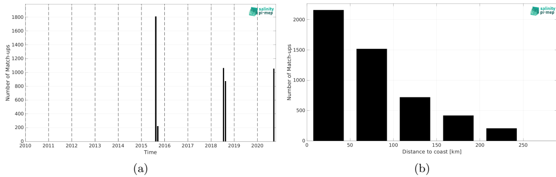
Figure 2: Number of match-ups between TSG (SAMOS) and SMAP SSS L2 v5.3 (RSS) SSS as a function of time (a) and as function of the distance to coast (b) over the Arctic Ocean Pi-MEP region and for the full satellite product period.
