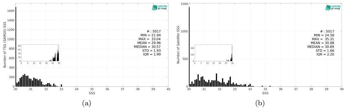
Figure 3: Histograms of SSS from TSG (SAMOS) (a) and SMAP SSS L2 v5.3 (RSS) (b) considering all match-up pairs per bins of 0.1 over the Arctic Ocean Pi-MEP region and for the full satellite product period.
