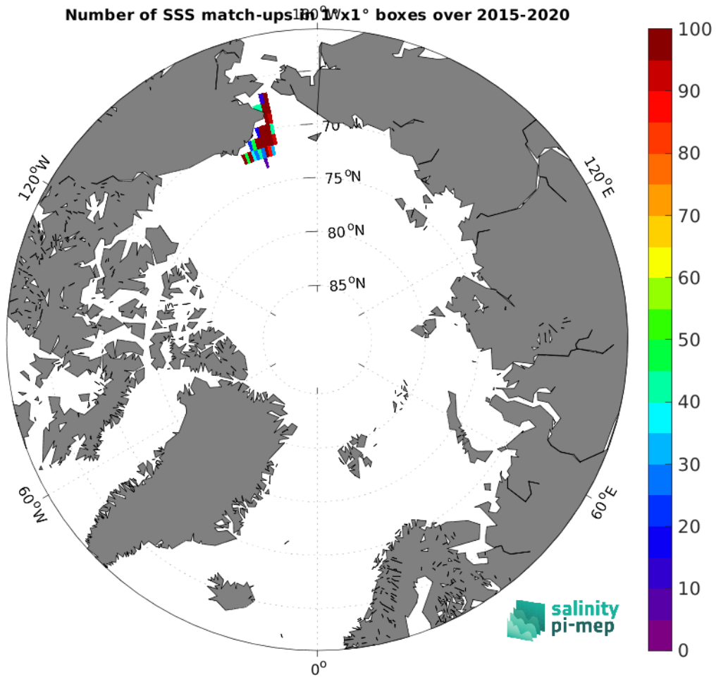
Figure 5: Number of SSS match-ups between TSG (SAMOS) SSS and the SMAP SSS L2 v5.3 (RSS) SSS product for the Arctic Ocean Pi-MEP region over 1^\circ \times 1^\circ boxes and for the full satellite product period.
