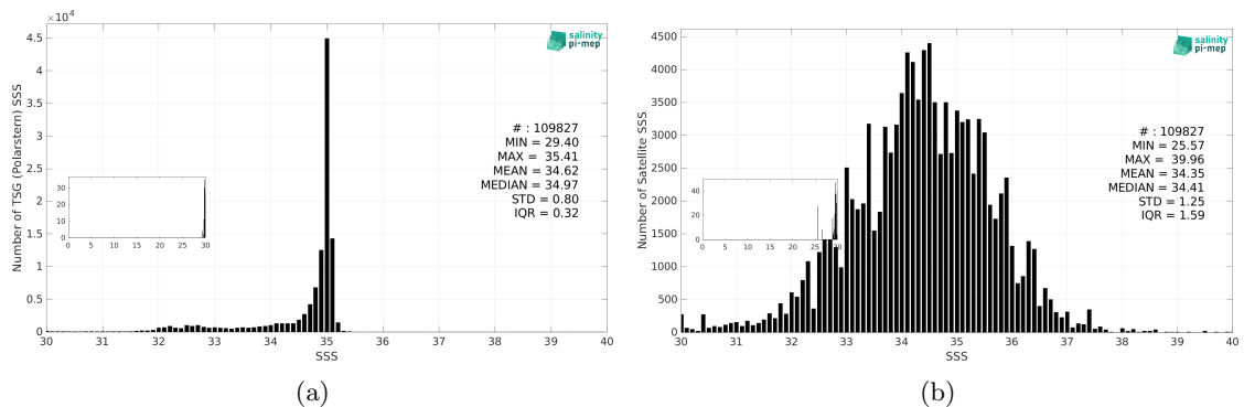
Figure 3: Histograms of SSS from TSG (Polarstern) (a) and SMAP SSS L2 v5.3 (RSS) (b) considering all match-up pairs per bins of 0.1 over the Arctic Ocean Pi-MEP region and for the full satellite product period.
