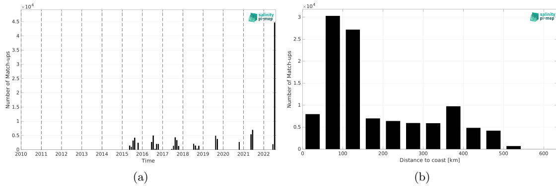
Figure 2: Number of match-ups between TSG (Polarstern) and SMAP SSS L2 v5.3 (RSS) SSS as a function of time (a) and as function of the distance to coast (b) over the Arctic Ocean Pi-MEP region and for the full satellite product period.
