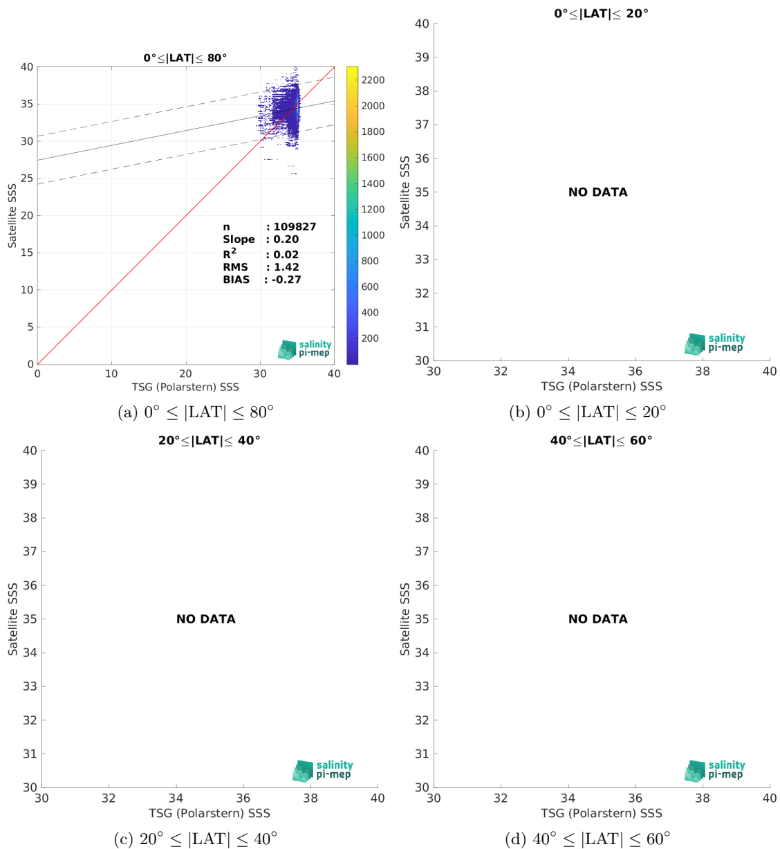
Figure 10: Contour maps of the concentration of SMAP SSS L2 v5.3 (RSS) SSS (y-axis) versus TSG (Polarstern) SSS (x-axis) at match-up pairs for different latitude bands. For each plot, the red line shows x=y . The black thin and dashed lines indicate a linear fit through the data cloud and the \pm 95\% confidence levels, respectively. The number match-up pairs n , the slope and R^2 coefficient of the linear fit, the root mean square (RMS) and the mean bias between satellite and in situ data are indicated for each latitude band in each plots.
