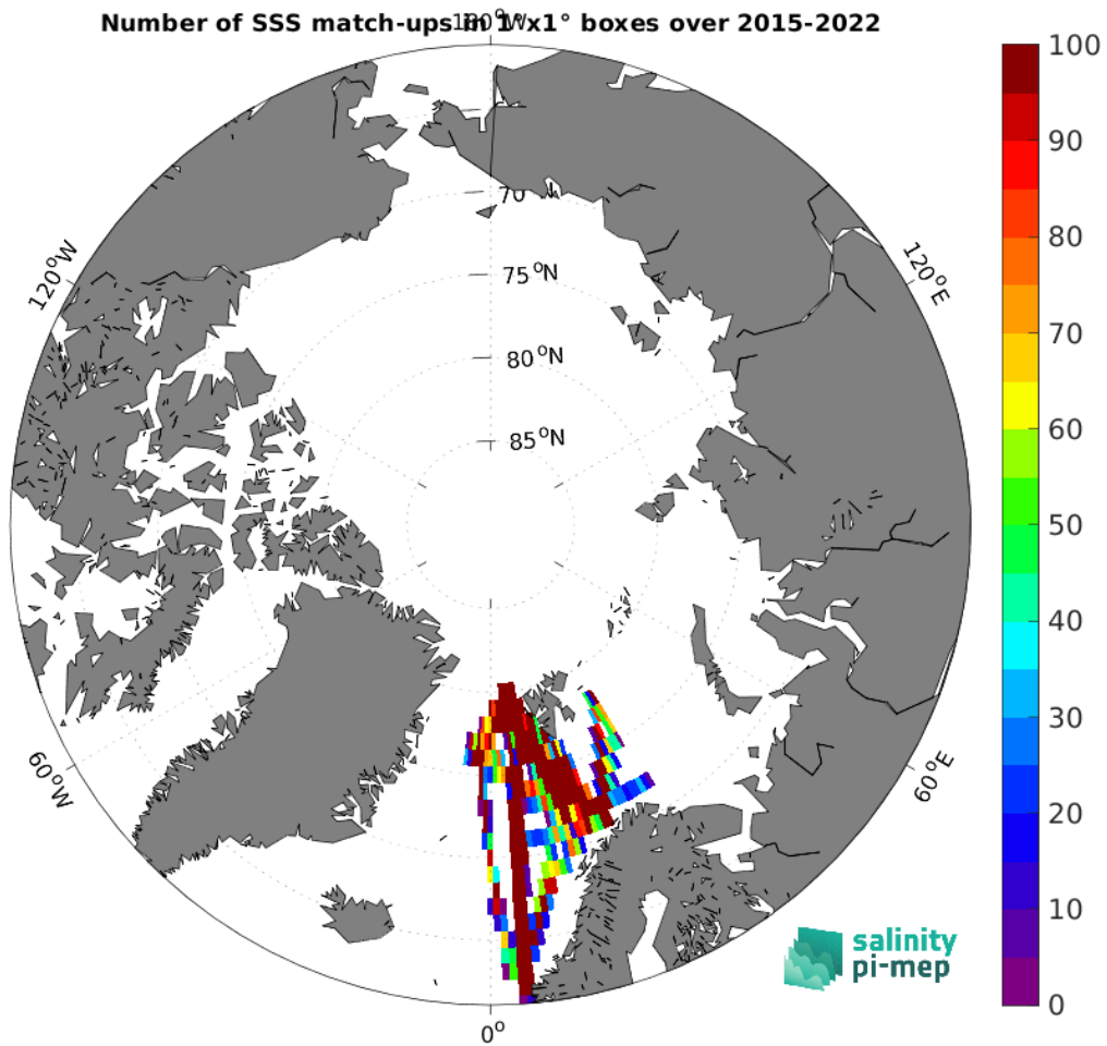
Figure 5: Number of SSS match-ups between TSG (Polarstern) SSS and the SMAP SSS L2 v5.3 (RSS) SSS product for the Arctic Ocean Pi-MEP region over 1^\circ \times 1^\circ boxes and for the full satellite product period.
