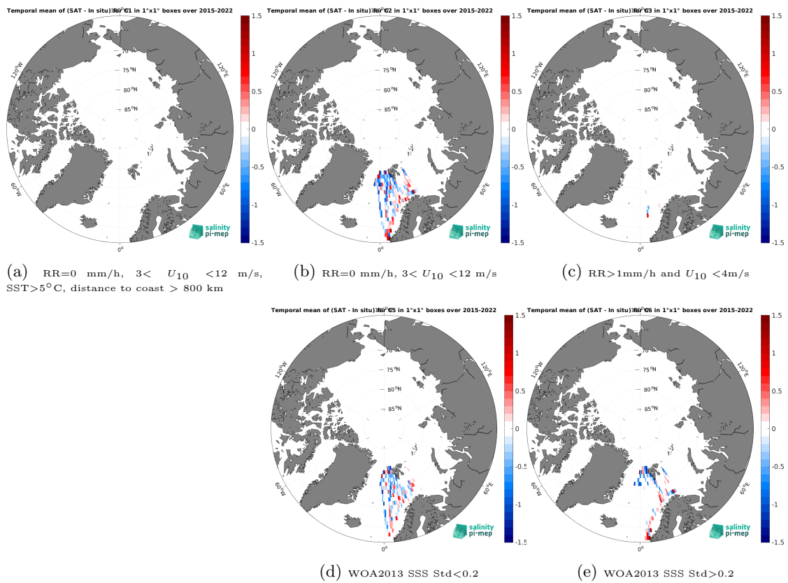
Figure 14: Temporal mean gridded over spatial boxes of size 1^\circ \times 1^\circ of \Delta SSS (SMAP SSS L2 v5.3 (RSS) - TSG (Polarstern)) for 5 different subdatasets corresponding to:RR=0 mm/h, 3 < U_{10} < 12 m/s, SST>5°C, distance to coast > 800 km (a), RR=0 mm/h, 3 < U_{10} < 12 m/s (b), RR>1mm/h and U_{10} < 4 m/s (c), WOA2013 SSS Std<0.2 (d), WOA2013 SSS Std>0.2 (e).
