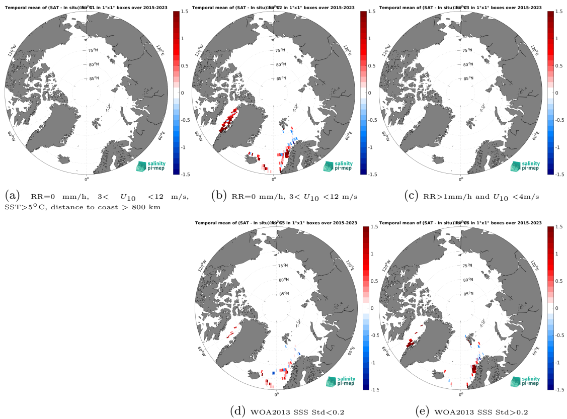
Figure 14: Temporal mean gridded over spatial boxes of size 1^\circ \times 1^\circ of \Delta SSS (SMAP SSS L2 v5.3 (RSS) - TSG (LEGOS-DM)) for 5 different subdatasets corresponding to:RR=0 mm/h, 3 < U_{10} < 12 m/s, SST>5°C, distance to coast > 800 km (a), RR=0 mm/h, 3 < U_{10} < 12 m/s (b), RR>1mm/h and U_{10} < 4 m/s (c), WOA2013 SSS Std<0.2 (d), WOA2013 SSS Std>0.2 (e).
