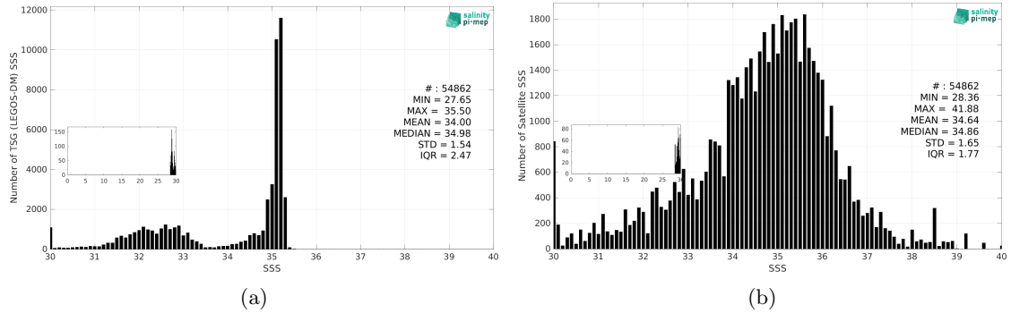
Figure 3: Histograms of SSS from TSG (LEGOS-DM) (a) and SMAP SSS L2 v5.3 (RSS) (b) considering all match-up pairs per bins of 0.1 over the Arctic Ocean Pi-MEP region and for the full satellite product period.
