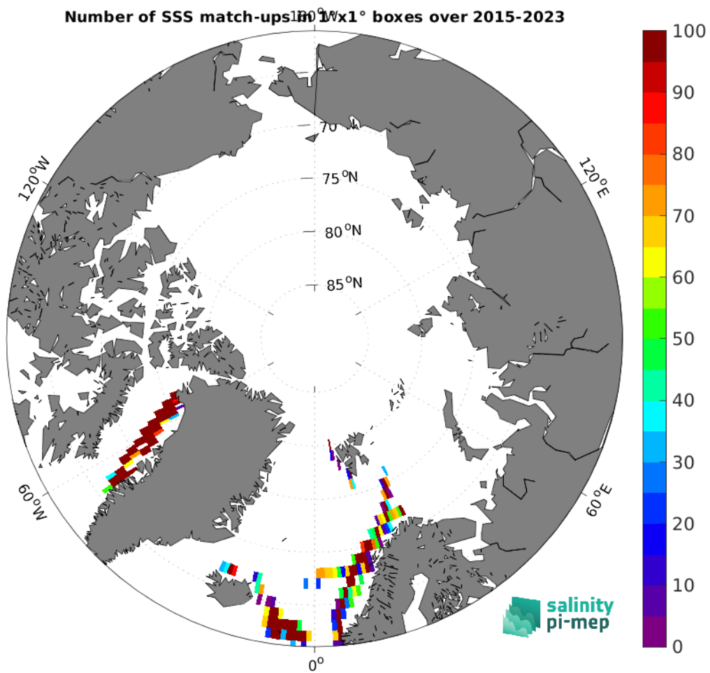
Figure 5: Number of SSS match-ups between TSG (LEGOS-DM) SSS and the SMAP SSS L2 v5.3 (RSS) SSS product for the Arctic Ocean Pi-MEP region over 1^\circ \times 1^\circ boxes and for the full satellite product period.
