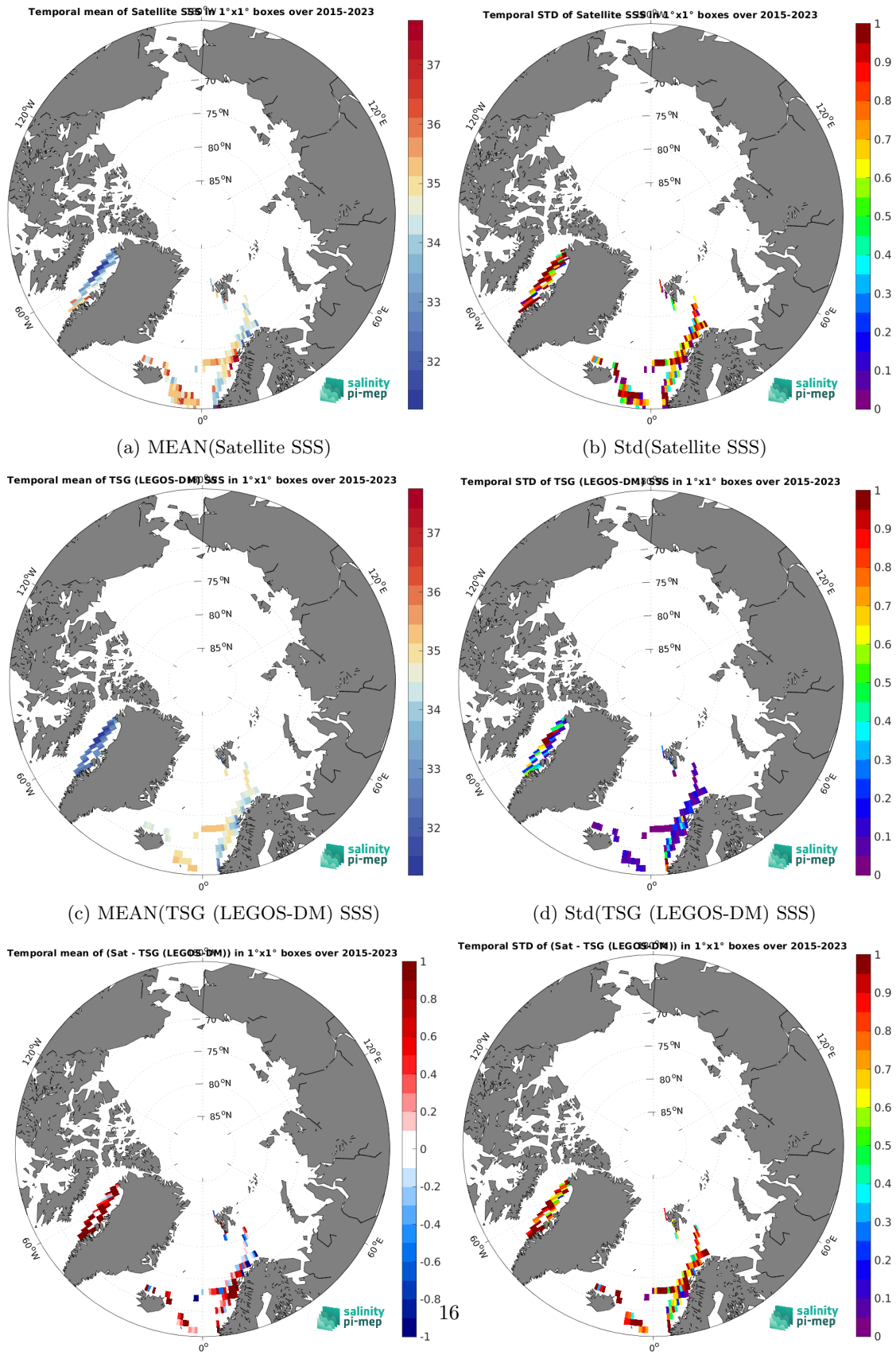
Figure 7: Temporal mean (left) and Std (right) of SSS from SMAP SSS L2 v5.3 (RSS) (top), TSG (LEGOS-DM) (middle), and of \Delta SSS (Satellite - TSG (LEGOS-DM)). Only match-up pairs are used to generate these maps.
