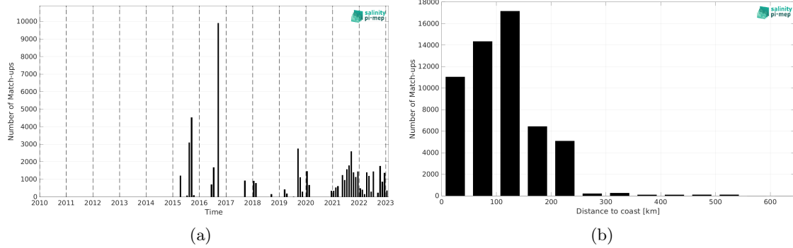
Figure 2: Number of match-ups between TSG (LEGOS-DM) and SMAP SSS L2 v5.3 (RSS) SSS as a function of time (a) and as function of the distance to coast (b) over the Arctic Ocean Pi-MEP region and for the full satellite product period.
