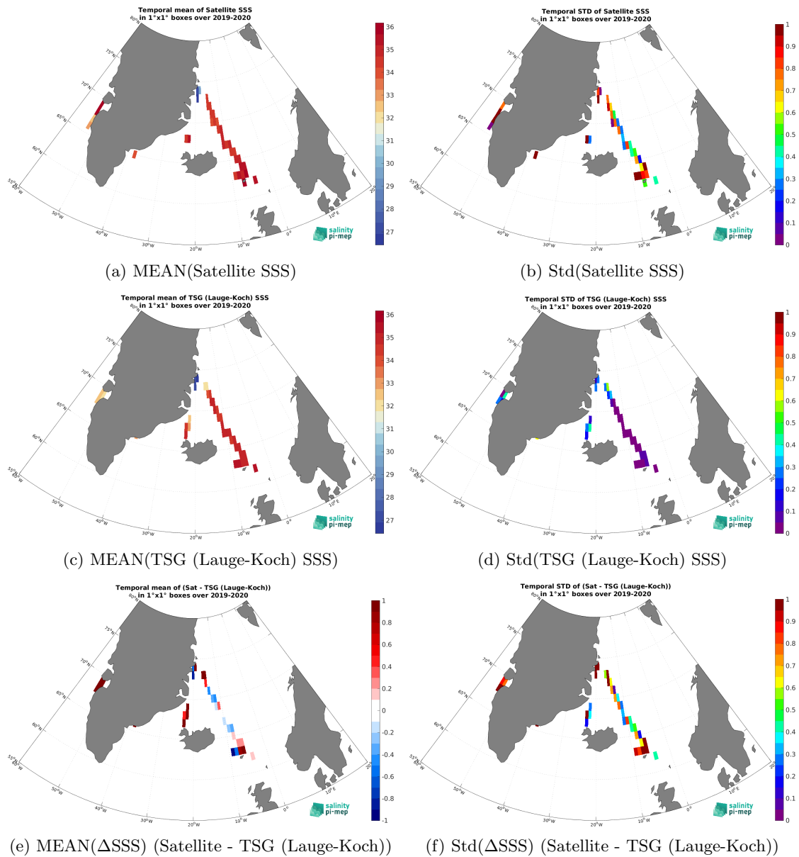
Figure 7: Temporal mean (left) and Std (right) of SSS from SMAP SSS L2 v5.3 (RSS) (top), TSG (Lauge-Koch) (middle), and of \Delta SSS (Satellite - TSG (Lauge-Koch)). Only match-up pairs are used to generate these maps.
