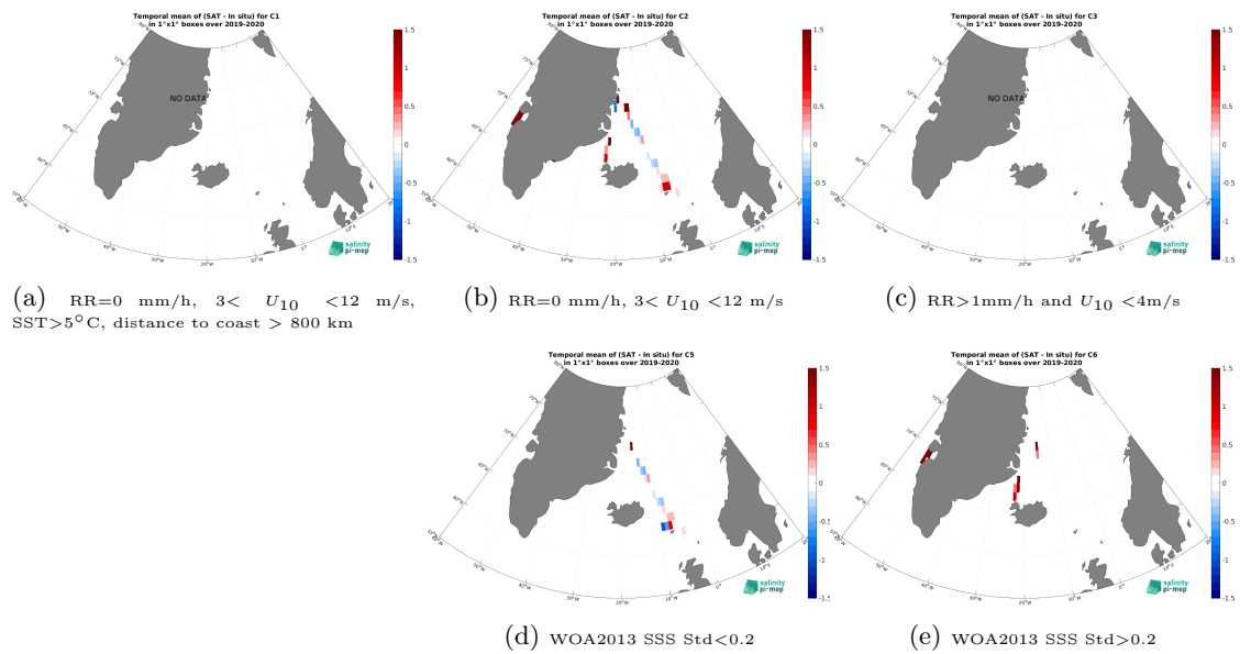
Figure 14: Temporal mean gridded over spatial boxes of size 1^\circ \times 1^\circ of \Delta SSS (SMAP SSS L2 v5.3 (RSS) - TSG (Lauge-Koch)) for 5 different subdatasets corresponding to:RR=0 mm/h, 3 < U_{10} < 12 m/s, SST > 5^\circ\text{C} , distance to coast > 800 km (a), RR=0 mm/h, 3 < U_{10} < 12 m/s (b), RR > 1 mm/h and U_{10} < 4 m/s (c), WOA2013 SSS Std < 0.2 (d), WOA2013 SSS Std > 0.2 (e).
