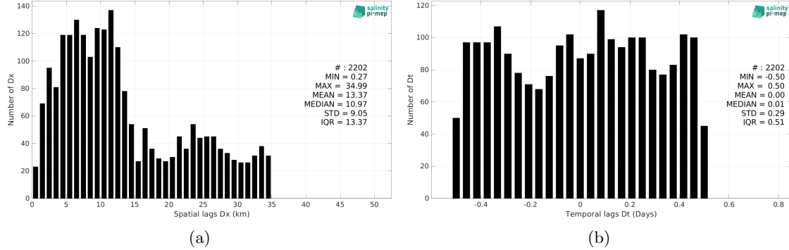
Figure 6: Histograms of the spatial (a) and temporal (b) lags between the location/time of the TSG (Lauge-Koch) measurement and the date of the corresponding SMAP SSS L2 v5.3 (RSS) SSS pixel.
