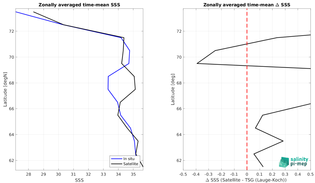
Figure 9: Left panel: Zonal mean SSS from SMAP SSS L2 v5.3 (RSS) satellite product (black) and from TSG (Lauge-Koch) (blue). Right panel: Zonal mean of \Delta SSS (Satellite - TSG (Lauge-Koch)) for all the collected Pi-MEP match-up pairs estimated over the full satellite product period.
