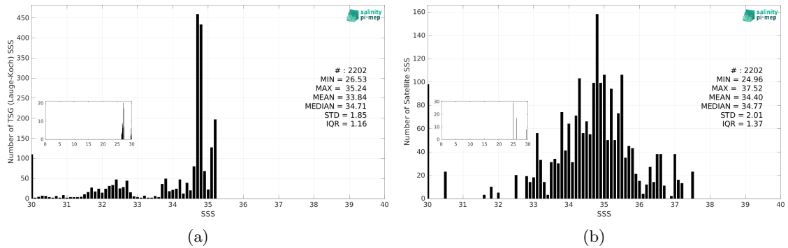
Figure 3: Histograms of SSS from TSG (Lauge-Koch) (a) and SMAP SSS L2 v5.3 (RSS) (b) considering all match-up pairs per bins of 0.1 over the Arctic Ocean Pi-MEP region and for the full satellite product period.
