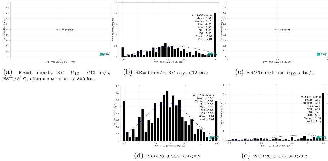
Figure 15: Normalized histogram of \Delta SSS (SMAP SSS L2 v5.3 (RSS) - TSG (Lauge-Koch)) for 5 different subdatasets corresponding to: RR=0 mm/h, 3 < U_{10} < 12 m/s, SST > 5°C, distance to coast > 800 km (a), RR=0 mm/h, 3 < U_{10} < 12 m/s (b), RR > 1mm/h and U_{10} < 4 m/s (c), WOA2013 SSS Std < 0.2 (d), WOA2013 SSS Std > 0.2 (e).
