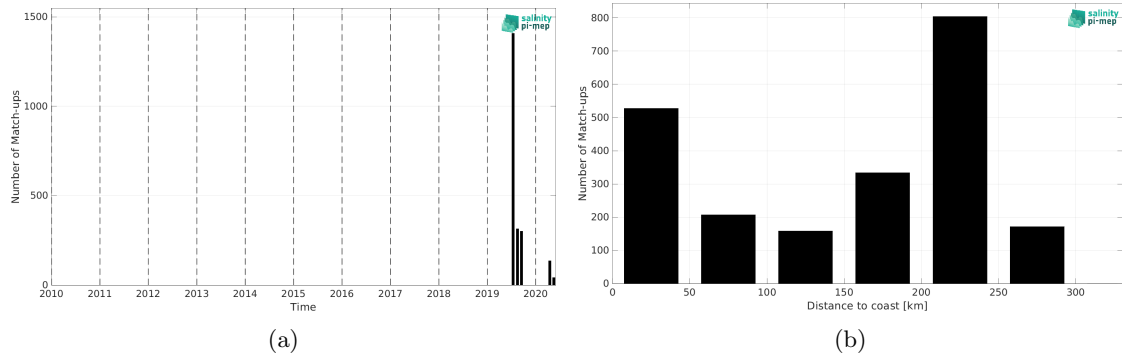
Figure 2: Number of match-ups between TSG (Lauge-Koch) and SMAP SSS L2 v5.3 (RSS) SSS as a function of time (a) and as function of the distance to coast (b) over the Arctic Ocean Pi-MEP region and for the full satellite product period.
