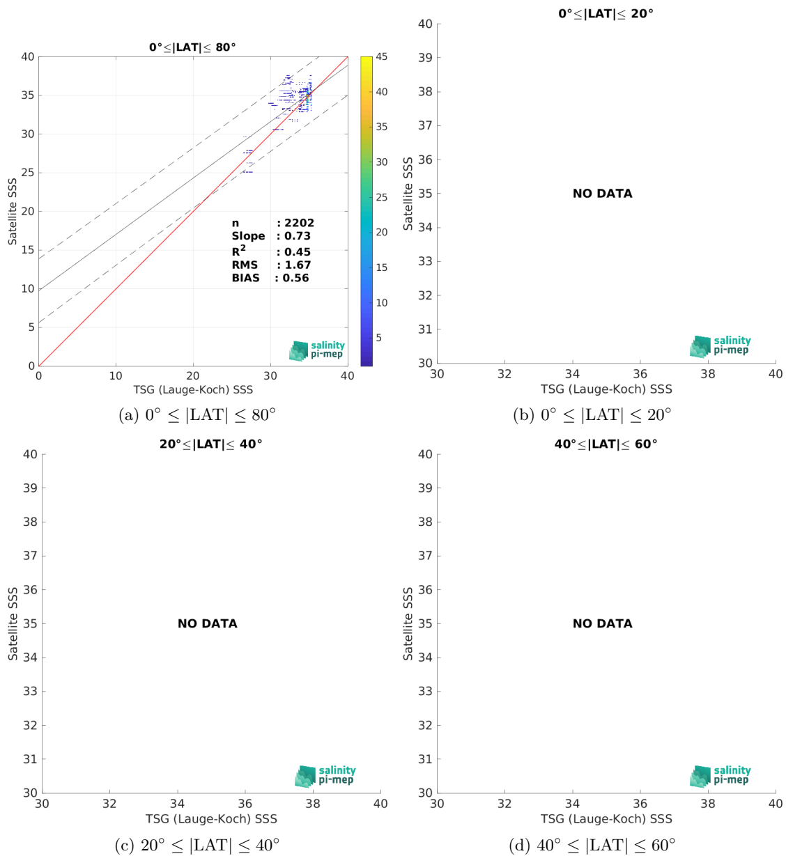
Figure 10: Contour maps of the concentration of SMAP SSS L2 v5.3 (RSS) SSS (y-axis) versus TSG (Lauge-Koch) SSS (x-axis) at match-up pairs for different latitude bands. For each plot, the red line shows x=y . The black thin and dashed lines indicate a linear fit through the data cloud and the \pm 95\% confidence levels, respectively. The number match-up pairs n , the slope and R^2 coefficient of the linear fit, the root mean square (RMS) and the mean bias between satellite and in situ data are indicated for each latitude band in each plots.
