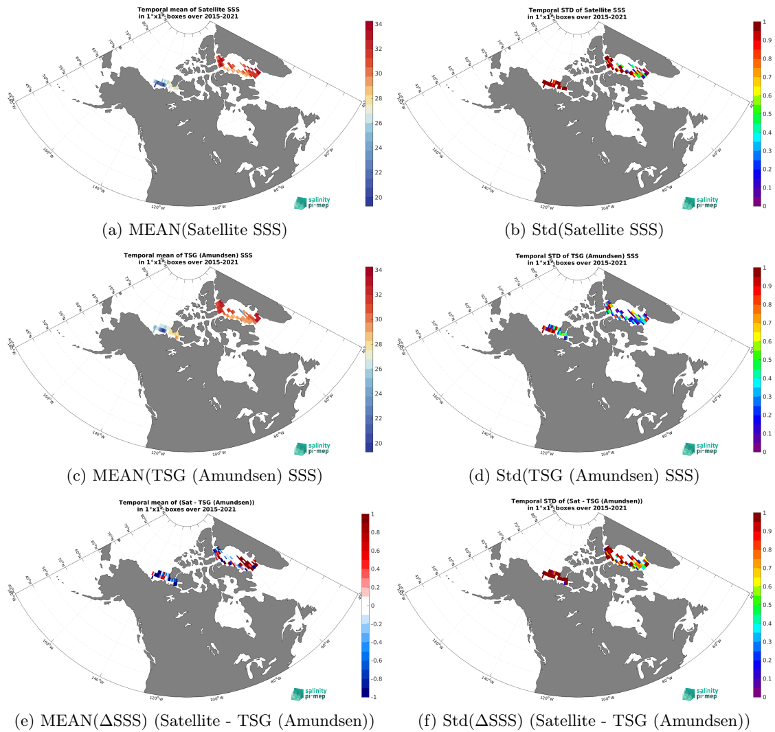
Figure 7: Temporal mean (left) and Std (right) of SSS from SMAP SSS L2 v5.3 (RSS) (top), TSG (Amundsen) (middle), and of \Delta SSS (Satellite - TSG (Amundsen)). Only match-up pairs are used to generate these maps.
