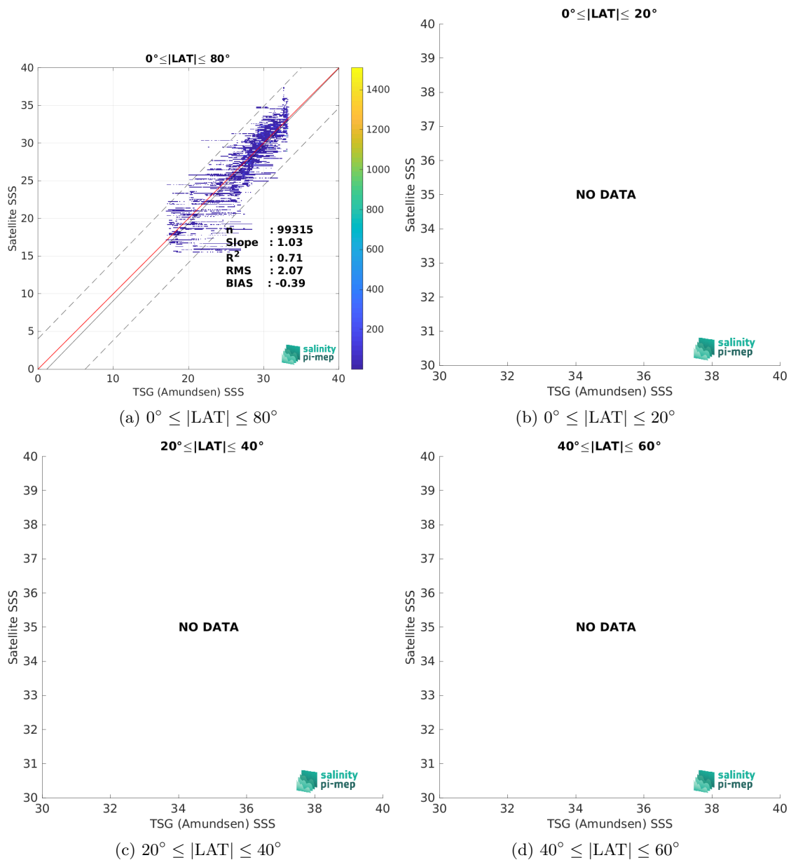
Figure 10: Contour maps of the concentration of SMAP SSS L2 v5.3 (RSS) SSS (y-axis) versus TSG (Amundsen) SSS (x-axis) at match-up pairs for different latitude bands. For each plot, the red line shows x=y . The black thin and dashed lines indicate a linear fit through the data cloud and the \pm 95\% confidence levels, respectively. The number match-up pairs n , the slope and R^2 coefficient of the linear fit, the root mean square (RMS) and the mean bias between satellite and in situ data are indicated for each latitude band in each plots.
