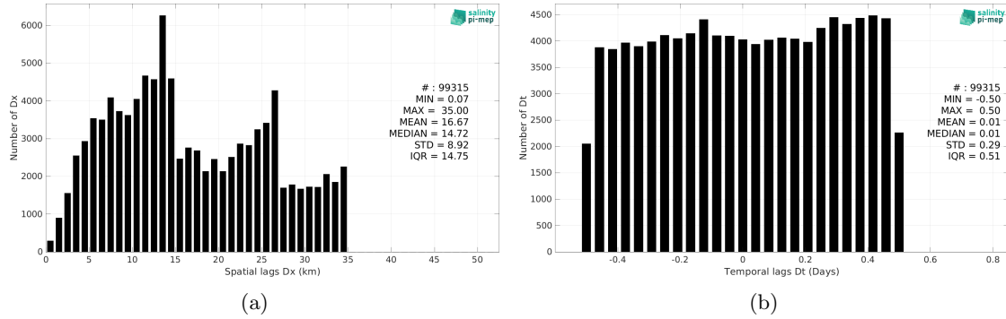
Figure 6: Histograms of the spatial (a) and temporal (b) lags between the location/time of the TSG (Amundsen) measurement and the date of the corresponding SMAP SSS L2 v5.3 (RSS) SSS pixel.
