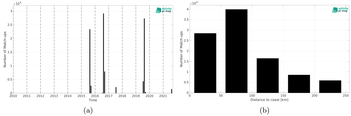
Figure 2: Number of match-ups between TSG (Amundsen) and SMAP SSS L2 v5.3 (RSS) SSS as a function of time (a) and as function of the distance to coast (b) over the Arctic Ocean Pi-MEP region and for the full satellite product period.
