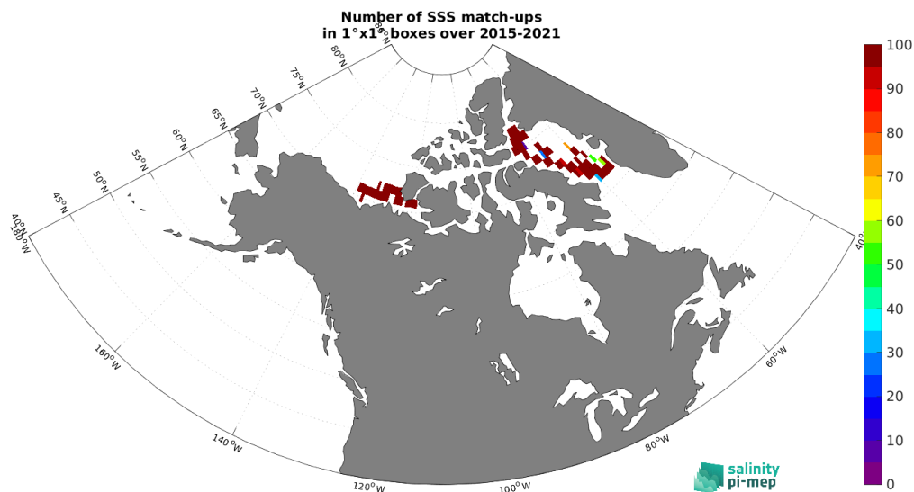
Figure 5: Number of SSS match-ups between TSG (Amundsen) SSS and the SMAP SSS L2 v5.3 (RSS) SSS product for the Arctic Ocean Pi-MEP region over 1^\circ \times 1^\circ boxes and for the full satellite product period.
