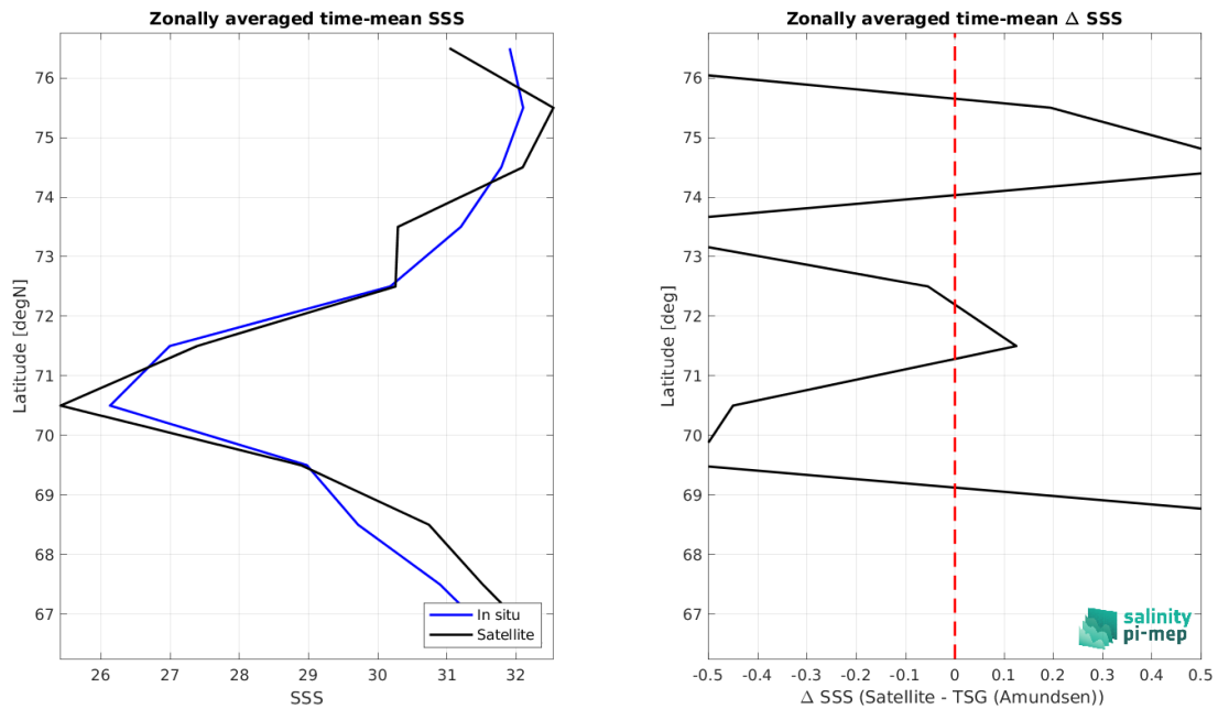
Figure 9: Left panel: Zonal mean SSS from SMAP SSS L2 v5.3 (RSS) satellite product (black) and from TSG (Amundsen) (blue). Right panel: Zonal mean of \Delta SSS (Satellite - TSG (Amundsen)) for all the collected Pi-MEP match-up pairs estimated over the full satellite product period.
