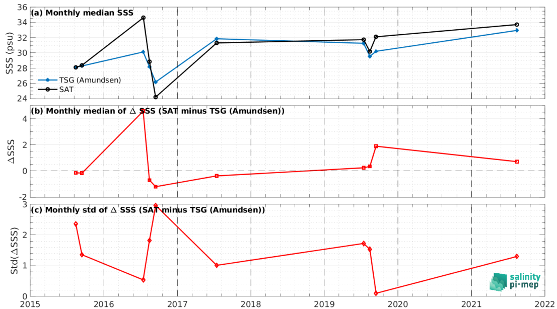
Figure 8: Time series of the monthly median SSS (top), median of \Delta SSS (Satellite - TSG (Amundsen)) and Std of \Delta SSS (Satellite - TSG (Amundsen)) over the Arctic Ocean Pi-MEP region considering all match-ups collected by the Pi-MEP.
