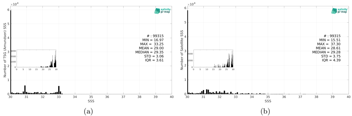
Figure 3: Histograms of SSS from TSG (Amundsen) (a) and SMAP SSS L2 v5.3 (RSS) (b) considering all match-up pairs per bins of 0.1 over the Arctic Ocean Pi-MEP region and for the full satellite product period.
