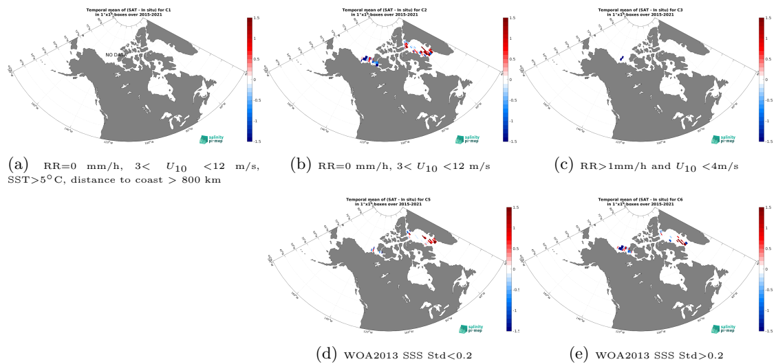
Figure 14: Temporal mean gridded over spatial boxes of size 1^\circ \times 1^\circ of \Delta SSS (SMAP SSS L2 v5.3 (RSS) - TSG (Amundsen)) for 5 different subdatasets corresponding to: RR=0 mm/h, 3 < U_{10} < 12 m/s, SST > 5°C, distance to coast > 800 km (a), RR=0 mm/h, 3 < U_{10} < 12 m/s (b), RR > 1mm/h and U_{10} < 4 m/s (c), WOA2013 SSS Std < 0.2 (d), WOA2013 SSS Std > 0.2 (e).
