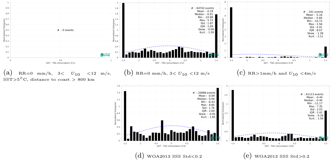
Figure 15: Normalized histogram of \Delta SSS (SMAP SSS L2 v5.3 (RSS) - TSG (Amundsen)) for 5 different subdatasets corresponding to: RR=0 mm/h, 3 < U_{10} < 12 m/s, SST > 5°C, distance to coast > 800 km (a), RR=0 mm/h, 3 < U_{10} < 12 m/s (b), RR > 1mm/h and U_{10} < 4 m/s (c), WOA2013 SSS Std < 0.2 (d), WOA2013 SSS Std > 0.2 (e).
